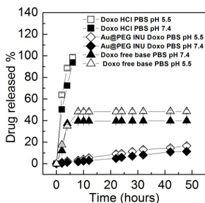
Fig. 2 Percentage doxorubicin release from Au@PEG-INU/Doxo NPs over time, when stored in PBS solutions at pH 7.4 and pH 5.5. Doxorubicin not associated with NPs, both in the free base (-NH 2 ) and hydrochloride forms, were used to determine normal doxorubicin release during dialysis.
