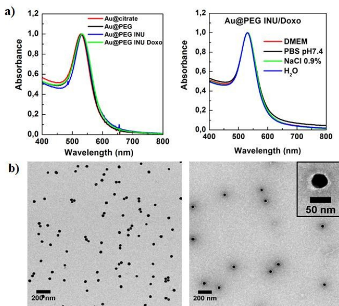
Fig. 1 a) UV-Vis spectra of Au@citrate, Au@PEG, Au@PEG-INU and Au@PEG-INU/Doxo nanoparticles, showing a sharp LSPR band (left) and the stability of Au@PEG-INU/Doxo in different media (right): Milli-Q water, NaCl 0.9%, cell medium (DMEM) and PBS pH 7.4. b) TEM images of Au@PEG-INU/Doxo without
