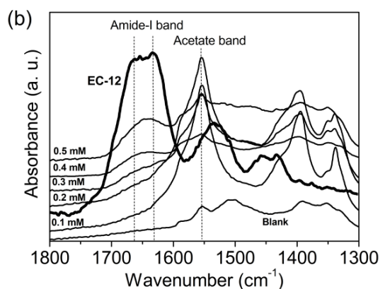
Fig. 9 (a) EC-12 concentration, [EC-12], in supernatants collected at different reaction time from reaction with initial [EC-12] of 0.1 mM, 0.2 mM, 0.3 mM and 0.5 mM from UV-vis measured (b) FTIR spectra of precipitates collected at 24 hours.
