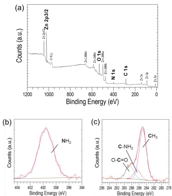
Fig. 10 (a) XPS survey spectrum recorded from an as-deposited precipitate collected at 24 hours ([EC-12] at 0.4 mM) and the corresponding high resolution core level spectra of (b) N 1s and (c) C 1s regions.
