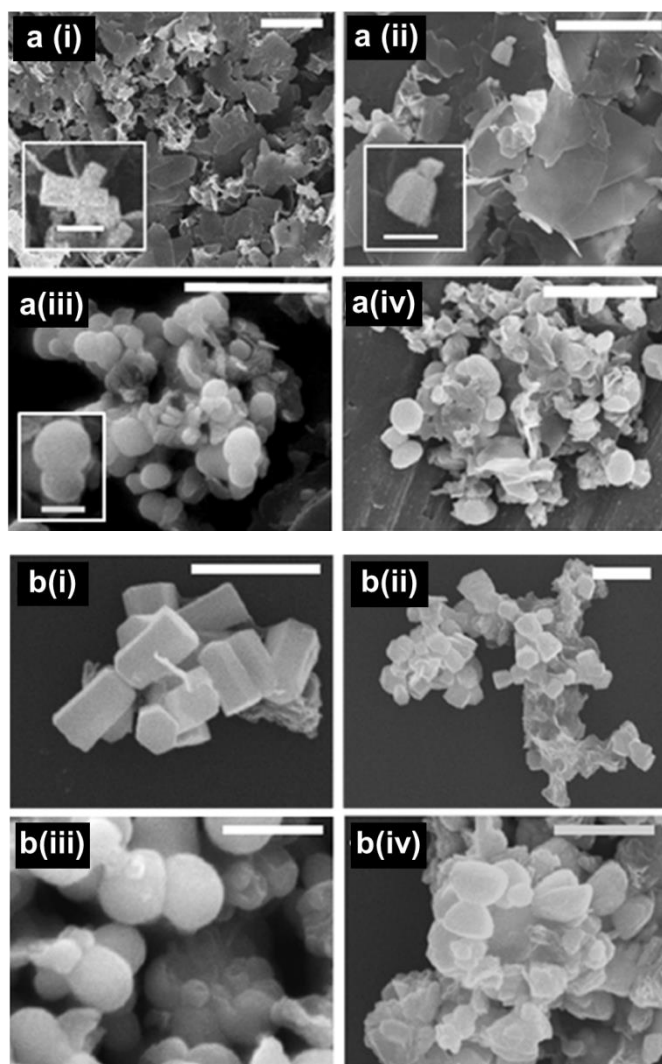
Fig. 12 SEM images of precipitates collected at (a) 24 hours (scale bars=5 \mu\text{m} , inset scale bars=1 \mu\text{m} ) and (b) 48 hours (scale bar=2 \mu\text{m} ). EC-12 concentration for SEM images are (i) 0.1 mM for (ii) 0.2 mM, (iii) 0.4 mM and (iv) 0.5 mM.
