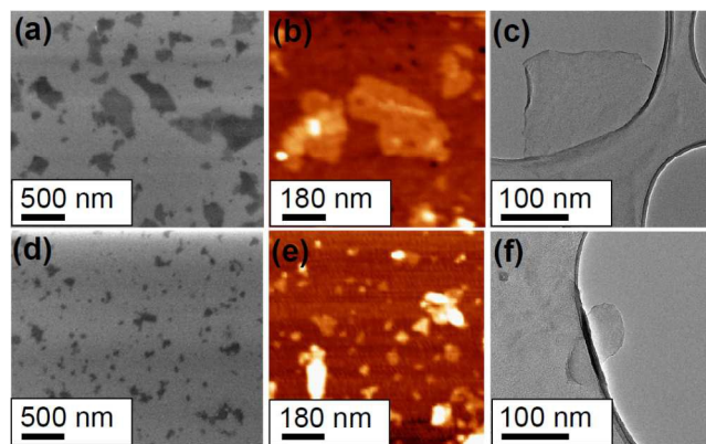
Figure 2. Panel (a) shows the SEM image of NGO with 277 nm in diameter and panel (b) shows an AFM image where the measured height of NGO was 4 layers. Panel (c) shows a TEM image of the Panels (d) to (f) show the same set of measurements for a second sample containing NGO nanoparticles with an average diameter of 89 nm and 6 layers.
