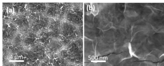
Fig. 2 (a and b) SEM images of \text{Co(OH)}_2 electrodeposited on to a Au electrode at a potential of -0.95 \text{ V} for 60 \text{ s} in a solution of 10 \text{ mM Co(NO}_3)_2 \cdot 6\text{H}_2\text{O} .
