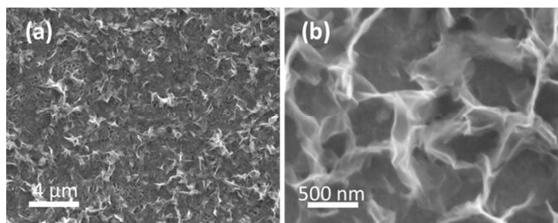
Fig. 6 SEM images of electrodeposited \text{Co(OH)}_2 on the Au electrode after the OER performed for 5 cycles under the conditions of Figure 5.
