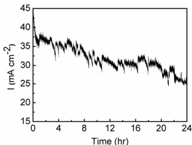
Fig. 9 Stability measurements of \text{Au}/\text{Co}(\text{OH})_2 held at 1.67 V for 24 hrs in 1 M NaOH.
