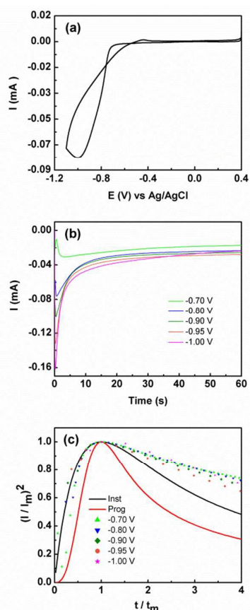
Fig. 1 (a) Cyclic voltammogram obtained at 50 \text{ mV s}^{-1} at a Au electrode in 10 \text{ mM Co(NO}_3)_2 \cdot 6\text{H}_2\text{O} solution (b) Current-time curves obtained at different applied potentials and (c) Non-dimensional plots of (I/I_m)^2 vs t/t_m for the electrodeposition of \text{Co(OH)}_2 . Overlaid are the theoretical curves calculated using Eqs. (3) and (4) for progressive (—) and instantaneous (---) nucleation and diffusion limited growth.
