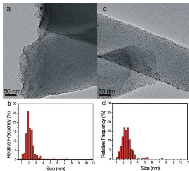
oxide. [22] Figure 1. a, c) TEM images and b, d) particle distribution obtained from TEM analysis of a,b) Pt/CFs, c, d) SnO 2 /Pt/CFs before cyclic voltammetry.
