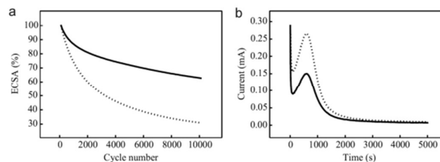
Figure 6. a) ECSA of Pt/CFs (dotted line) and SnO 2 /Pt/CFs (full line) calculated from cyclic voltammetry at 50 mV/s in a N 2 saturated 0.5 M H 2 SO 4 solution every 100 cycles performed at 100 mV/s. b) Oxidation/corrosion characteristics for Pt/CFs (dotted line) and SnO 2 /Pt/CFs (full line) at 1.4 V/RHE.
