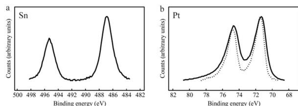
Figure 3. XPS spectra of SnO 2 /Pt/CFs (full line) and Pt/CFs (dotted line). High resolution scans across a) the Sn 3d and b) Pt 4f edges, respectively.
