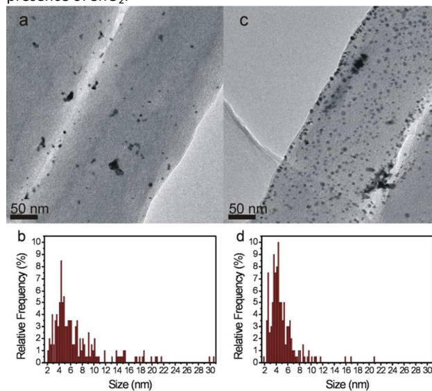
Figure 7. TEM images a,c) and b,d) particle distribution from TEM analysis of a,b) Pt-CFs and c,d) SnO 2 -Pt-CFs after 10,000 potential cycles.
