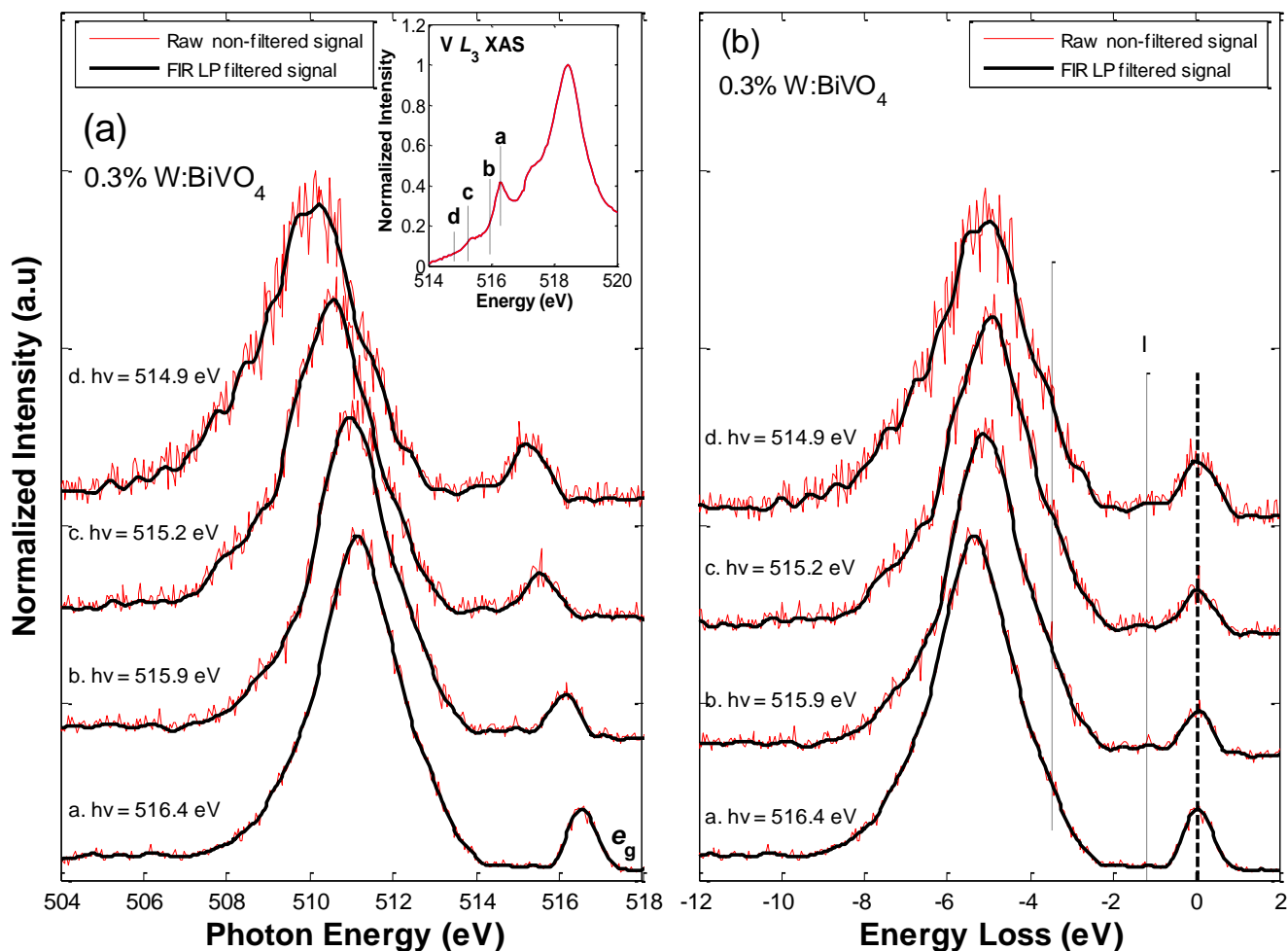
Figure 6 – (a) V L_3 -edge RIXS spectra for 0.3% W:BiVO 4 . The spectra have been vertically offset for clarity. The excitation energy for each spectrum is indicated on the plot. (b) The V L_3 -edge RIXS spectra for 0.3% W:BiVO 4 on an energy loss (charge transfer) scale. The raw, non-filtered, signals are shown in red and the FIR LP filtered signals are shown in black.
