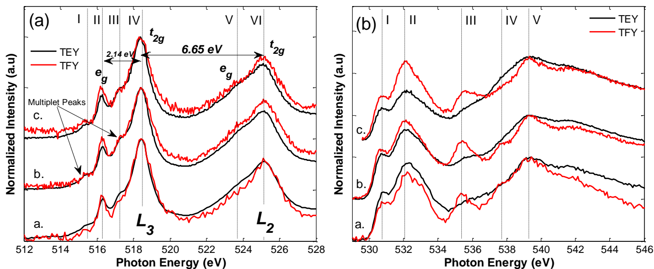
Figure 1 – (a) V L_{3,2} XAS in the TEY (black) and TFY (red) modes for a. BiVO_4 , b. 0.6% Mo: BiVO_4 and c. 0.3% W: BiVO_4 . (b) - O K -edge XAS in the TEY (black) and TFY (red) modes for a. BiVO_4 , b. 0.6% Mo: BiVO_4 and c. 0.3% W: BiVO_4 . Spectra are vertically offset for clarity.
