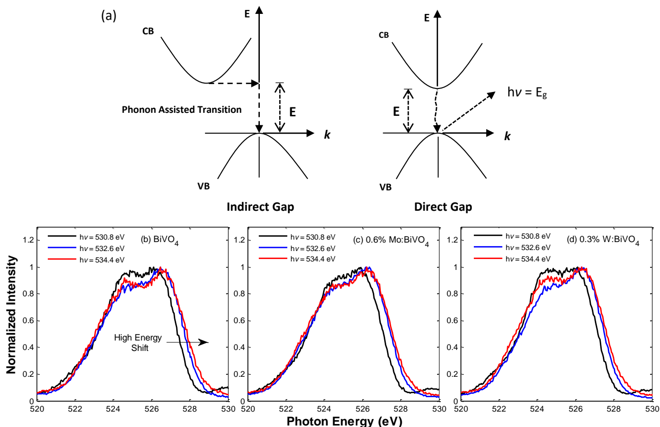
Figure 4 – (a) The indirect (left) and direct (right) electronic band gaps. (b)-(d) Plots of O K -edge XES spectra collected at three energies near the onset of the O K -edge XAS. The high energy shift of VB onset with increasing photon energy verifies that the band gap of the material is indirect and unaffected by Mo or W doping.
