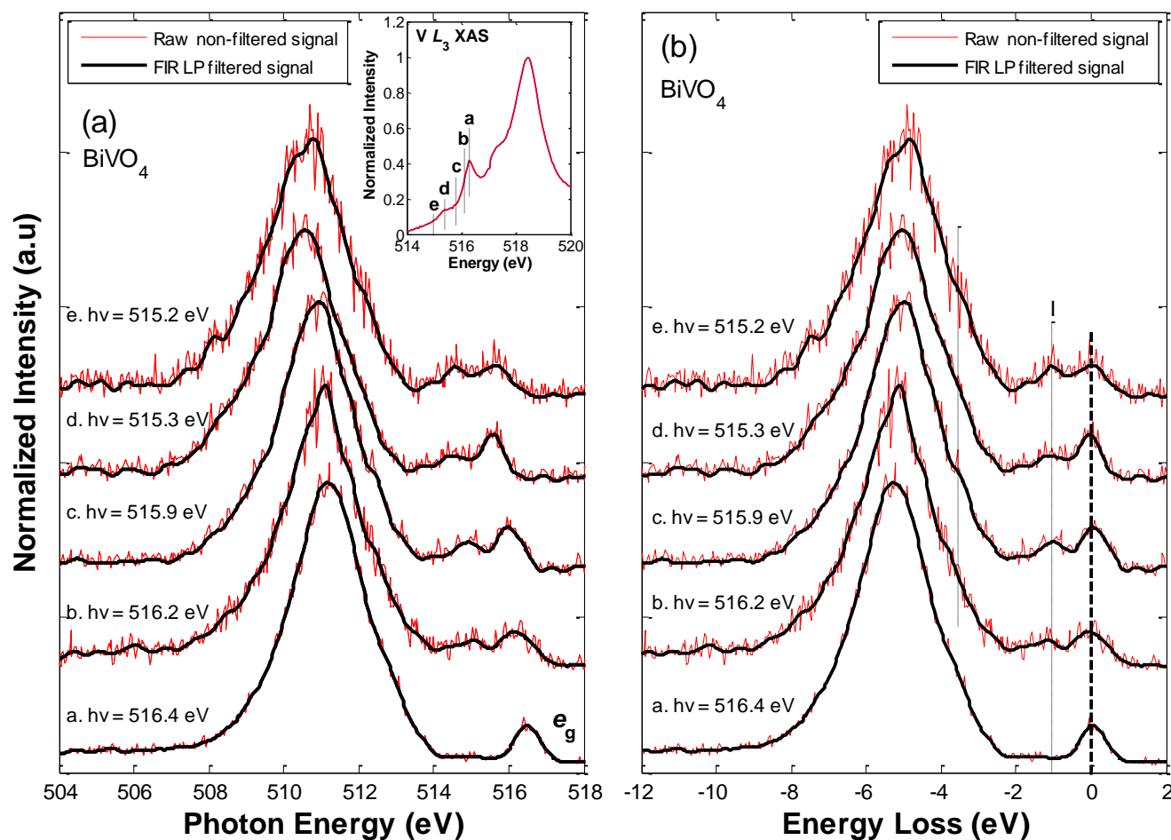
Figure 5 – (a) V L_3 -edge RIXS spectra for \text{BiVO}_4 . The spectra have been vertically offset for clarity. The excitation energy for each spectrum is indicated on the plot. (b) The V L_3 -edge RIXS spectra for \text{BiVO}_4 on an energy loss (charge transfer) scale. In all plots, the raw, non-filtered, signals are shown in red and the FIR LP filtered signals are shown in black.
