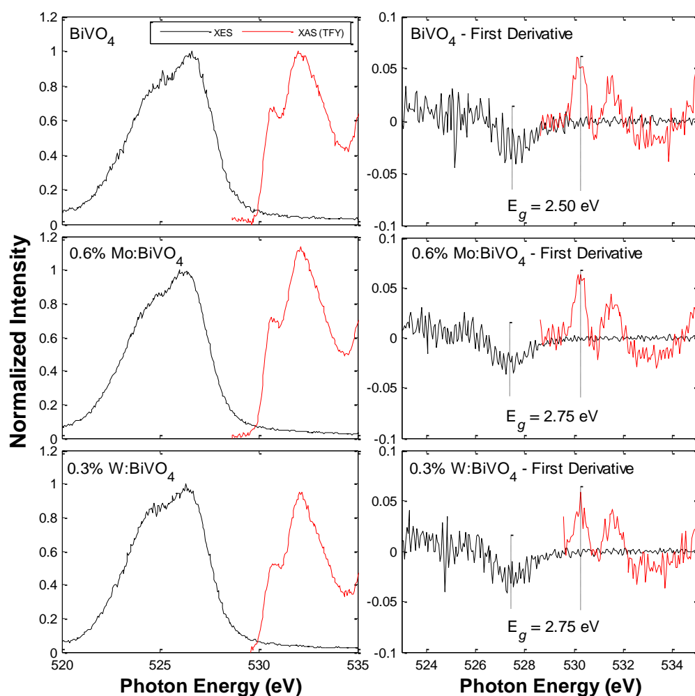
Figure 3 – Left Panels; O K -edge XES (black) and O K -edge XAS TFY (red) for \text{BiVO}_4 , 0.6% Mo: \text{BiVO}_4 and 0.3% W: \text{BiVO}_4 . The XES spectra were taken at h\nu = 550 eV. Right Panels; First derivative plots for the plots at left.
