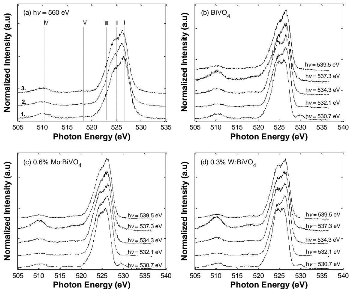
Figure 2 – (a) O K XES spectra for 1. BiVO 4 , 2. 0.6% Mo:BiVO 4 and 3. 0.3% W:BiVO 4 collected with an incident photon energy of 560 eV. (b) BiVO 4 O K-edge RXES. (c) 0.6% Mo:BiVO 4 O K-edge RXES. (d) 0.3% W:BiVO 4 O K-edge RXES.
