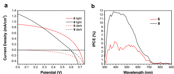
Fig. 3 (a) J - V curves for champion devices, dashed and (b) IPCE spectra for devices based on active layers of 6 or 8 and PC 71 BM.
