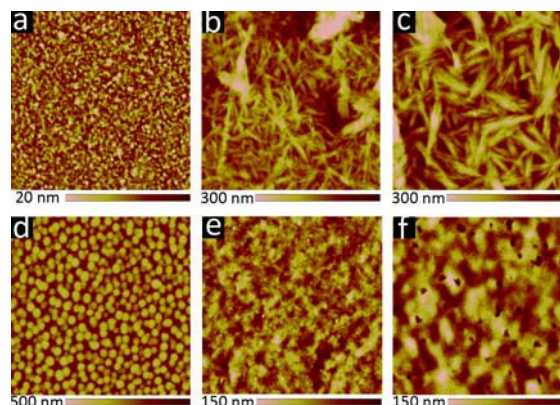
Fig. 4 10 \times 10 \mu\text{m} AFM images of active layer blends cast from 20 mg/mL solutions; (a-c) 6 :PC 71 BM active layers with (a) 0%, (b) 1%, (c) 3% DIO (v/v); (d-f) 8 :PC 71 BM active layers with (d) 0%, (e) 1%, (f) 3% DIO (v/v).
