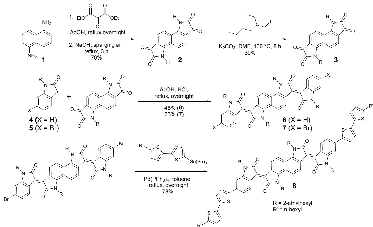
Scheme 1 Synthesis of bisisoindigo ( 6 ) and bis(5'-hexyl-2,2'-bithienyl)-bisisoindigo ( 8 )
