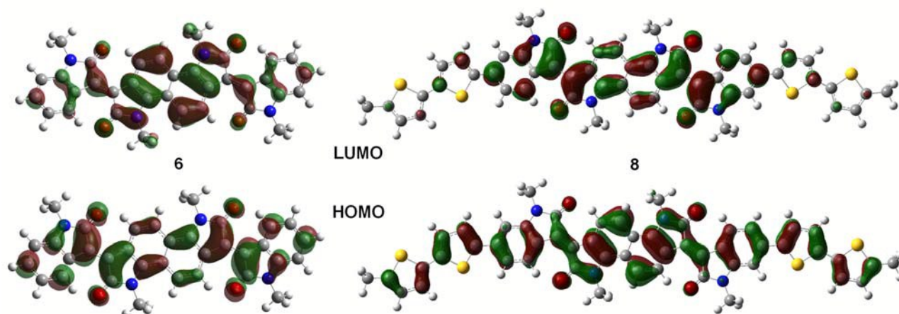
Fig. 1 Frontier molecular orbitals of 6 and 8 .
