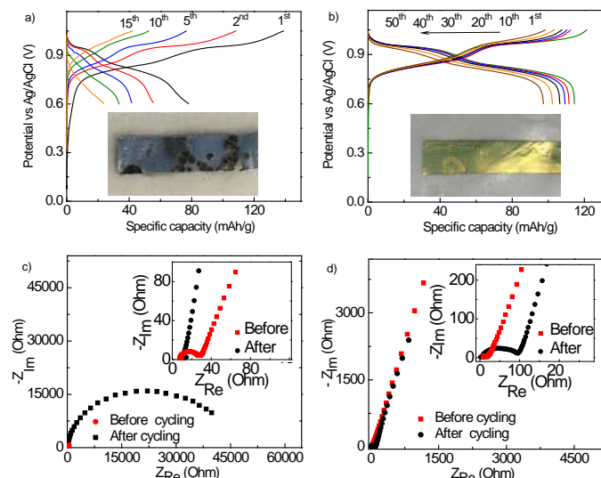
Figure 2: Electrochemical characterization of \text{LiMn}_2\text{O}_4 electrodes on un-treated aluminium and CCC aluminium foil as current collectors. (a) Charge–discharge voltage curve of different cycles in 2.5 M \text{Li}_2\text{SO}_4 electrolyte (pH = 7) for \text{LiMn}_2\text{O}_4 electrode on un-treated aluminium foil. Inset shows the photograph of the backside of un-treated aluminium foil current collector after 15 cycles. (b) \text{LiMn}_2\text{O}_4 electrode on CCC aluminium foil. Inset shows the photograph of the backside of CCC aluminium foil current collector after 50 cycles. The golden color is typical color of CCC coating. Impedance spectra for (c) un-treated aluminium foil and (d) CCC aluminium foil before and after cycling. In both (c) and (d), insets show the magnified high frequency region.
