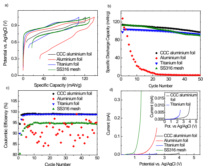
Figure 4: Comparison of electrochemical performance of LiMn 2 O 4 electrodes fabricated on different current collectors in 2.5 M Li 2 SO 4 electrolyte (pH = 7): (a) 1 st galvanostatic charge-discharge voltage profiles, (b) stability of specific discharge capacity, (c) Coulombic efficiency, and (d) linear scan voltammetry for different current collectors in 2.5 M Li 2 SO 4 (pH = 7) at a scan rate of 1 mV/s.
