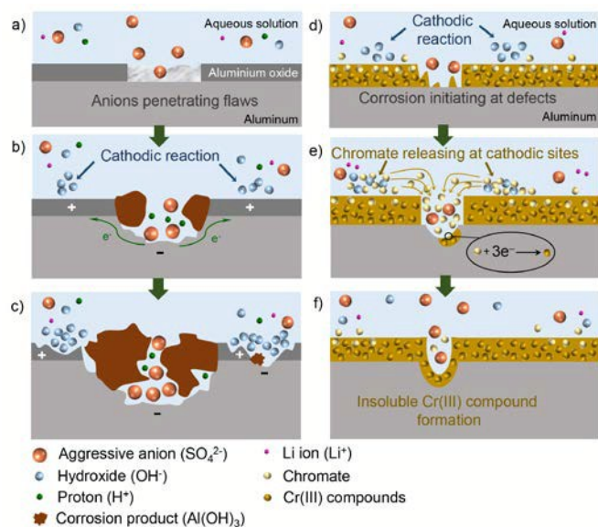
Figure 3: Schematics of the corrosion behavior of un-treated (a–c) and CCC (d–f) aluminium in aqueous electrolytes. (a) Pitting initiation, (b) propagation of the pit and formation of \text{Al}(\text{OH})_3 as the corrosion product, (c) local increase of pH around the pit and formation of new corrosion sites. (d) Initiation of a corrosion site at an un-protected site on the surface, (e) chromate released to the solution as a result of pH increase around the corrosion site followed by chromate reduction to form insoluble Cr(III) compounds, and (f) passivation of the corrosion site as insoluble Cr(III) formed.
