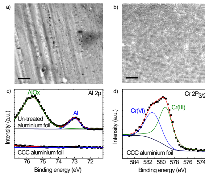
Figure 1. Characterization of CCC aluminium foil. SEM image of the surface obtained from aluminium foil (a) before and (b) after coating (scale bar: 10 \mu\text{m} ). (c) XPS Al 2p spectra of aluminium foil before and after coating; and (d) XPS Cr 2p 3/2 for CCC aluminium foil.
