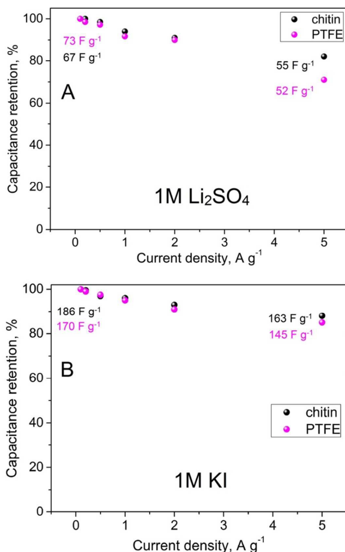
Fig. 6. Capacitance retention and values of capacitance versus current density in (A) 1M Li 2 SO 4 (B) 1M KI.
