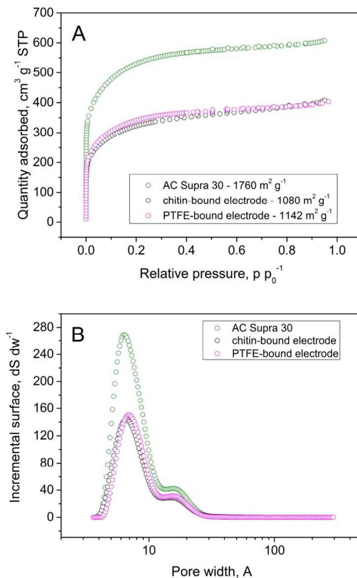
Fig. 3. (A) Nitrogen sorption isotherms of Supra 30, PTFE-bound electrode, and chitin-bound electrode (B) pore size distribution of materials estimated by 2D-NDLFT
