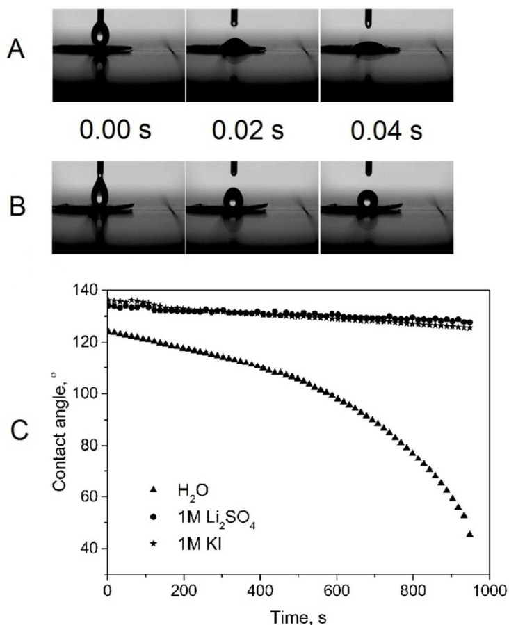
Fig. 2. Behaviour of a droplet of deionized water on (A) chitin-bound electrode (B) PTFE-bound electrode (C) contact angle measurements of PTFE-bound electrode using deionised water, 1M Li 2 SO 4 , 1M KI
