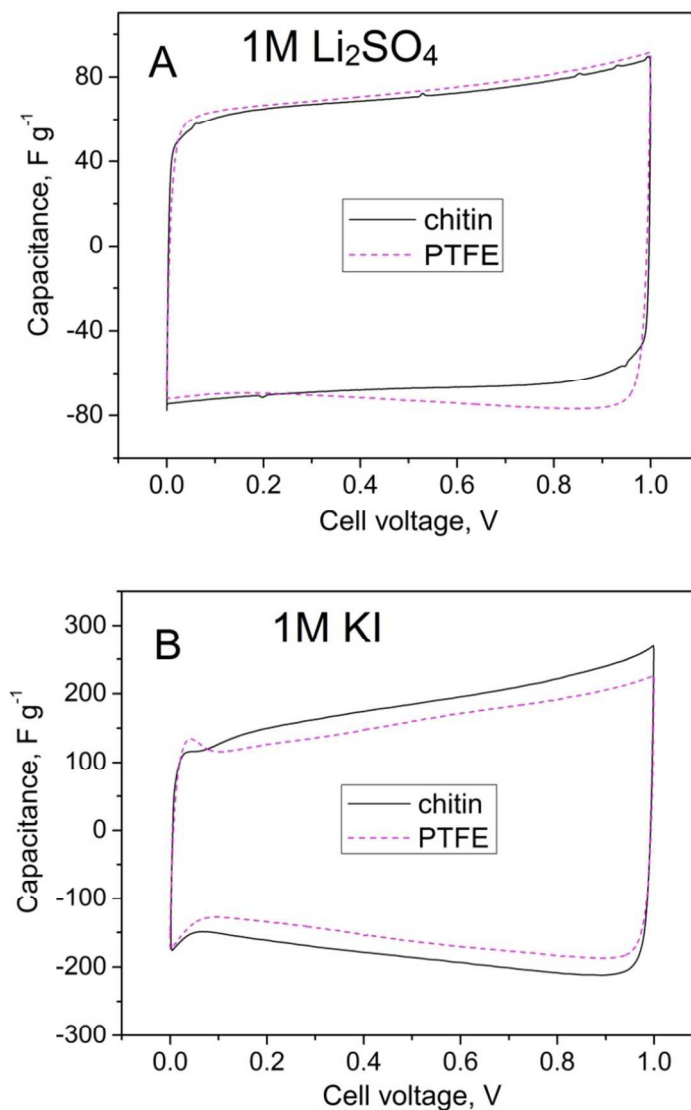
Fig. 4. Cyclic voltammograms (10 mV s -1 ) of capacitor based on chitin-bound electrode compared to PTFE-bound electrode in (A) 1M Li 2 SO 4 (B) 1M KI
