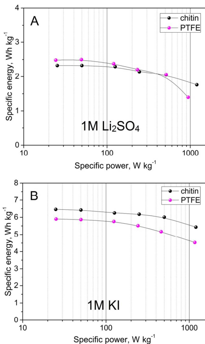
Fig. 11. Energy density vs. power density of capacitor with chitin- and PTFE-bound electrodes in (A) 1M Li 2 SO 4 (B) 1M KI
