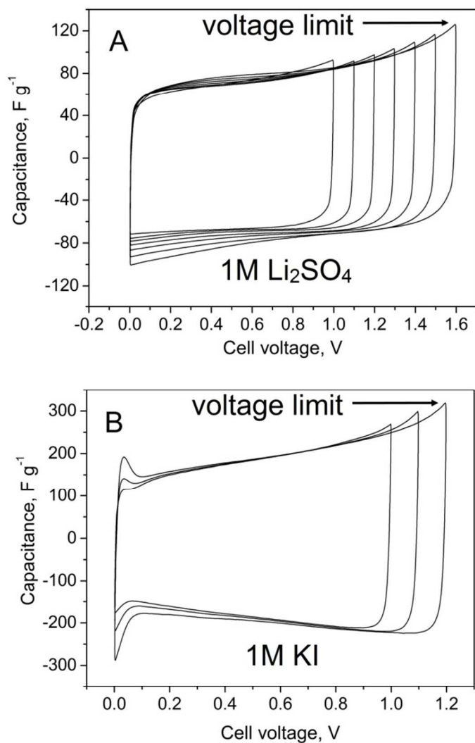
Fig. 5. Cyclic voltammograms ( 10 \text{ mV s}^{-1} ) of EDLC based on chitin-bound electrodes (A) at the cut-off voltage of 1.0 - 1.6 V in 1M Li 2 SO 4 (B) at the cut-off voltage of 1.0 - 1.2 V in 1M KI
