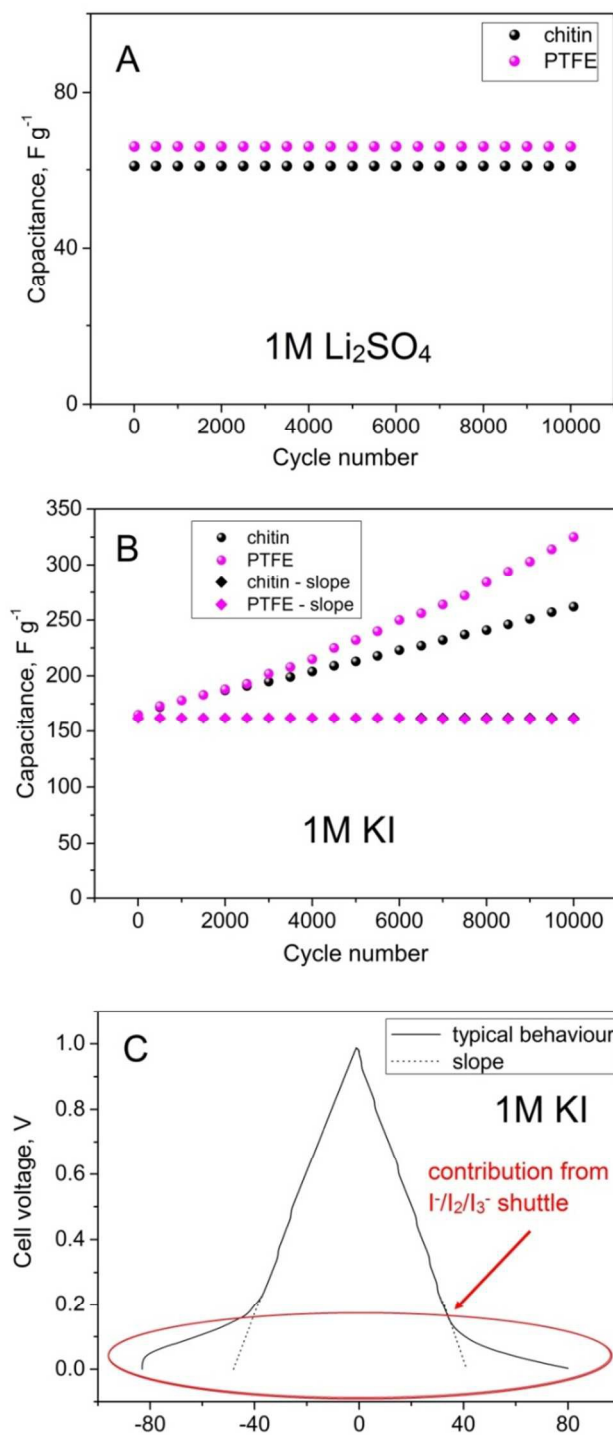
Fig. 7. Cycle life of chitin- and PTFE-bound electrodes at 2 A g^{-1} in (A) 1M Li_2SO_4 (B) 1M KI (C) Constant current charging/discharging of PTFE-bound electrode at 2 A g^{-1} in 1M KI .
