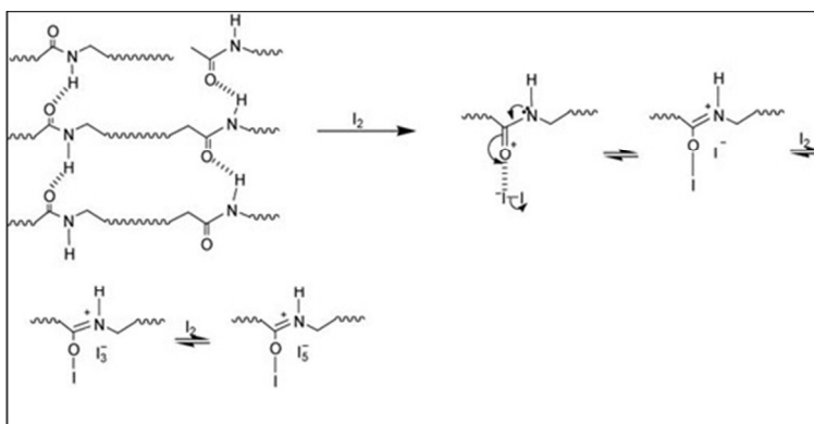
Fig. 8. A representative scheme of chitin-iodine complex formation. 39
