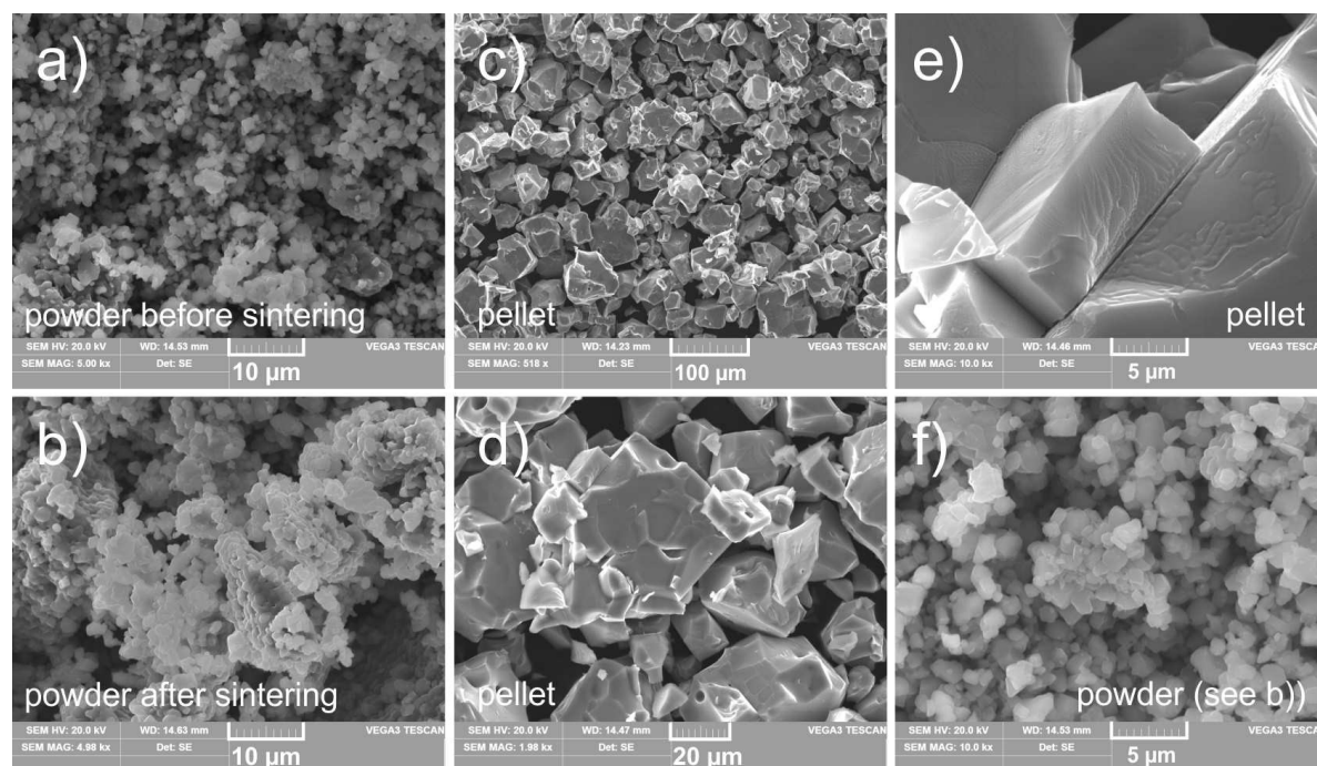
Fig. 2: SEM images of the powder sample (a), (b) and (f)) as well as the pellet investigated (c), (d) and (e), just differing by the magnification). Except the one shown in a) all images were taken after the sintering step at 1223 K and the conductivity measurements. (b) and (f) refer to the same sample, the images differ in magnification.
