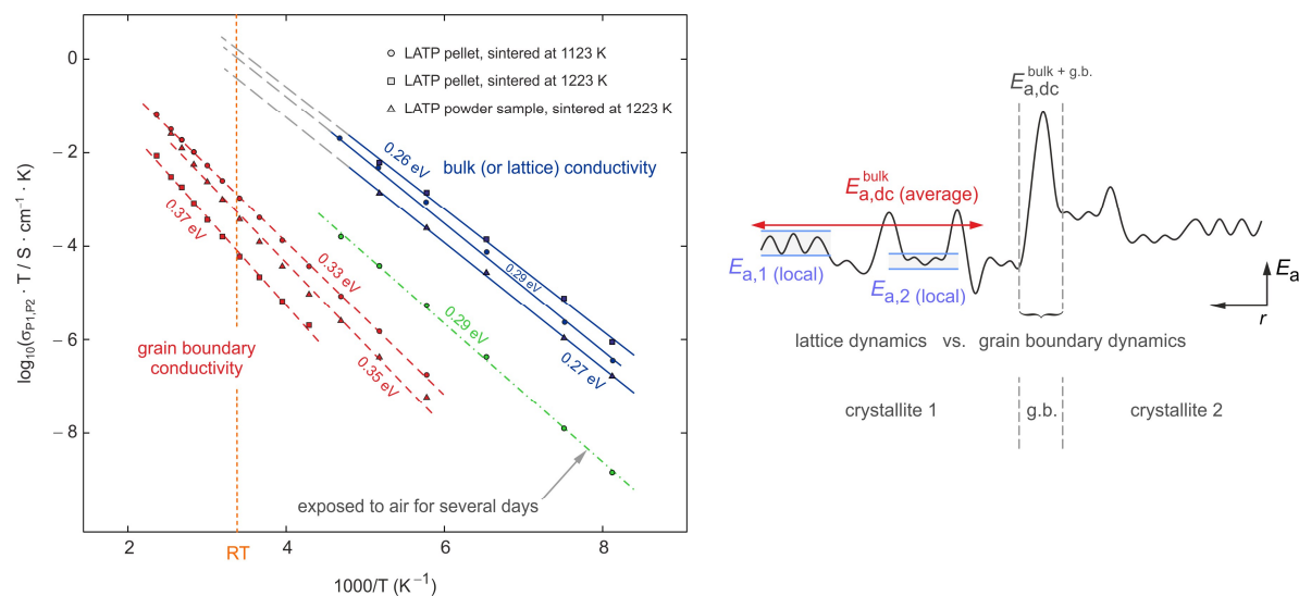
Fig. 6: Left: Arrhenius plot of the g.b. and bulk ion conductivities of the \text{Li}_{1.5}\text{Al}_{0.5}\text{Ti}_{1.5}(\text{PO}_4)_3 samples studied. The data were deduced from the conductivity isotherms partly shown in Fig. 3 a) and b). The dashed and solid lines represent fits according to an Arrhenius law: \sigma T \propto \exp(-E_a/(k_B T)) , k_B denotes Boltzmann's constant. The activation energies obtained are indicated. At ambient temperature, see vertical line, a DC bulk conductivity of ca. 3.4 mS/cm is obtained after extrapolation. Right: Schematic illustration of a heterogeneous potential landscape. Depending on the length scale, the method chosen to study ion dynamics is either sensitive to long-range ion dynamics or to local ionic jump processes. While atomic-scale methods, such as Li NMR, are also sensitive to individual ion hopping with low energy barriers, dc conductivity measurements probe an average value that characterises long-range, i.e. , through-going, ion dynamics.
