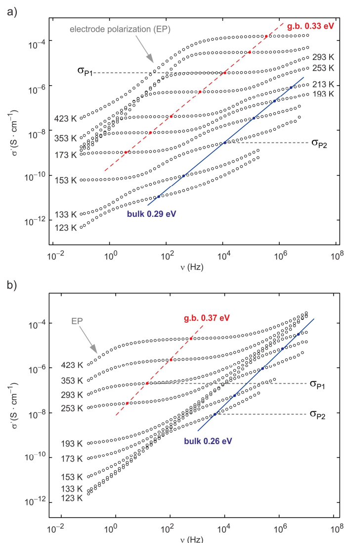
Fig. 4: a) Conductivity isotherms of a sintered LATP pellet ( \text{Li}_{1.5}\text{Al}_{0.5}\text{Ti}_{1.5}(\text{PO}_4)_3 ) with a thickness of 4 mm. The pellet was sintered at 1123 K. In b) the corresponding isotherms of the same sample are shown after sintering at 1223 K. The conductivity spectra exhibit two separate plateaus reflecting grain boundary (g.b.) and bulk ion conductivities: \sigma_{P1} and \sigma_{P2} . EP denotes electrode polarisation because of the ion blocking electrodes used to record the data.
