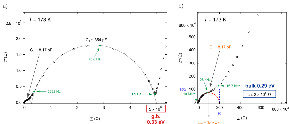
Fig. 3: a) Complex plane plot, i.e. , AC-impedance diagram, of the \text{Li}_{1.5}\text{Al}_{0.5}\text{Ti}_{1.5}(\text{PO}_4)_3 pellet sintered at 1123 K. In b) a magnification of the high-frequency region is shown. The highest frequency used to measure the data was 10 MHz. The solid line shows a fit using individual resistances and CPEs connected in parallel; see text for further discussion.
