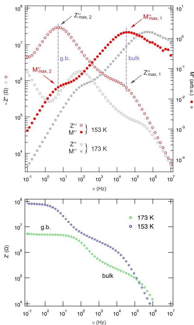
Fig. 5: Top: Change of the imaginary part of the complex impedance of \text{Li}_{1.5}\text{Al}_{0.5}\text{Ti}_{1.5}(\text{PO}_4)_3 with frequency. The curves exhibit two maxima that are ascribed to bulk and g.b. response. The maximum associated with lattice ion dynamics is more pronounced in the modulus representation, see right axis. Besides the data recorded at 153 K, the two spectra acquired at 173 K are also shown. Bottom: Variation of the real part of the complex impedance with frequency. As in the case of \sigma'(\nu) the bulk regions appear at higher frequencies.
