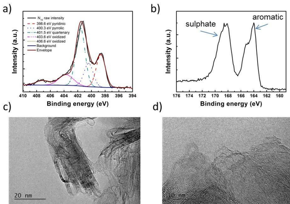
Figure 3: a) High resolution N1s XPS spectrum with the peaks deconvoluted into pyridinic, pyrrolic, quaternary and oxidised nitrogen species. b) High resolution S2p XPS spectrum showing peaks that can be assigned to aromatic sulphur and sulphate species respectively. c) and d) TEM images of ODAN catalyst.
