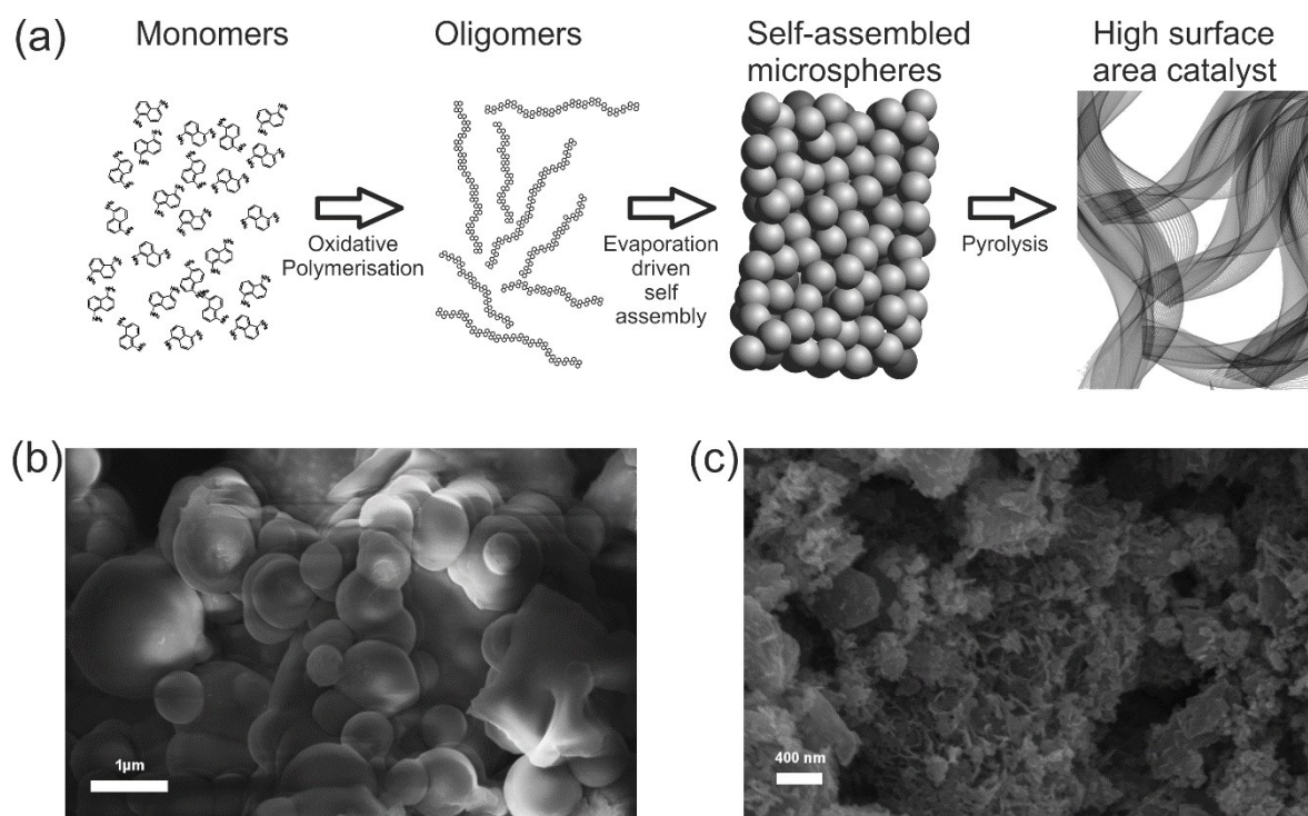
Figure 1: a) Schematic, depicting the synthesis procedure of the catalyst b) Scanning Electron Microscopy image of polymerized 1,5-Diaminonaphthalene as precursor for the ODAN catalyst c) Scanning Electron Microscopy image of ODAN catalyst material after heat treatment at 1000 °C for 2h.
