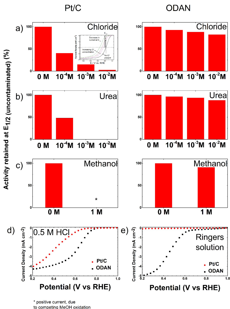
Figure 6: Bar plot showing the performance at the respective half wave potential of the RDE measurement, comparing a Pt/C catalyst to ODAN Rotating speed: 1600 rpm, 30s hold, 30 mV step potential, catalyst loading: ODAN: 750 \mu\text{g}/\text{cm}^2 , Pt/C: 30 \mu\text{g}_{\text{Pt}}/\text{cm}^2 , \text{O}_2 -saturated at 1 atm before and after adding a) \text{Cl}^- to 0.5M \text{H}_2\text{SO}_4 b) Urea to 0.5M \text{H}_2\text{SO}_4 and c) methanol to 0.1M NaOH to obtain the respective concentrations. The complete measurements are shown in the Supporting Information Figure S13 and S14 and S15. d) 0.5M HCl e) Ringers Solution
