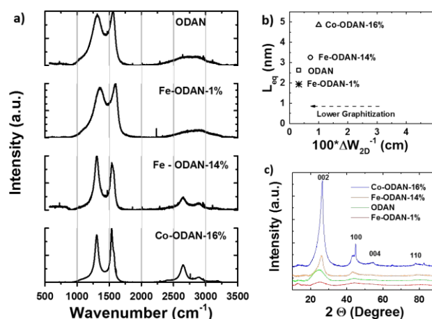
Figure 2: a) Raman spectra of ODAN, Fe-ODAN-1%, Fe-ODAN-14% and Co-ODAN-16%. b) Plot of the average continuous graphene layer length ( L_{eq} ) of selected catalysts as a function of the crystalline quality at curvature [ (\Delta W_{2D})^{-1} ] for a comparative analysis of the degree of graphitization. c) XRD spectra of ODAN, Fe-ODAN-14%, Fe-ODAN-1% and Co-ODAN-16%. The shape of the peak at ~26° shows that the degree of graphitization is reduced from Co-ODAN-16% over Fe-ODAN-14% to ODAN. Also seen in the peak at ~44°.
