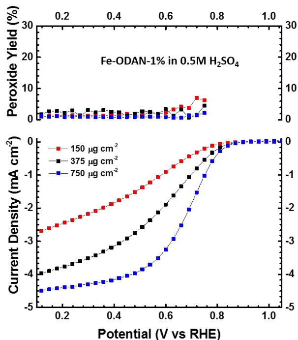
Figure 5: Steady-state RRDE measurement in 0.5M H 2 SO 4 at different catalyst loadings. Rotating speed: 1600 rpm, 30s hold, 30 mV step potential, O 2 -saturated at 1 atm.
