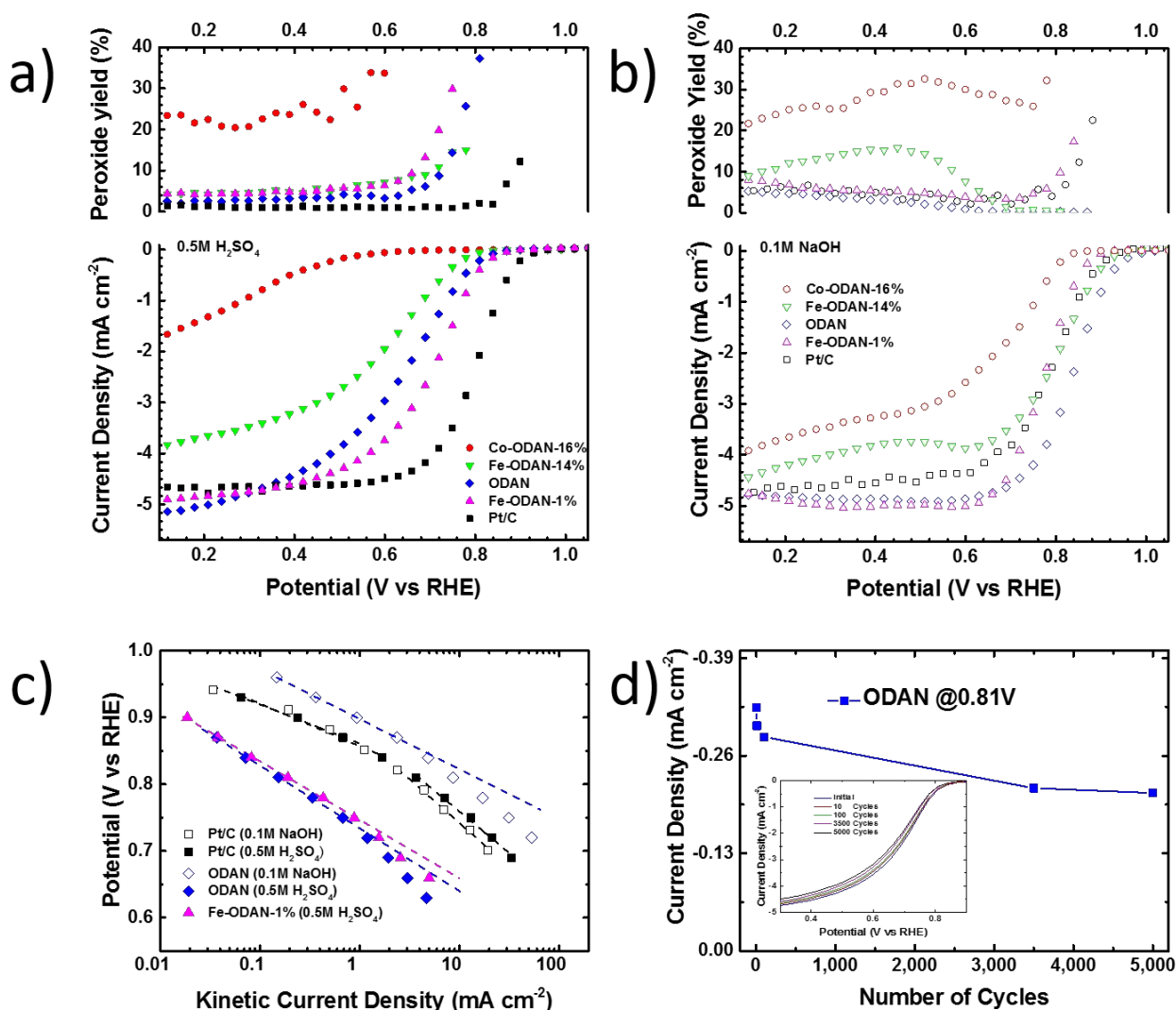
Figure 4: a) Steady-state RRDE measurement in 0.5M H 2 SO 4 , Rotating speed: 1600 rpm, 30s hold, 30 mV step potential, catalyst loading: non-precious metal catalysts: 750 μg/cm 2 , Pt/C: 60 μg Pt /cm 2 , O 2 -saturated at 1 atm (bottom) ORR activity (top) Peroxide yield b) in 0.1M NaOH c) Tafel plot of selected catalysts in 0.5M H 2 SO 4 and 0.1M NaOH d) long term stability test: current density in O 2 -saturated 0.5M H 2 SO 4 at different potentials after cycling between 0.6 and 1V versus RHE in N 2 -saturated 0.5M H 2 SO 4 .
