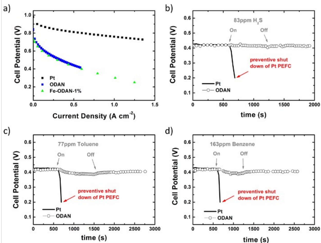
Figure 7: a) \text{H}_2\text{-O}_2 polarization plot for MEA comparing cathodes, brush painted with ODAN and Fe-ODAN-1% ( 4 \text{ mg}/\text{cm}^2 ) to a commercial Pt cathode ( 0.4 \text{ mg}_{\text{Pt}}/\text{cm}^2 ). b) Cell voltage before and after adding b) 83 ppm \text{H}_2\text{S} c) 77 ppm Toluene and d) 163 ppm Benzene into the cathode gas stream.
