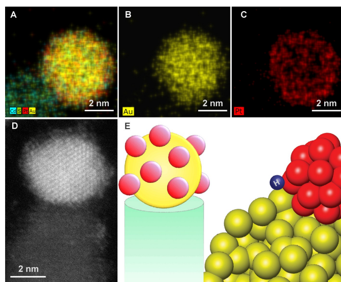
Figure 3. X-ray energy dispersive spectroscopy micrographs with elemental mapping (A–C) and an atomic resolution HAADF image (D) of the bimetallic tip, demonstrating the formation of a Au core that is decorated with islands of Pt (E). The Au–Pt boundary is suggested to be the active catalytic site.
