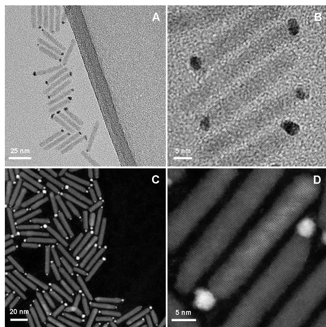
Figure 1. TEM (A,B) and HAADF (C,D) micrographs of CdSe@CdS nanorod photocatalysts with Au-Pt bimetallic tips acting as cocatalyst reduction sites.
