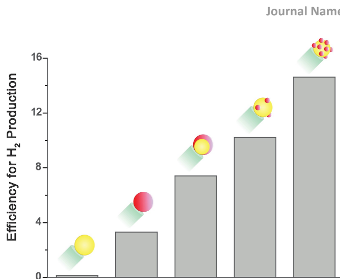
Figure 2. Relative efficiency for the photocatalytic hydrogen production half reaction utilizing CdSe@CdS nanorods decorated with different metal cocatalysts serving as the reduction site: Au, Pt, Au@Pt core shell and Au-Pt. All measurements were done using identical solution conditions, and at equivalent concentrations.
