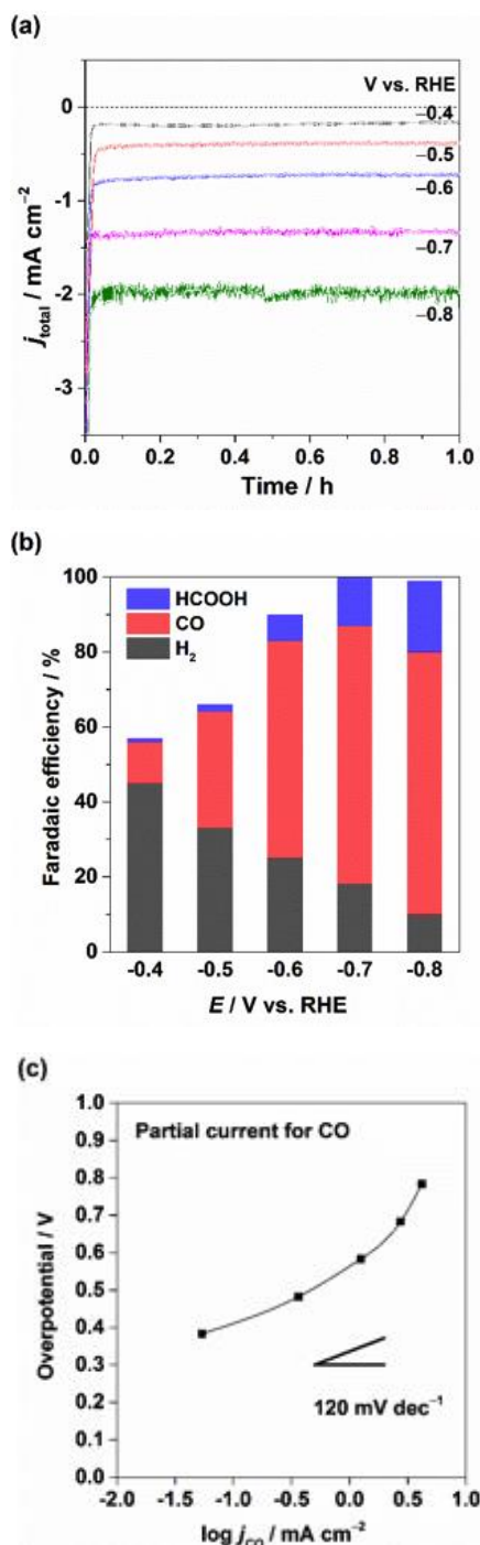
Fig. 3. (a) Chronoamperometric electrolysis profiles, (b) their Faradaic efficiencies, and (c) Tafel analysis for j_{\text{CO}} using the CuIn electrode in \text{CO}_2 -saturated 0.1 M \text{KHCO}_3 aq.
