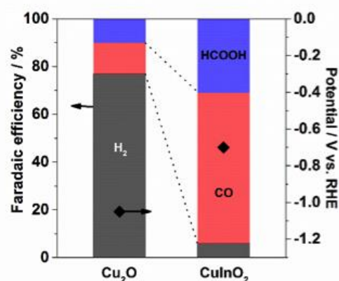
Fig. 2. Comparison of the chronopotentiometric results of Cu-based electrodes at j_{\text{tot}} of -1.67 \text{ mA cm}^{-2} in CO 2 -saturated 0.1 M KHCO 3 aq. (pH 6.8).
