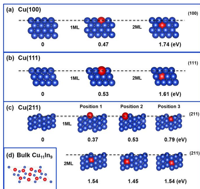
Fig. 7. Side views of (a) Cu(100), (b) Cu(111) and (c) Cu(211) with one In atom replacing a Cu atom for the first layer (1ML) and the second layer (2ML). The energies relative to the most stable structure (left) are presented. (d) Top view of bulk \text{Cu}_{11}\text{In}_9 .
