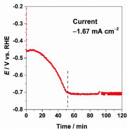
Fig. 1. Chronopotentiometric electrolysis of CuInO 2 (initial reduction) at j_{\text{tot}} of -1.67 \text{ mA cm}^{-2} in CO 2 -saturated 0.1 M KHCO 3 aq. (pH 6.8).
