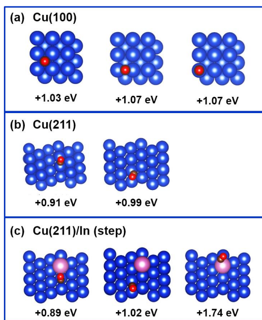
Fig. 9. Optimized geometries and relative energy of CO adsorbed on the pure Cu (100) and Cu (211), and the In modified (211) Cu facet. The values shown in the figure represents \Delta E , the electronic energy of the state minus the electronic energy of the clean slab associated with that state, with the C atom referenced to graphene and the O atom to ( \text{H}_2\text{O} - \text{H}_2 ) ( \Delta E(\text{CO}) = E(\text{slab} + \text{CO}) - E(\text{slab}) - E(\text{C})/4 - [E(\text{H}_2\text{O}) - E(\text{H}_2)] ).
