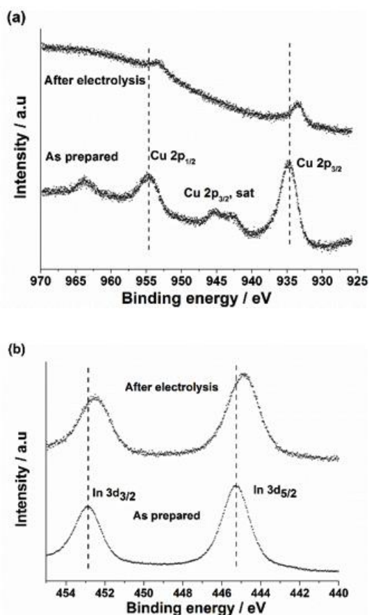
Fig. 5. XPS spectra of (a) Cu 2p and (b) In 3d for as-prepared and after-electrolysis CuIn samples.
