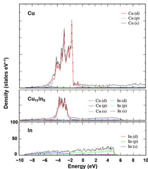
Fig. 6. Density of states of Cu, Cu 11 In 9 , and In for respective orbitals.
