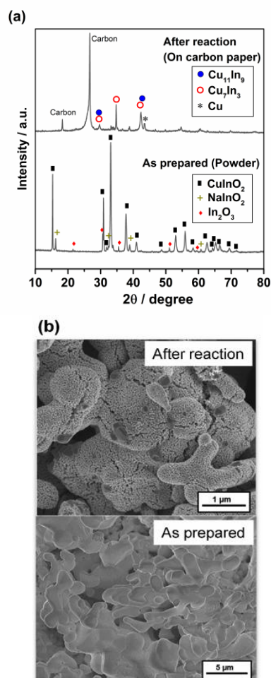
Fig. 4. a) XRD profiles and b) SEM images of the as-prepared and after-electrolysis CuIn electrodes.
