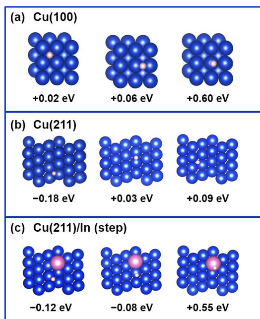
Fig. 8. Optimized geometries and relative energy of H adsorbed on the pure Cu (100) and Cu (211), and the In modified (211) Cu facet. The values shown in the figure represents \Delta E , the electronic energy of the state minus the electronic energy of the clean slab associated with that state, with the H atom referenced to 1/2 \text{H}_2 ( \Delta E(\text{H}) = E(\text{slab} + \text{H}) - E(\text{slab}) - E(\text{H}_2)/2 ).
