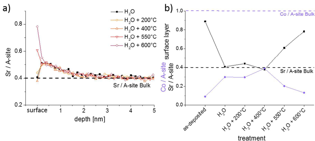
Fig. 10 (a) LEIS depth profiles showing the Sr / A-site ratio after annealing thin films for 1 h at different temperatures; (b) Co / A-site and Sr / A-site ratio of the termination layer of the same thin films
