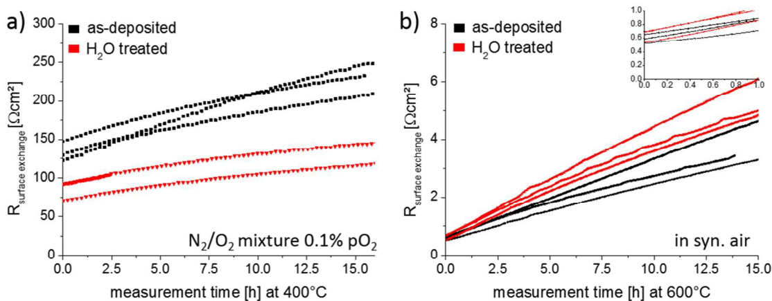
Fig. 12 Variation of the surface exchange resistance for as-deposited and H_2O treated thin films with annealing time. Measurements were performed (a) at 400°C in 0.1% pO_2 and (b) at 600°C in 21% pO_2
