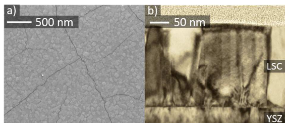
Fig. 1 SEM image of a LSC thin film surface (a) and TEM cross-section of a ~210 nm thin LSC film (b)
