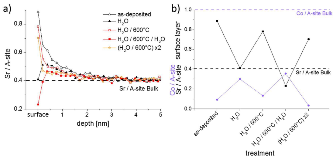
Fig. 8 (a) LEIS depth profiles showing the Sr / A-site ratio after different surface treatments; (b) Co / A-site and Sr / A-site ratio of the termination layer is displayed after different surface treatments
