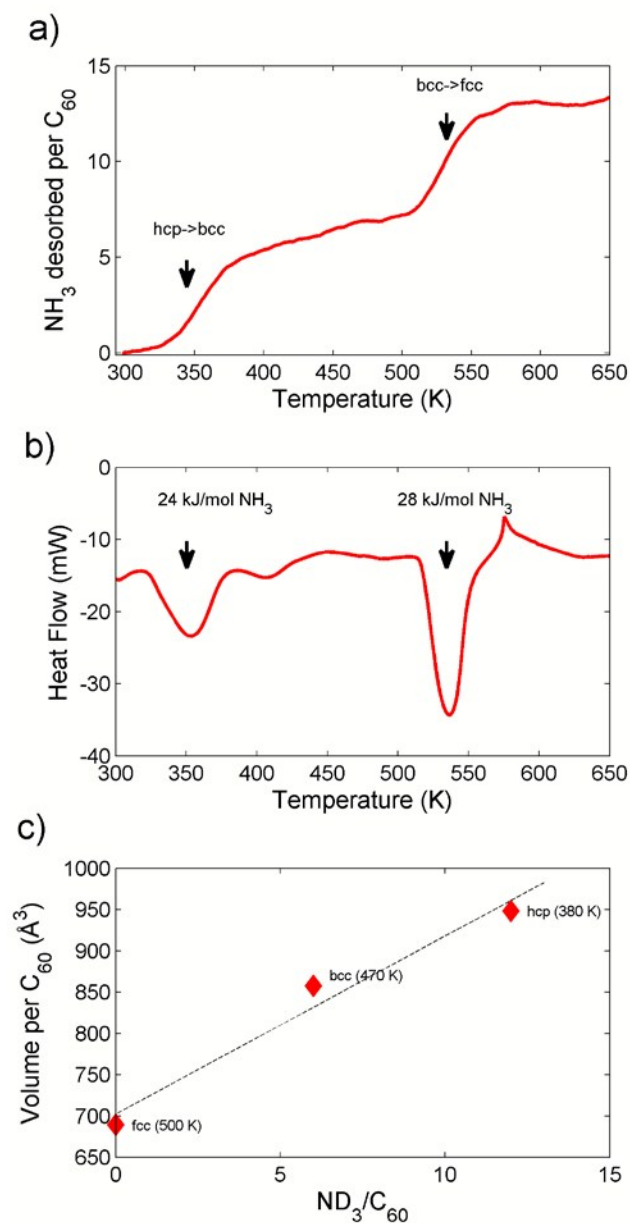
Figure 3: a) Manometric data of the \text{NH}_3 desorption process in (\text{NH}_3)_y\text{Li}_6\text{C}_{60} upon heating in the range 300-650 K (rate of 5 K/min). b) DSC data of the \text{NH}_3 desorption process. c) Refined volume per \text{C}_{60} as a function of the number of ammonia molecules intercalated for the ammonia free-, super-expanded \text{bcc} - and hyper-expanded \text{hcp} phases of (\text{NH}_3)_y\text{Li}_6\text{C}_{60} . The observed trend is roughly linear (dotted line).
