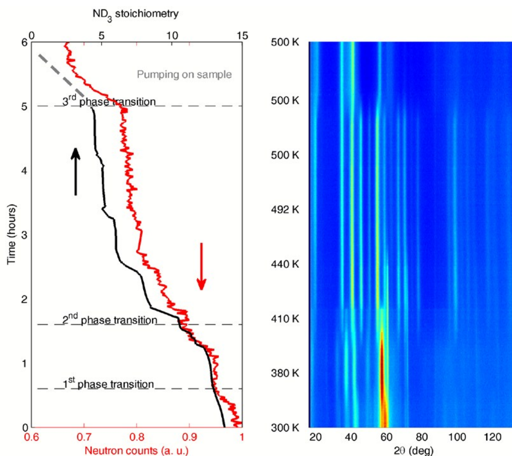
Figure 1: Left: Time evolution of the normalized total counts (red) of (ND 3 ) y Li 6 C 60 , plotted together with the estimated ND 3 stoichiometry of the sample (black), as evaluated by in-situ Sievert analysis. Right: Colour map showing the thermal evolution of the neutron diffraction profile in the range 300–500 K. The presence of three structural phase transitions at 350 K, 410 K and 500 K is evident. These are promoted by the progressive desorption of ND 3 molecules, co-intercalated in the host fullerene lattice. Discrete temperature points are reported in the middle, referring both to the left and right plots.
