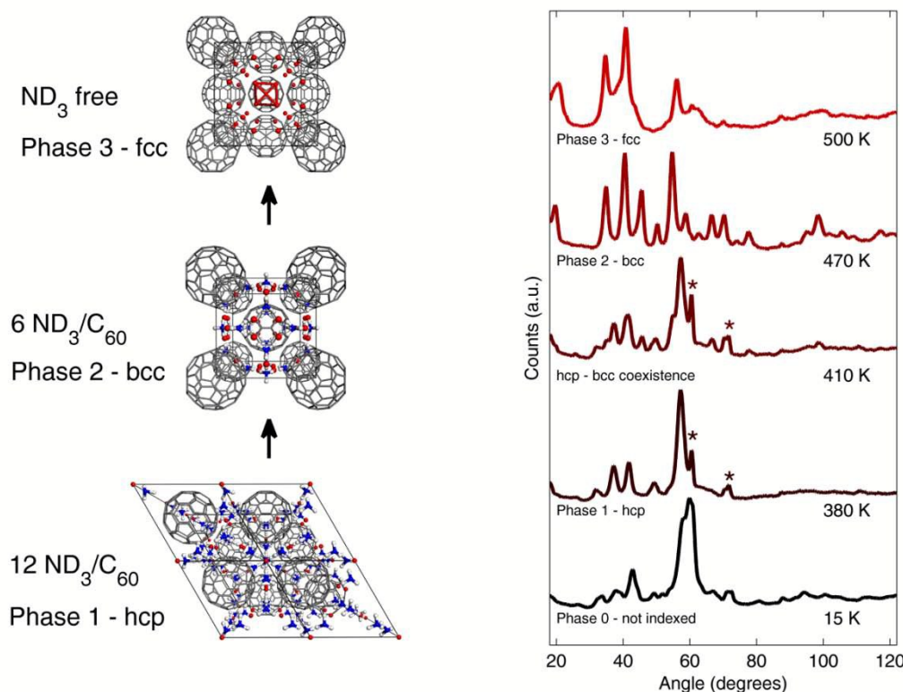
Figure 2: Left: structural representation for the three indexed phases of Li_6C_{60} at different degrees of ammoniation. Right: selected powder neutron diffraction patterns of the (ND_3)_xLi_6C_{60} sample during the ND_3 desorption process, referring to the four identified phases discussed in the text. Some sharp peaks (indicated by asterisks) were ascribed to the spurious LiND_2 phase, which in this sample is present in a very low amount (<2 wt%), thus not significantly affecting the sample properties.
