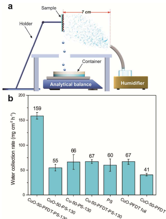
Fig. 6. (a) Schematic illustration of the homemade fog-harvesting system. (b) Water collection rates of different samples.
