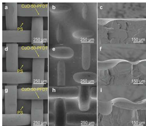
Fig. 5. The SEM images of composite surfaces composed of the PS and PFDT modified CuO gauze with 50# mesh size prepared under different thermal treatment temperature (a, d, g), and the SEM top view (b, e, h) and cross-section view (c, f, i) of the PS surface morphology (a, b, c at 120 °C; d, e, f at 130 °C; g, h, i at 140 °C) with the gauzes being removed.
