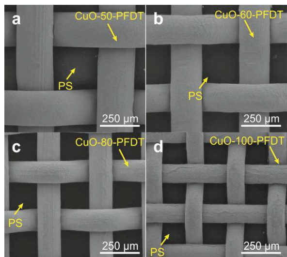
Fig. 4. The top view SEM images of the hybrid surfaces composed of the PS and PFDT modified CuO gauze with different mesh numbers (a) 50#, (b) 60#, (c) 80#, (d) 100#.
