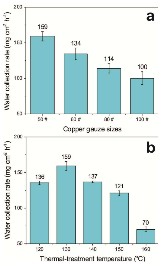
Fig. 7. (a) Water collection rates as a function of mesh number; (b) the comparison of water collection efficiency by the samples prepared at different thermal treatment temperature.
