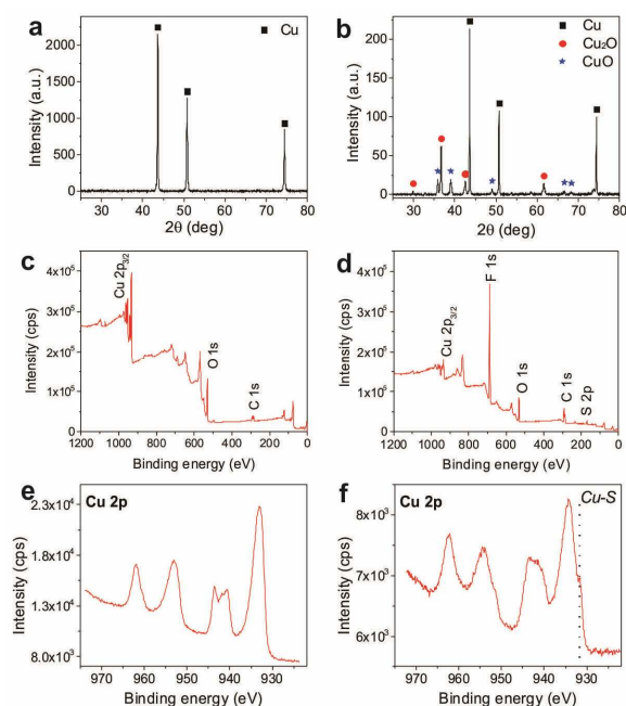
Fig. 2. XRD patterns of raw Cu gauze (50# mesh) (a) and CuO-50 (b). XPS spectra of CuO-50 (c), CuO-50-PFDT (d), and the Cu2p spectra of CuO-50 (e), CuO-50-PFDT (f).
