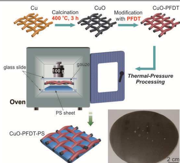
Scheme 1. The preparation procedure for the hydrophilic-superhydrophobic patterned composite surface: (i) calcination of copper gauze to form oxide surface coating layer; (ii) hydrophobic modification of the oxide coated copper gauze with PFDT; (iii) thermal-pressing of the PFDT modified gauze and PS sheet to form the composite surface with patterned wettability. The insert image presents some water droplets sitting on a composite sample surface.
