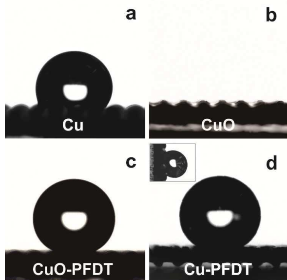
Fig. 3. The CA measurement images of the sample prepared from 50# gauze at different preparation stages, including (a) Cu, (b) CuO, (c) CuO-PFDT and (d) Cu-PFDT. The inset image was the water contact angle of Cu-PFDT with tilt angles of 90°. The water droplet volume in these images was all 5 \mu\text{L} .
