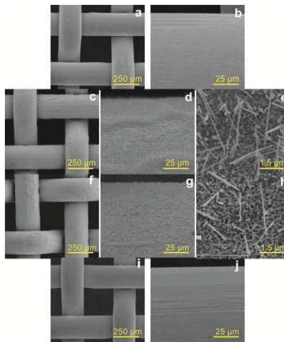
Fig. 1. SEM images of the samples prepared from 50# gauzes at different preparation stages: Cu (a, b), CuO (c-e), CuO-PFDT (f-h) and Cu-PFDT (i, j).
