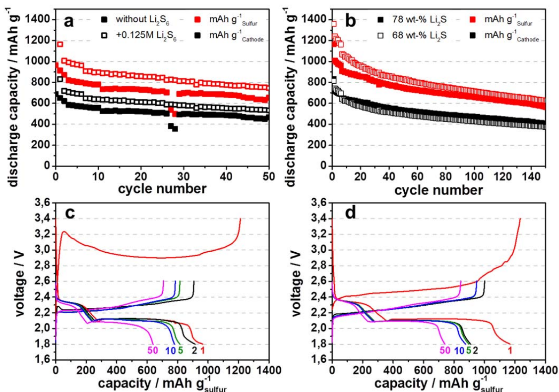
Figure 8 a) Galvanostatic discharge capacity over cycle number at a C-rate of 0.1 for Li 2 S based cathodes made from 60 h ball milled Li 2 SO 4 with KB EC-600JD as porous carbon host structure in the cathode and 1 M LiTFSI, 0.25 M LiNO 3 in DME/DOL (1:1 vol/vol) (filled symbols) or 1 M LiTFSI, 0.125 M LiNO 3 and 0.125 M Li 2 S 6 polysulfide in DME/DOL (1:1 vol/vol) (empty symbols), respectively, as electrolyte; b) Comparing the discharge capacities of cathodes consisting of 78 and 68 wt-% Li 2 S with 0.125 M Li 2 S 6 polysulfide containing electrolyte; voltage profiles during charge and discharge for chosen cycles at a C-rate of 0.1 for Li 2 S based cathodes made from 60 h ball milled Li 2 SO 4 , c) without and d) with 0.125 M Li 2 S 6 addition to the electrolyte.
