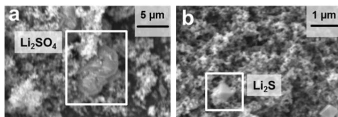
Figure 2 SEM images from a Li 2 SO 4 ·H 2 O sample before (a) and after (b) the heat treatment at 820 °C under argon atmosphere.
