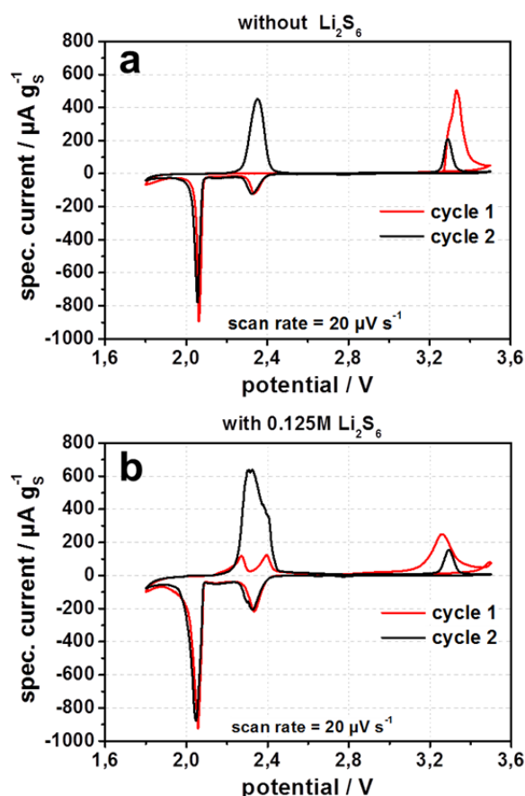
Figure 9 a,b) Cyclic voltammograms for the two first cycles at a scan speed of 20 \mu\text{V s}^{-1} , for \text{Li}_2\text{S} based cathodes made from 60 \text{ h} ball milled \text{Li}_2\text{SO}_4 with KB EC-600JD as porous carbon host structure in the cathode. a) 1 \text{ M LiTFSI} , 0.25 \text{ M LiNO}_3 in DME/DOL (1:1 vol/vol) and b) 1 \text{ M LiTFSI} , 0.125 \text{ M LiNO}_3 and 0.125 \text{ M Li}_2\text{S}_6 polysulfide in DME/DOL (1:1 vol/vol) as electrolyte.
