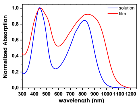
Figure 1. Absorption spectra of TBDPTV in chloroform solution and as thin film.
