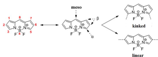
Scheme 1. Chemical structure of BODIPY dye and assignment of the different positions and forms
