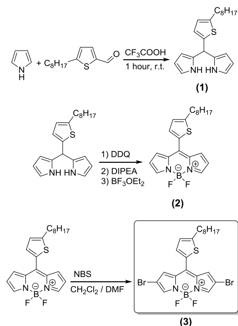
Scheme 2. Reaction procedures towards the synthesis of dibromo borondipyrrromethene monomer 3
