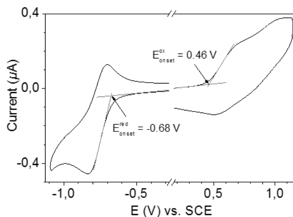
Figure 2. Cyclic voltammogram of TBDPTV in chloroform (containing 0.1 M tetrabutylammonium perchlorate).
