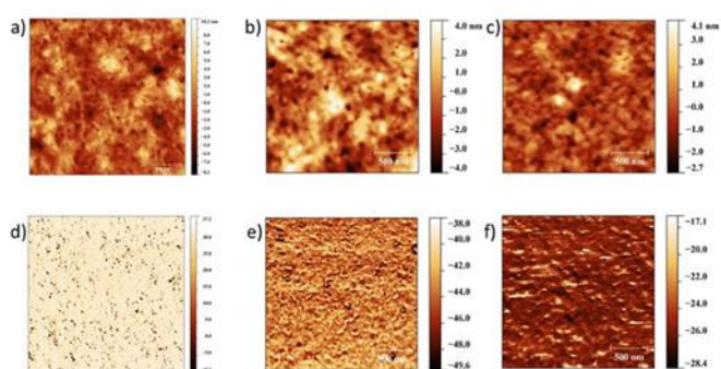
Figure 5. Topography(a,b,c) and phase (d,e,f) images of films TBDPTV:PC 71 BM 1:2, 1:3 and 1:4 respectively, on top of a layer of ZnO, as measured by intermittent contact mode atomic force microscopy.
