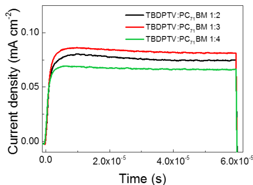
Figure 4. Time-dependent photo-CELIV traces of TBDPTV-based solar cells at a fixed delay time of 1 \mu\text{s} .
