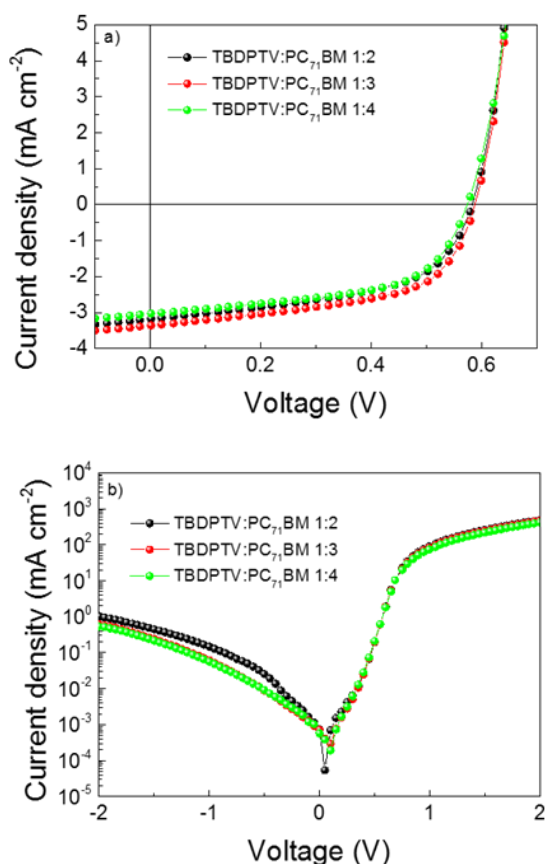
Figure 3. Current density-voltage characteristics under 100 \text{ mW cm}^{-2} illumination (AM1.5G) (a) in linear graph and (b) in semilogarithmic graph.
