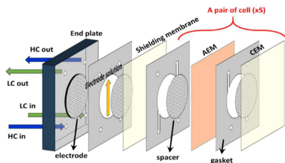
Fig. 1 Schematic diagram of RED stack
