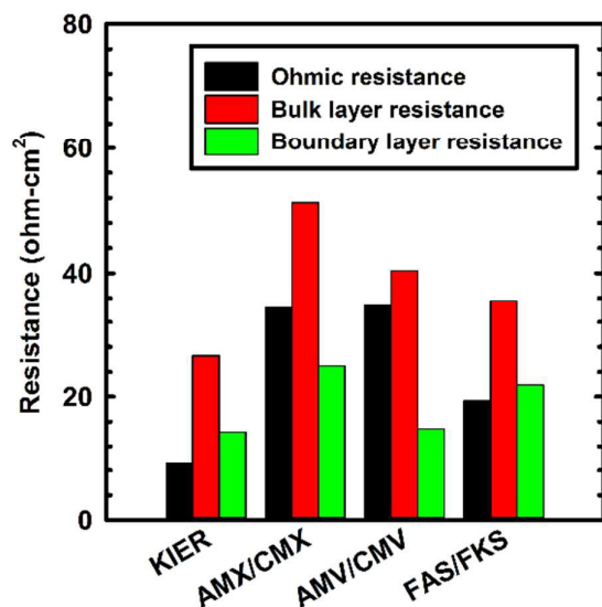
Fig. 3 Internal resistance contributions with respect to IEMs.
