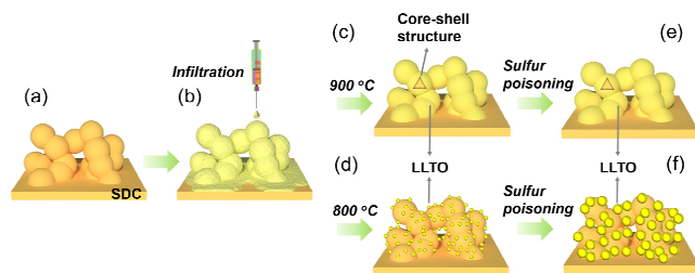
Figure 1 Schematic diagrams of the preparation processes for the nanoparticle-decorated electrode and core-shell structured electrode prepared by solution infiltration (a-d) and the possible mechanism for the sulfur poisoning process of the different anodes. (e and f)
