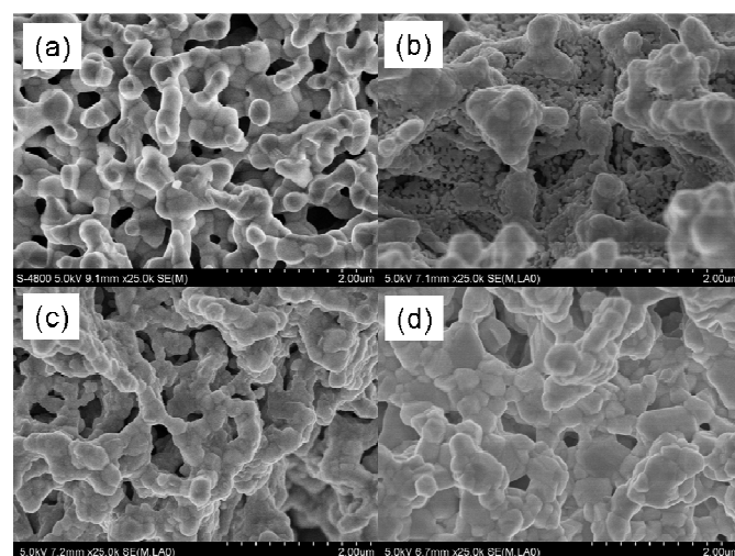
Figure 2 SEM images of (a) as-prepared SDC scaffold and the LLTO-infiltrated SDC anodes after firing at (b) 800, (c) 900 and (d) 1000 °C for 2 hours.
