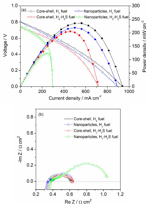
Figure 5 The typical I-V , I-P polarization curves (a) and EIS spectra (b) of the fuel cells with LLTO-infiltrated SDC anodes with different structures operating on 1000 ppm \text{H}_2\text{S-H}_2 at 800 °C.
