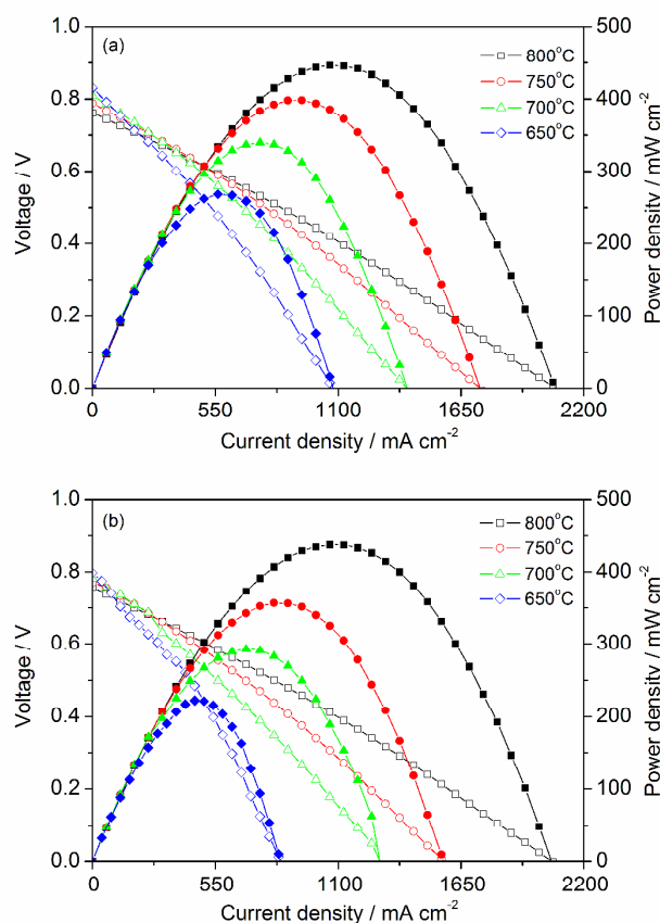
Figure 10 The typical I-V , I-P polarization curves of the fuel cells with Ni-LLTO co-infiltrated SDC anodes after calcination at 900 °C operating on H 2 (a) and 1000 ppm H 2 S-H 2 (b).
