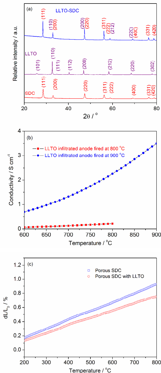
Figure 4 (a) XRD patterns of LLTO-infiltrated SDC anodes after calcination at 900 °C for 2 hours, as well as the pure phases such as SDC and LLTO, (b) Electrical conductivities of the LLTO infiltrated SDC anodes after sintering at 800 and 900
