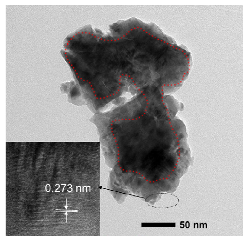
Figure 3 TEM results under different magnifications of the core-shell structured LLTO-infiltrated SDC anodes.
