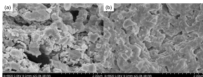
Figure 8 SEM photos of the LLTO-infiltrated SDC anodes with different structures (a) nanoparticles and (b) thin film after the operational stability test on 1000 ppm \text{H}_2\text{S}-\text{H}_2 fuel.
