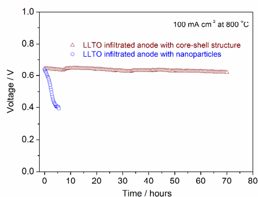
Figure 7 Time-dependent voltage of the fuel cell with LLTO-infiltrated SDC anodes with different structures operating on 1000 ppm \text{H}_2\text{S}-\text{H}_2 under a current density of 100 \text{ mA cm}^{-2} at 800 °C.
