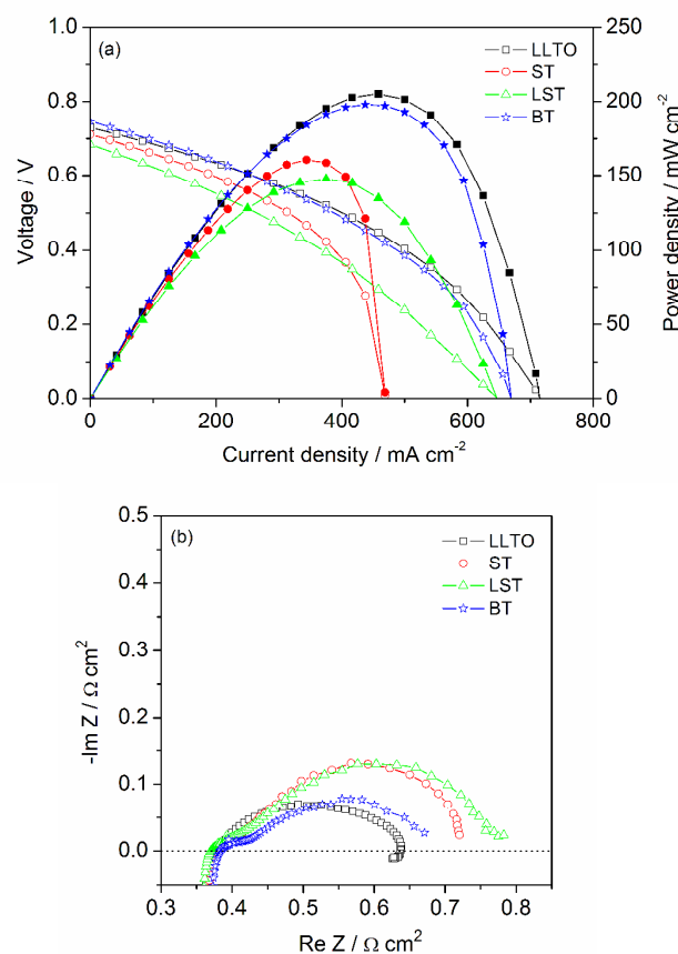
Figure 6 Typical I-V , I-P polarization curves (a) and EIS spectra (b) of the fuel cells with different infiltrated anodes operating on 1000 ppm \text{H}_2\text{S-H}_2 at 800 °C.
