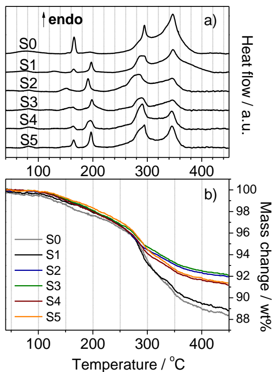
Fig. 3 DSC (a) and TG (b) curves for samples S0-S5 ( \Delta T/\Delta t = 2\text{ }^{\circ}\text{C}/\text{min} ).
