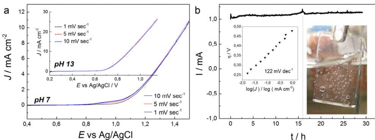
Figure 5. (a) LSV curves of CoNCN, recorded at different scan rates in 0.1 M phosphate buffer at a rotation speed of 1500 rpm ( E^0(\text{pH } 7) = 0.62 V and E^0(\text{pH } 13) = 0.27 V vs. Ag/AgCl). (b) Representative chronoamperometry measurement of CoNCN on a FTO electrode at 1.2 V vs. Ag/AgCl in 0.1 M phosphate buffer ( E^0(\text{pH } 7) = 0.62 V vs. Ag/AgCl). The dotted line indicates mechanical removal of bubbles. The inset shows the Tafel plot with a glassy carbon electrode under the same conditions.
