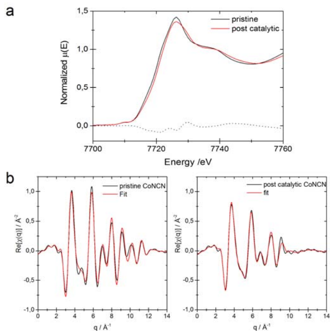
Figure 3. (a) XANES region for pristine and post-catalytic CoNCN and their difference spectrum. (b) EXAFS fit for pristine catalytic CoNCN vs. crystallographic data. 66
