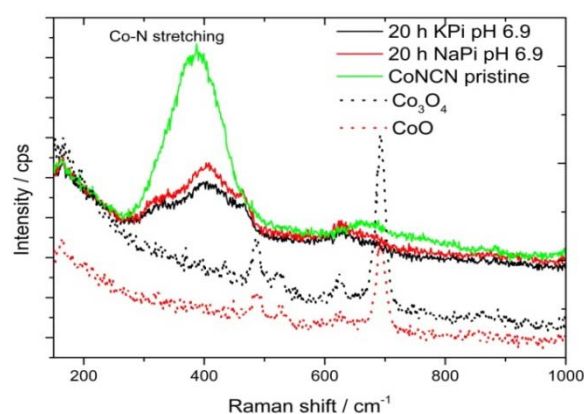
Figure 7. Raman spectra of post-electrocatalytic CoNCN on FTO electrodes after 20 h of electrolysis in KPi and NaPi media (pH 7) vs. reference data for Co 3 O 4 and CoO.
