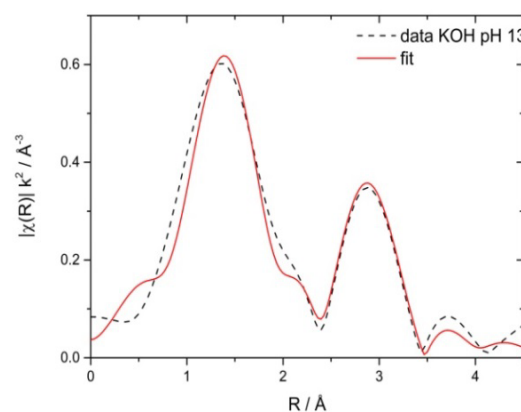
Figure 6. Representative EXAFS spectrum of CoNCN electrocatalyst on a FTO electrode after 20 h of electrolysis in KOH (pH 13) fitted vs. structural reference data. 66
