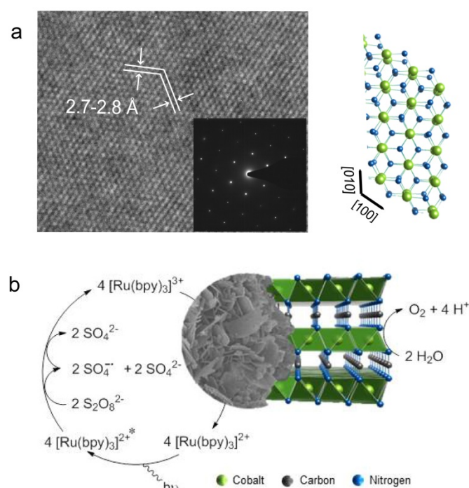
Figure 1. (a) HRTEM and SAED pattern of a CoNCN platelet along with the structural motif. (b) Photocatalytic water oxidation cycle with cobalt carbodiimide.
