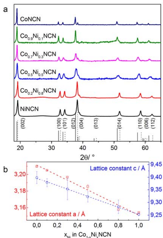
Figure 8. (a) PXRD patterns of \text{Co}_{1-x}\text{Ni}_x\text{NCN} catalysts with different metal ratios and (b) the corresponding Vegard diagram (reference patterns: — CoNCN [ICDD 04-015-1039] and - - - NiNCN [ICDD 04-015-1038]).
