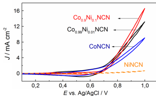
Figure 9. CV curves of \text{Co}_{1-x}\text{Ni}_x\text{NCN} catalysts with different metal ratios (glassy carbon electrodes; scan rate: 25 \text{ mV s}^{-1} , 0.1 M NaOH ( E^0(\text{pH } 13) = 0.27 \text{ V} )).
