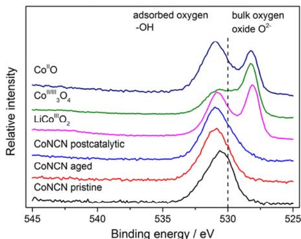
Figure 4. XPS analysis of CoNCN O1s XPS peaks (pristine, aged in carbonate buffer and post-photocatalytic) vs. cobalt oxide references.
