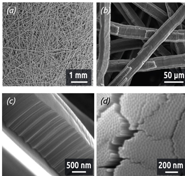
Fig. 12. SEM micrographs of Ti fleeces before anodization (a) and after anodization (glycerol + 0.5 wt-% NH 4 F, 40 V, 2 h, (b,c)). The lower extremity of TiO 2 tubes in an oxide block separated from the underlying Ti is shown in (d). An ultrasonication treatment has been performed before SEM observation in order to provide insight into the otherwise solid oxide layer.
