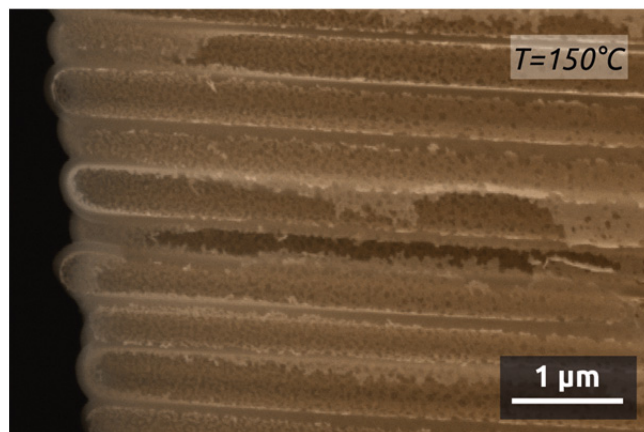
Fig. 6. SEM micrograph of AAO membrane coated by Pt deposited by ALD at 150°C.
