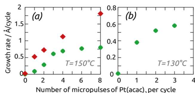
Fig. 1. Growth rates determined at 150°C (a) and at 130°C (b) as a function of the Pt(acac) 2 dosage by GCM for depositions using short 1 to 8 s (green) and long 30 s (red) exposure durations. The former give rise to self-limiting ALD behavior, the latter do not.
