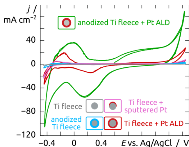
Fig. 13. Cyclic voltammetry performed on Ti fleeces under different conditions with and without Pt. Ti fleeces have been anodized and Pt has been deposited either by magnetron sputtering or by ALD. Scan rate: 100 mV/s. Internal resistance compensation was performed.
