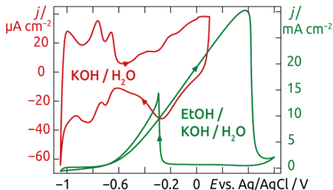
Fig. 11. Cyclic voltammograms of Pt clusters supported on TiO 2 nanotubes carried out in 1 M KOH and in 1 M KOH + 1 M EtOH. Scan rate: 50 mV/s.
