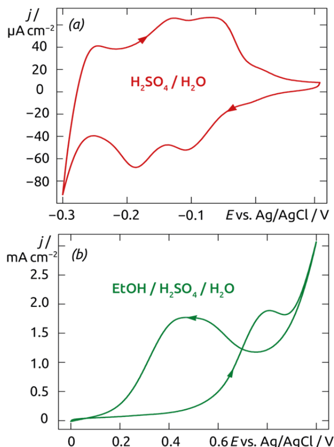
Fig. 10. Cyclic voltammograms of Pt clusters supported on TiO 2 nanotubes carried out in acidic medium (0.5 M H 2 SO 4 (a), and 0.5 M H 2 SO 4 + 1 M EtOH (b)). Scan rate: 50 mV/s.
