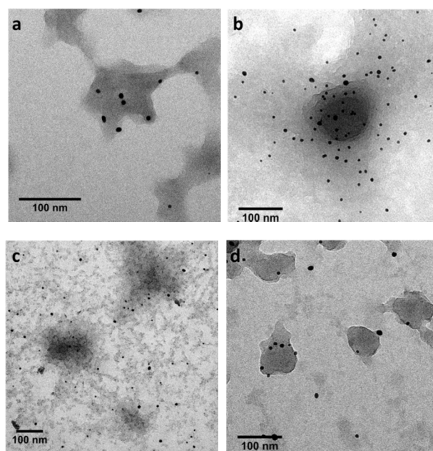
Figure 3. TEM images of the PVCL-CD-Au microgel particles synthesized with different amount of 0.01 M HAuCl 4 : (a) 0.1 ml, (b) 0.2 ml, (c) 0.3 ml and (d) 0.4 ml.
