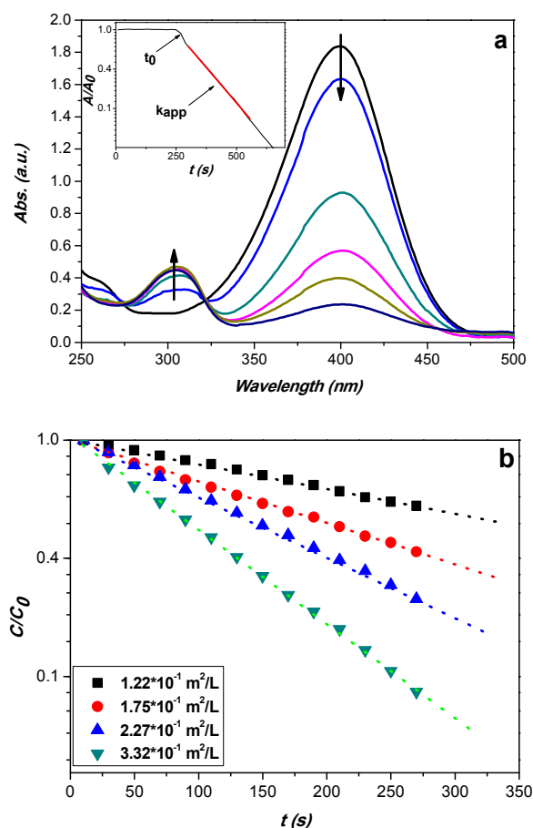
Figure 6. (a) UV-vis absorption spectra of Nip reduced by sodium borohydride using PVCL- \alpha -CD(13.08 wt.-%)-Au particles as catalyst at room temperature. The inset shows typical time dependence of the absorption of 4-nitrophenolate ions at 400 nm. (b) Kinetic analysis of the Nip reduced by
