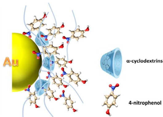
Figure 8. Immobilization of Nip on the \alpha -CD-modified Au nanoparticle surface.
