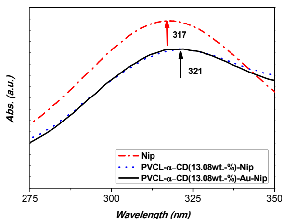
Figure 5. UV-vis spectra of Nip mixed with PVCL- \alpha -CD(13.08 wt.-%)-Au microgels (solid line); PVCL- \alpha -CD(13.08 wt.-%) microgels (dot line) and pure Nip (dash dot line). Concentrations: Nip: 10^{-5} mol/L; microgels: 0.203 mg/ml.
