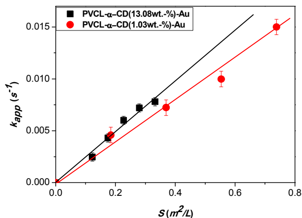
Figure 7. Rate constant ( k_{\text{app}} ) as a function of surface area S of Au nanoparticles normalized to the unit volume of the system: PVCL- \alpha -CD(13.08 wt.-%)-Au (solid squares) and PVCL- \alpha -CD(1.03 wt.-%)-Au (solid circles) at room temperature.
