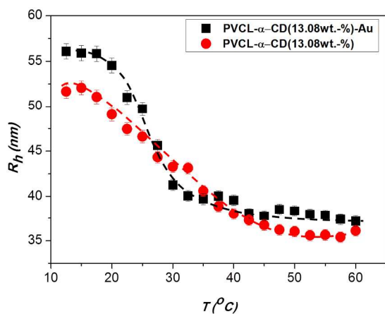
Figure 4. Hydrodynamic radius of PVCL- \alpha -CD(13.08 wt.-%) microgels with and without Au nanoparticles as a function of temperature in aqueous solution.
