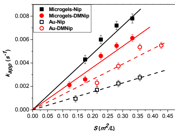
Figure 9. Rate constant k_{app} of the PVCL- \alpha -CD(13.08 wt.-%)-Au and pure Au nanoparticles for the catalytic reduction of 4-nitrophenol (Nip) and 2,6-dimethyl-4-nitrophenol(DMNip) by sodium borohydride as a function of surface area S of Au nanoparticles normalized to the unit volume of the system.
