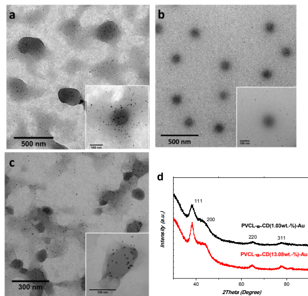
Figure 1. TEM images of (a) PVCL- \alpha -CD(13.08 wt.-%)-Au microgel nanoparticles, (b) PVCL-Au microgel nanoparticles and (c) PVCL- \alpha -CD(1.03 wt.-%)-Au microgel nanoparticles. (d) XRD patterns of PVCL- \alpha -CD(1.03 wt.-%)-Au (black) and PVCL- \alpha -CD(13.08 wt.-%)-Au (red).
