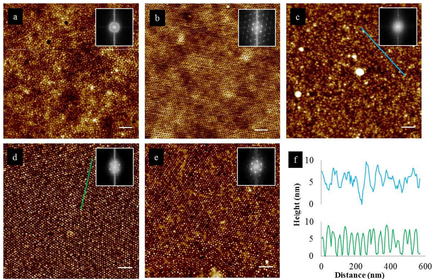
Fig. 1 Atomic force microscopy height images of PS- b -PEO films after solvent vapor annealing with (a) toluene and (b) toluene/water. TiO 2 arrays were templated by (c) EISA and (d) SPICE; and (e) AuNPs were spincoated onto templated SPICE TiO 2 . Inset images are FFTs of the AFM images. Scale bars represent 200 nm. (f) Line scans show height profiles of the TiO 2 made by the SPICE (green, bottom) and EISA (blue, top) methods.
