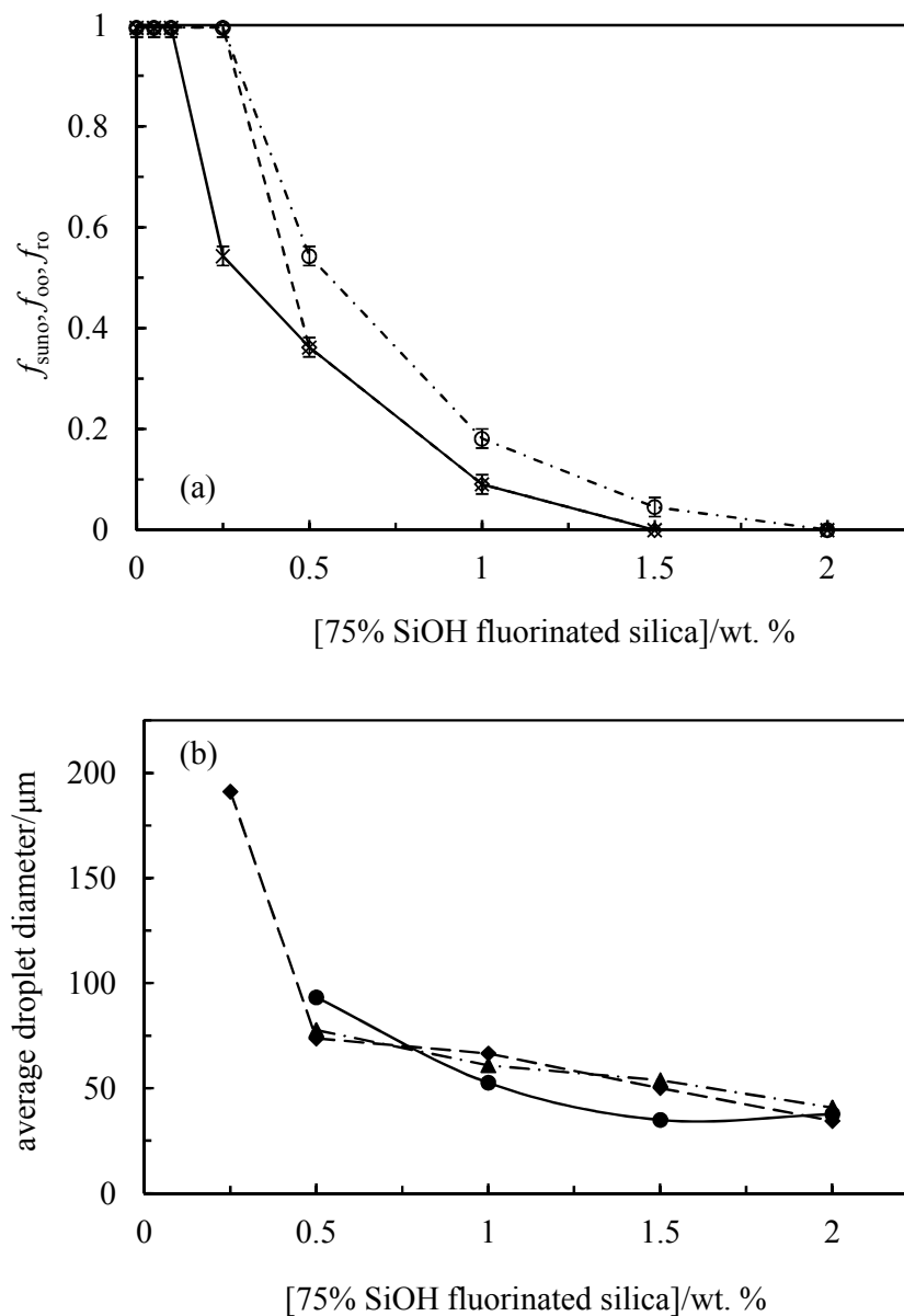
Figure 10. (a) Fraction of sunflower oil f_{\text{sun0}} ( \circ ) or olive oil f_{\text{oo}} ( \diamond ) or rapeseed oil f_{\text{ro}} ( \times ) released from 50 cS PDMS-in-sunflower oil, 50 cS PDMS-in-olive oil or 50 cS PDMS-in-rapeseed oil emulsions, respectively, shown in Figure 9 versus concentration of 75% SiOH fluorinated silica particles. (b) Average droplet diameter after 1 month of PDMS drops in sunflower oil ( \bullet ), olive oil ( \blacktriangle ) or rapeseed oil ( \blacklozenge ) emulsions versus particle concentration. The standard deviation decreases from \sim 40 \mu\text{m} at 0.25 wt.% to \sim 10 \mu\text{m} at 2 wt.%.
