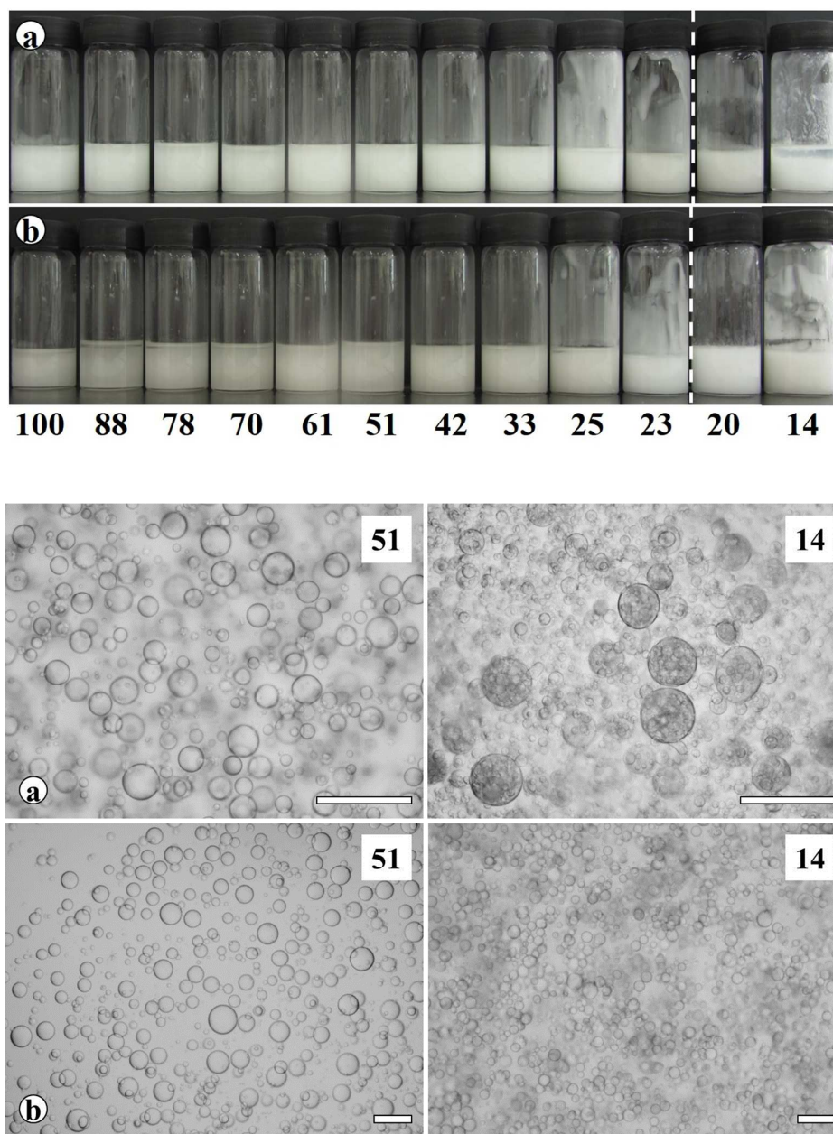
Figure 5. (upper) Photographs of glass vials containing (a) sunflower oil-100 cS PDMS and (b) olive oil-100 cS PDMS emulsions (both 1:1) after 1 month stabilised by 1 wt.% of DCDMS-coated fumed silica particles with different % SiOH on their surfaces (given). Dashed line indicates transitional phase inversion. (lower) Corresponding optical micrographs of the emulsions at selected % SiOH (given). Scale bars = 200 \mu\text{m} .
