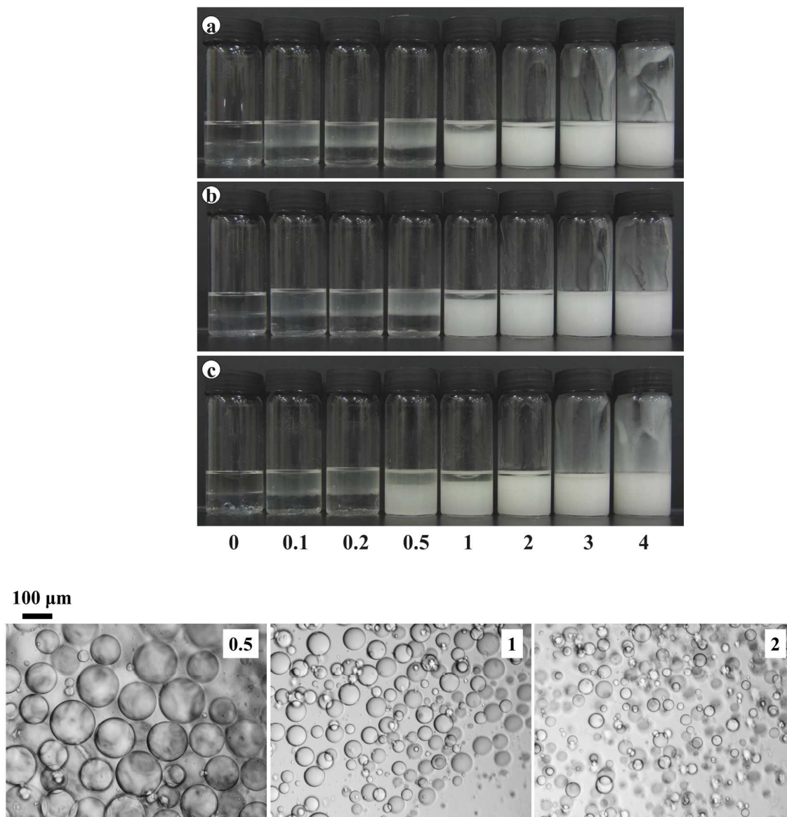
Figure 9. (upper) Photographs of glass vials containing 50 cS PDMS-in-(a) sunflower oil, (b) olive oil or (c) rapeseed oil emulsions (1:1) 1 month after preparation stabilised by different concentrations (given, wt.%) of 75% SiOH fluorinated fumed silica particles. (lower) Corresponding optical micrographs of the emulsions in (a) at selected particle concentrations (given, wt.%).
