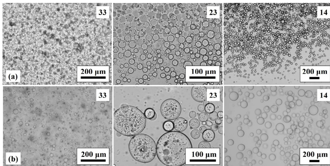
Figure 3. Corresponding optical micrographs of the emulsions shown in Figure 2 at selected % SiOH (given) for (a) sunflower oil and (b) olive oil with DCDMS-coated particles.
