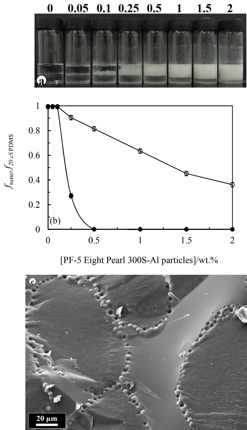
Figure 12. (a) Photographs of glass vials containing sunflower oil-in-20 cS PDMS emulsions (1:1, 1 month after preparation) stabilised by different concentrations (given, wt.%) of PF-5 Eight Pearl 300S-Al particles, (b) fraction of sunflower oil f_{\text{sun}}(\bullet) and fraction of PDMS oil f_{20\text{cS PDMS}}(\circ) released from above emulsions versus particle concentration, (c) cryo-SEM image of a sunflower oil-in-50 cS PDMS emulsion stabilised by 1 wt.% of silicone particles of PF-5 Tospearl 145A.
