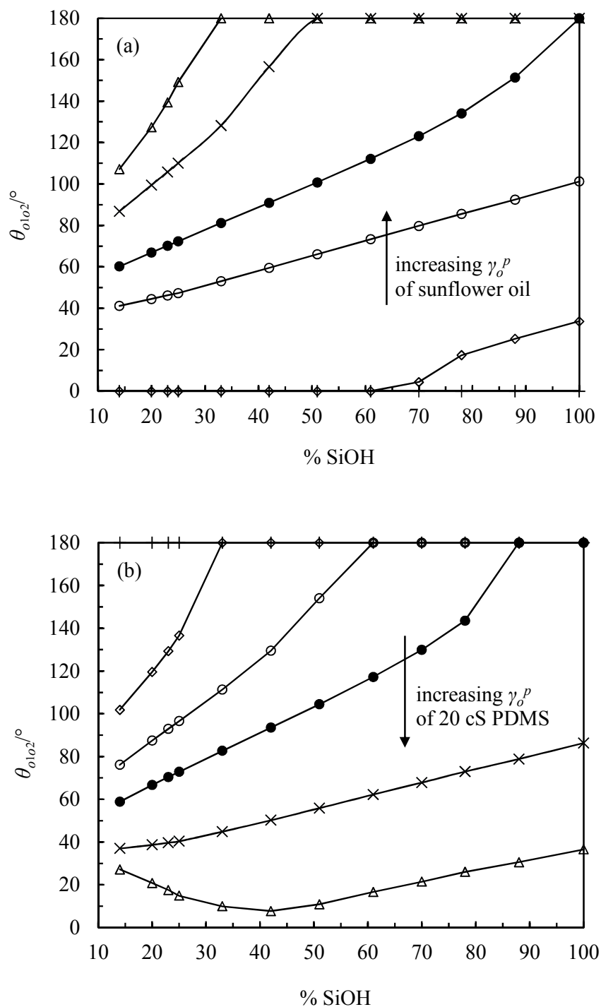
Figure 8. Plot of calculated \theta_{o_1o_2} into PDMS versus % SiOH on DCDMS-coated fumed silica particle surfaces for the interface sunflower oil-20 cS PDMS with (a) \gamma_o^p ; \gamma_o^d = 0 ; 33.3 (+), 0.2; 33.1 ( \diamond ), 0.4; 32.9 ( \circ ), 0.6; 32.7 ( \bullet ), 1.0; 32.3 ( \times ) and 1.4; 31.9 ( \triangle ) mN m -1 for sunflower oil and \gamma_o^p ; \gamma_o^d = 0.9 ; 19.9 mN m -1 for PDMS and (b) \gamma_o^p ; \gamma_o^d = 0 ; 20.8 (+), 0.2; 20.6 ( \diamond ), 0.4; 20.4 ( \circ ), 0.6; 20.0 ( \bullet ), 1.0; 19.8 ( \times ) and 1.4; 19.4 ( \triangle ) mN m -1 for PDMS and \gamma_o^p ; \gamma_o^d = 0.4 ; 32.9 mN m -1 for sunflower oil.
