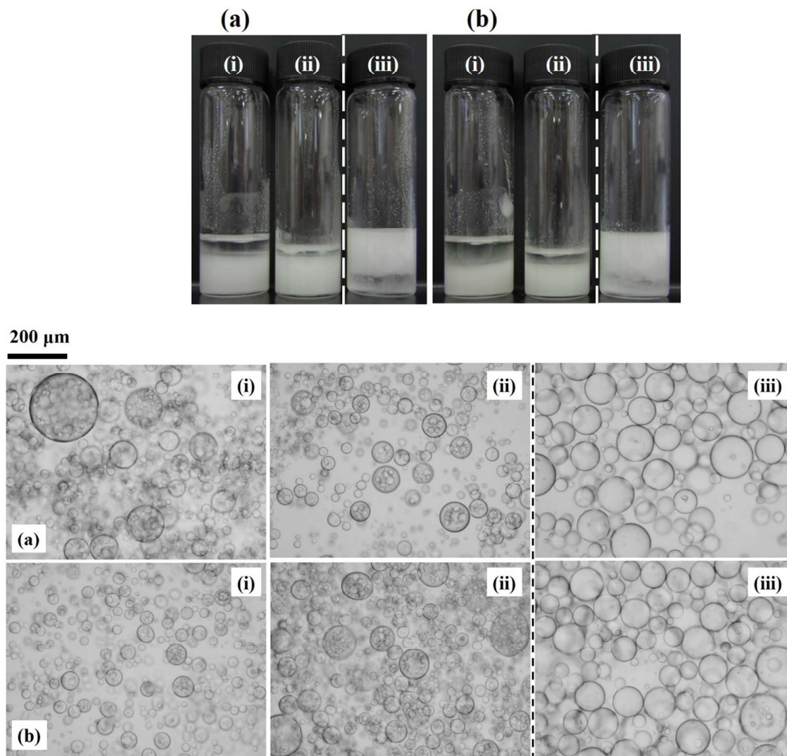
Figure 7. (upper) Photographs after 1 month of (a) sunflower oil-in-50 cS PDMS-in-sunflower oil and (b) olive oil-in-50 cS PDMS-in-olive oil multiple emulsions containing a volume fraction of initial V/S emulsion of (i) 0.3 and (ii) 0.7 prepared using low shear; (iii) simple V/S emulsions containing the vegetable oils and 50 cS PDMS after attempting to prepare S/V/S multiple emulsions with low shear. (lower) Corresponding optical micrographs of the emulsions.
