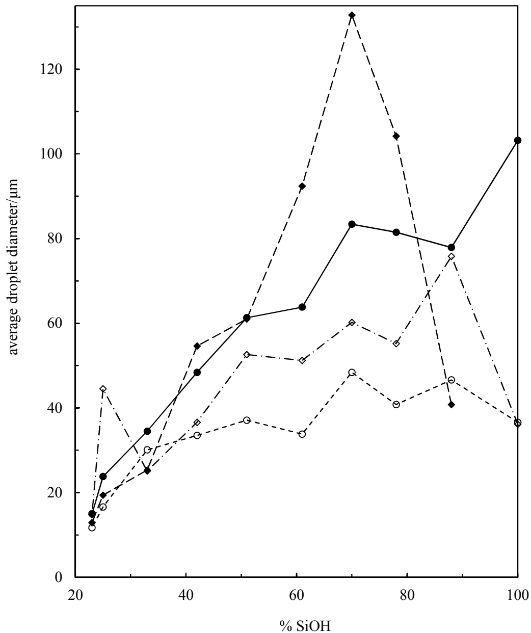
Figure 6. Plot of average droplet diameter of 50 cS PDMS-in-sunflower oil (●), 100 cS PDMS-in-sunflower oil (○), 50 cS PDMS-in-olive oil (◆) and 100 cS PDMS-in-olive oil (◇) emulsions after 1 month versus % SiOH on DCDMS-coated fumed silica particle surfaces. Standard deviation is in the range of 30 \mu\text{m} at relatively high % SiOH and 10 \mu\text{m} at relatively low % SiOH.
