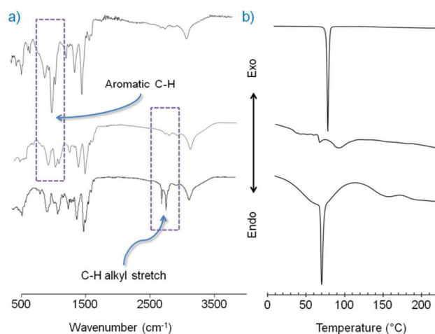
Fig. 1: a) FTIR spectra of poly(O-benzyl-L-serine), top , PS, middle and PSSA, bottom . b) Comparison of the DSC thermograms of octadecanoic acid, top , PS, middle and PSSA, bottom . The successful grafting of octadecanoic acid to PS is evidenced by the emergence of the melting point endotherm at 71.5 °C. on the thermogram of PSSA. (Endo = endotherm, Exo = exotherm).
