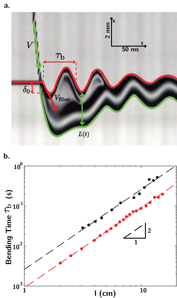
Fig. 5 Impact on a flexible fiber. (a) Kymograph for the impact of a viscous drop ( \eta = 100 cst) of speed V on a fiber of radius a = 127 \mu m and length l = 5 cm. The fiber starts oscillating with a typical timescale \tau_b , amplitude \delta_0 and initial velocity V_{fiber} . (b) Variation of the typical bending timescale \tau_b with fiber length l . We find \tau_b \sim l^2 , as expected on the basis of Eq. (1). Black points: impacts for Oh \ll 1 , with a = 63.5 \mu m and a fiber tip of 250 \mu m. Red points: impacts for Oh > 1 , with a = 127 \mu m.
