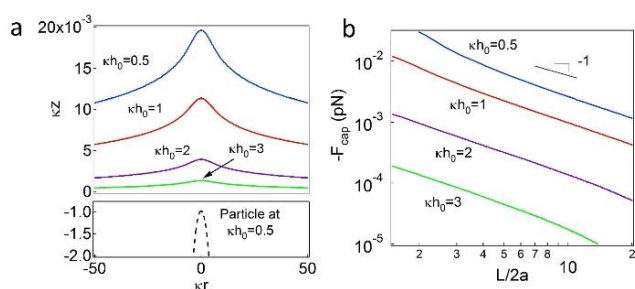
Fig. 4 (a) Dimensionless interface profiles obtained by solving the augmented Young-Laplace equation (Eqs. 6 and 10). The solid lines represent the curved interfaces with various initial heights of the interface \kappa h_0 . The dashed line represents the particle surface at \kappa h_0 = 0.5 . (b) Lateral capillary forces F_{cap} between two particles.
