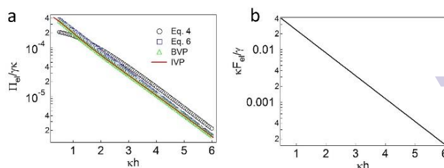
Fig. 3 (a) Comparison of disjoining pressure between two identically charged planes (i.e., \psi_{PW} = \psi_{DW} = -80 \text{ mV} ) obtained using Eq. 4, Eq. 6, BVP, and IVP. (b) Nondimensionalized double-layer interaction force between a spherical particle and a planar interface (i.e., \psi_{PW} = \psi_{DW} = -80 \text{ mV} ), as obtained from Eq. 8.
