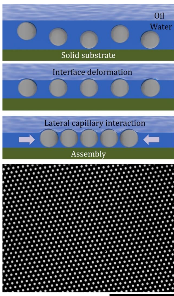
Fig. 1 Schematic of the self-assembled colloidal crystal via fluid interface templating. The bottom image is a snapshot of a 2D colloidal crystal extracted from movie 1 in SI. The scale bar is 30 \mu\text{m} .
