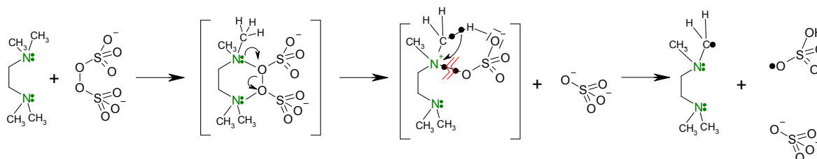
Scheme 1. Mechanism of the primary radical formation in the redox initiation by APS and TEMED. 26
