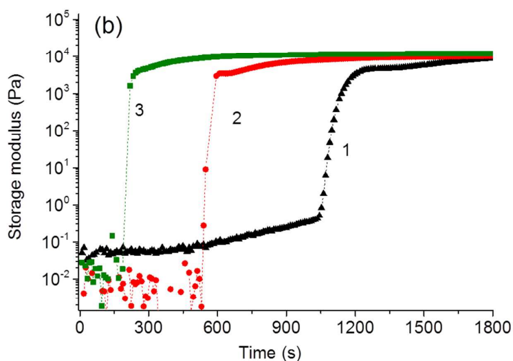
Fig. 8 Evolution of storage modulus G'(t) during polymerization of the system NIPA-clay at 25 °C, [NIPA]=0.75 mol/l
