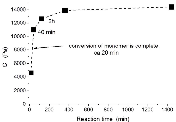
Fig. 10 Evolution of the modulus in the postgel stage during polymerization of the system 60X, content of initiators [\text{APS}]_f=0.0087 , [\text{TEMED}]_f=0.028 ( T=25 °C).
