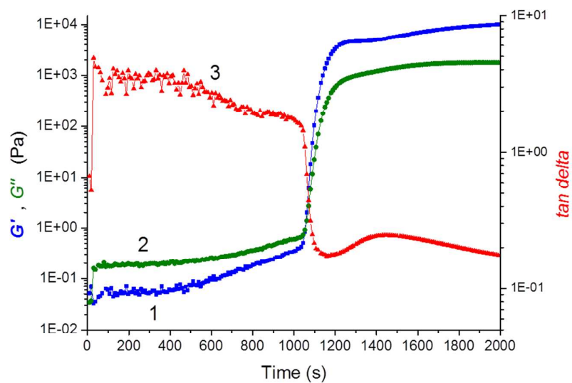
Fig. 7 Evolution of complex moduli G'(t) , G''(t) and loss factor \tan \delta during polymerization of the system 60X-0.01-0.0087; 1-(blue ■) Storage modulus, 2-(green ●) Loss modulus, 3-(red ▲) loss factor \tan \delta .
