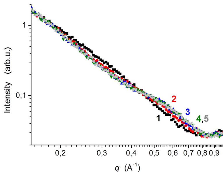
Fig. 11 SAXS profiles during polymerization of PNIPA-clay at 25°C, (60X-0.028-0.0043). The curves are indicated according to the reaction time; 1-(■) 10 min, 2-(●) 20 min, 3-(▲) 30 min, 4-(▼) 40 min, 5-(◄) 100 min.
