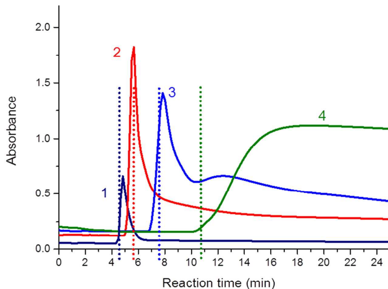
Fig. 12 Evolution of absorbance at 600 nm measured by UV-VIS spectrometry during polymerization of the PNIPA-clay system at 25°C, [APS]_r=0.0087 , [TEMED]_r=0.028 ; curves: 1- 20X, 2- 30X, 3- 40X, 4- 60X. Dashed lines show the gelation point.
