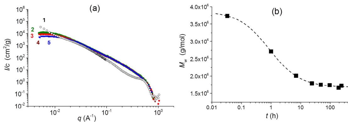
Fig. 1 (a) Evolution of SAXS profiles during mixing of clay suspensions; sample 30X curves (1;○)- dry, t(\text{mixing})=0 (2; ■) – 2 min, (3; ●)- 1h, (4; ▲) – 24 h, (5; ◆)- 48 h
