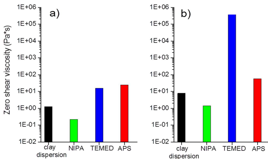
Fig. 3 Effect of reaction components on the viscosity of clay dispersions for different clay contents, mixing time = 1 h: a) 30X, b) 60X
