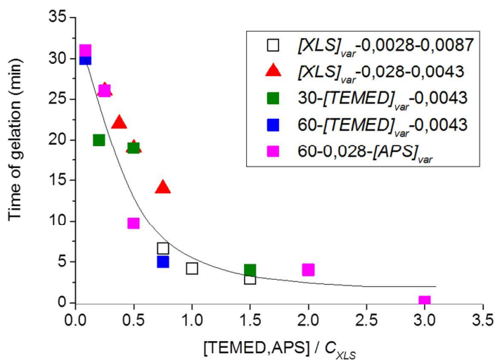
Fig. 9 Gel time as a function of the ratio of concentrations [\text{TEMED-APS}]/C_{XLS} corresponding to the theoretical functionality of the platelet.
