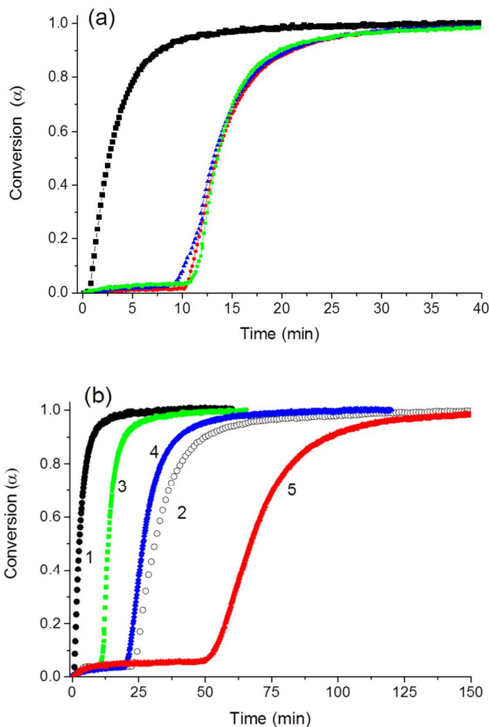
Fig. 5 Kinetics of NIPA conversion during polymerization in the systems with a different content of clay and initiators, T=25^\circ\text{C}
