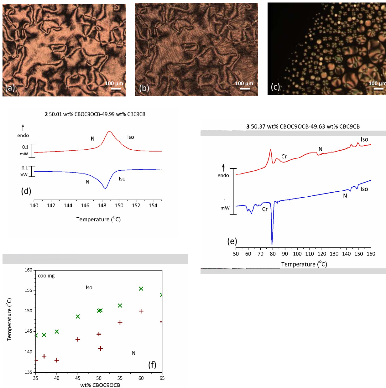
Figure 5: Optical textures on untreated glasses under crossed polarizers for mixtures in the range of 50-50 wt% a) N_x phase at 108.4 °C on cooling, b) N_x phase at 92 °C on cooling, c) biphasic region during the Iso-N transition d) segment of the DSC trace (3 °C/min) of mixture 2 where the N-Iso and Iso-N transitions are detected by a single peak (second heating/cooling runs), e) DSC thermogram (3 °C/min) for the second heating/cooling runs of mixture 3 where the N-Iso and Iso-N transitions split into two peaks, f) POM temperature transition data for the biphasic region
