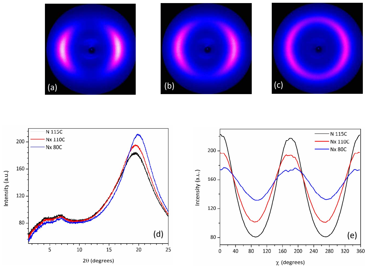
Figure 8: Two dimensional diffraction patterns of CBC9CB a)N at 115 °C, b)N x at 110 °C, c)N x at 80 °C, d) \theta -scan of the diffraction patterns in the N and N x phases, e)distribution of the wide angle scattering along \chi (15°-25° 2\theta )
