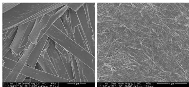
Figure 2 SEM micrographs of ethanol xerogels (a) large, flat ribbons of compound 1d typical of type 1 , (b) narrow cylindrical fibres of 2b typical of compounds of type 2 .
