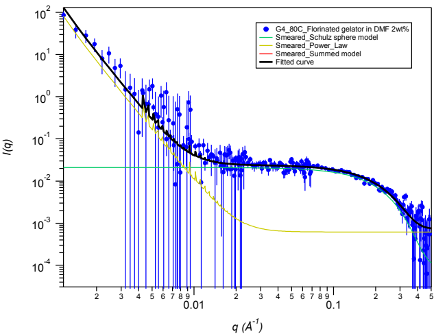
Figure 6. SANS Smeared summed model (red line beneath black fitted curve line) of Porod_low fit and Schulz sphere fit for the fluorinated bis-urea gelator 2a in DMF at 2 wt%, measured at 80 °C, showing breaking of the gel structure.
