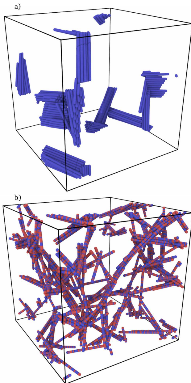
Fig. 2 a) Typical uniform (non-patchy), low corrugation ( a = 0.4\sigma ) configuration at long time. b) Typical patchy (50% functionalized surface) low corrugation ( a = 0.4\sigma ) configuration at long time. The uniform system forms disconnected clusters with fluid-like dynamics. The patchy system forms a rigid, spanning network with finite shear modulus and yield stress. Rods which are uniform but with stronger corrugation ( a = \sigma ) not shown) may also form rigid, spanning structures with solid-like dynamics.
