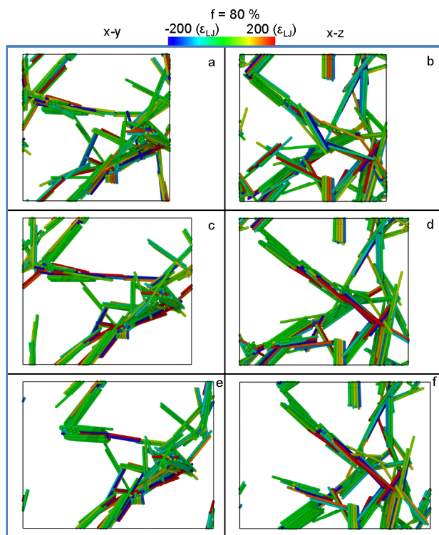
Fig. 12 The same as Figure 11, but for f = 80\% .
