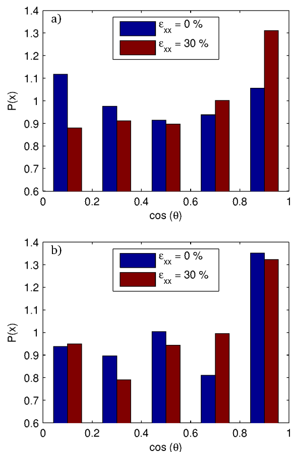
Fig. 13 Distribution of orientation x = \cos(\theta_x) at a strain of 0% and 30% for the systems with surface fraction a) 20% and b) 80%. \cos(\theta_x) is the cosine of the angle the rod makes with extensional axis.
