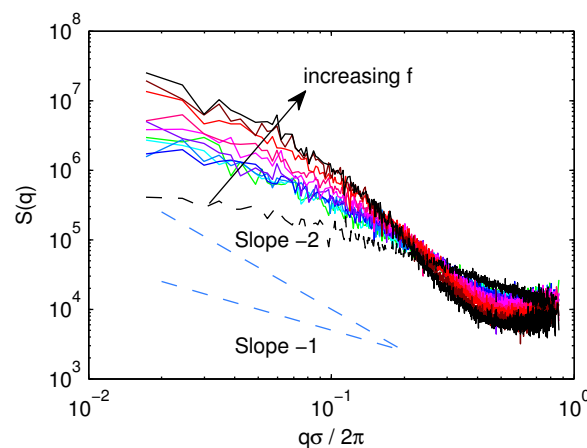
Fig. 4 Structure factor, S(q) , for rod networks at various f for t_w = 5 \times 10^4 \tau .
