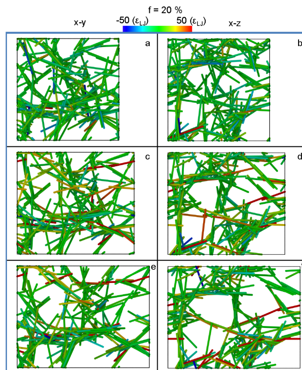
Fig. 11 Orthographic projection in the xy and xz planes of : a-b) unstrained, c-d) 15% and e-f) 30% strained configuration for f = 20\% . The extension axis, x , is horizontal. Rods are colored according to their contribution to the total Virial in the stretching direction, \Sigma_{xx} . Red indicates tensile and blue compressive stresses.
