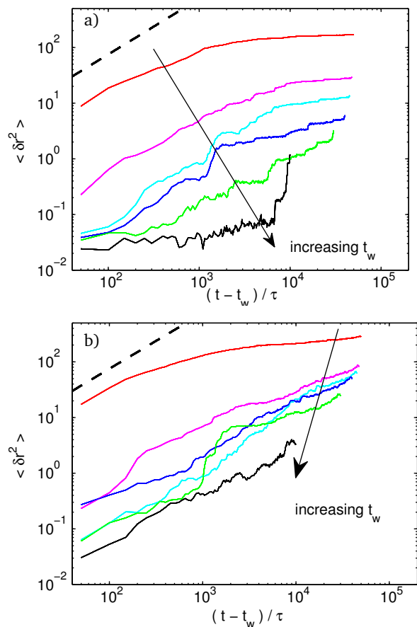
Fig. 7 The same as Figure 6 for f = a) 80%, b) 90%.
