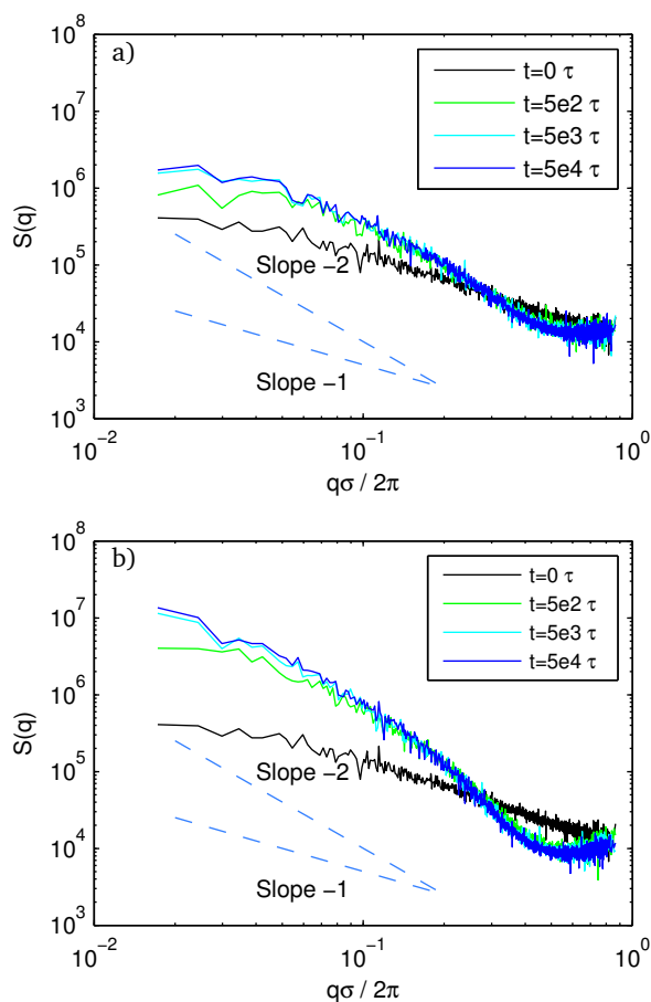
Fig. 3 Structure factor, S(q) , for rod networks at various waiting time: t = 0 (black), 5 \times 10^2 \tau (green), 5 \times 10^3 \tau (cyan), 5 \times 10^4 \tau (blue). Fraction, f , of attractive sites: a) 40%, b) 80%. The blue dashed lines are S \sim q^{-1} and S \sim q^{-2} for reference.
