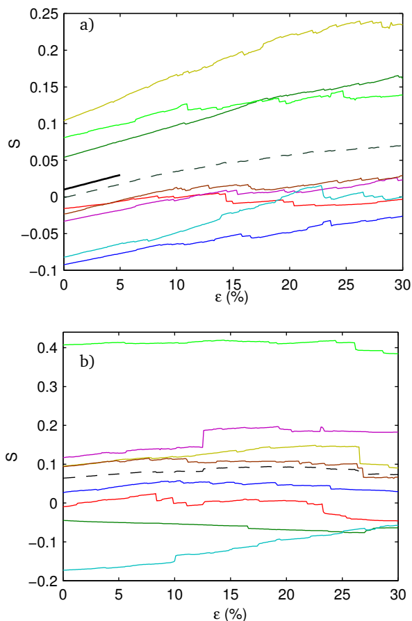
Fig. 14 Nematic order parameter, S , as a function of \epsilon , for the systems with surface fraction a) 20% and b) 80%. The black solid line shows the slope of Nematic order parameter versus \epsilon for rods deforming affinely with the extension flow.
