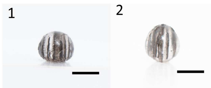
Figure 4. Photographs of the resulting particles polymerized with a magnet above and below the droplet in the attractive regime. The bottom distance is fixed as 2 cm and both particles are synthesized at center (place I) (5,5). Top distance for (1) is 5 cm and for (2) is 3.5 cm. All scale bars in the pictures are 1mm.
