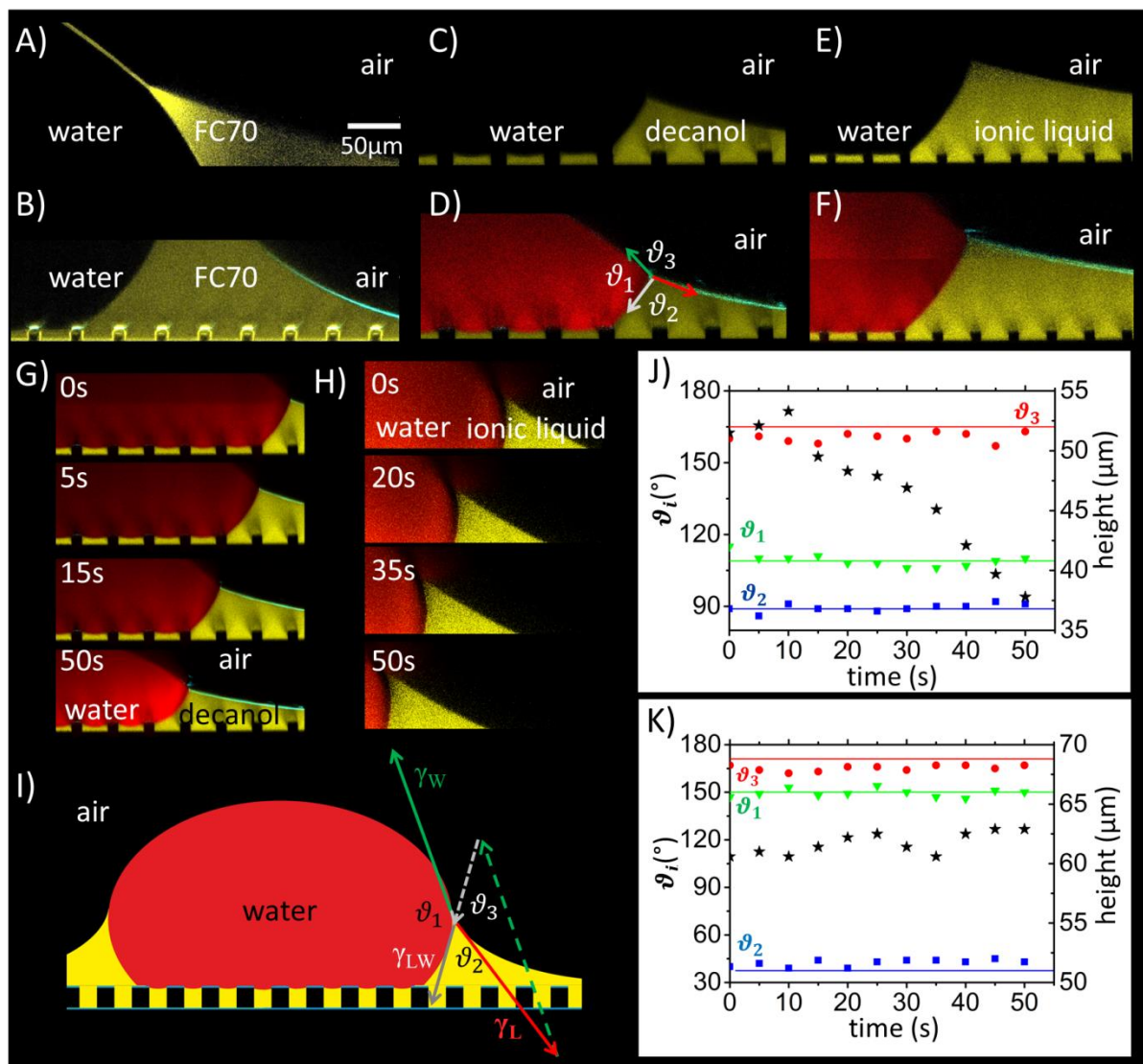
Figure 4. Cloaking of drops or a liquid-three phase contact line. A-B) Confocal images of vertical sections through a water drop placed on lubricant-impregnated micropillar arrays (black rectangles). FC70, decanol and ionic liquid were used as lubricants. A, B) Fluorescence signals (yellow) of FC70 and the reflection of light from the lubricant–air interface (cyan). C, D) Fluorescence signals (yellow) of decanol. The combined image (D) shows the fluorescence signal of the lubricant, the water drop (red) and reflection of light (cyan). E, F) Fluorescence signals (yellow) of ionic liquid. The combined image (F) shows the fluorescence signal of the lubricant, the water drop (red) and reflection of light (cyan). G,H) Time series of an evaporating water drop on (G) a decanol and (H) an ionic liquid lubricated micropillar array.
