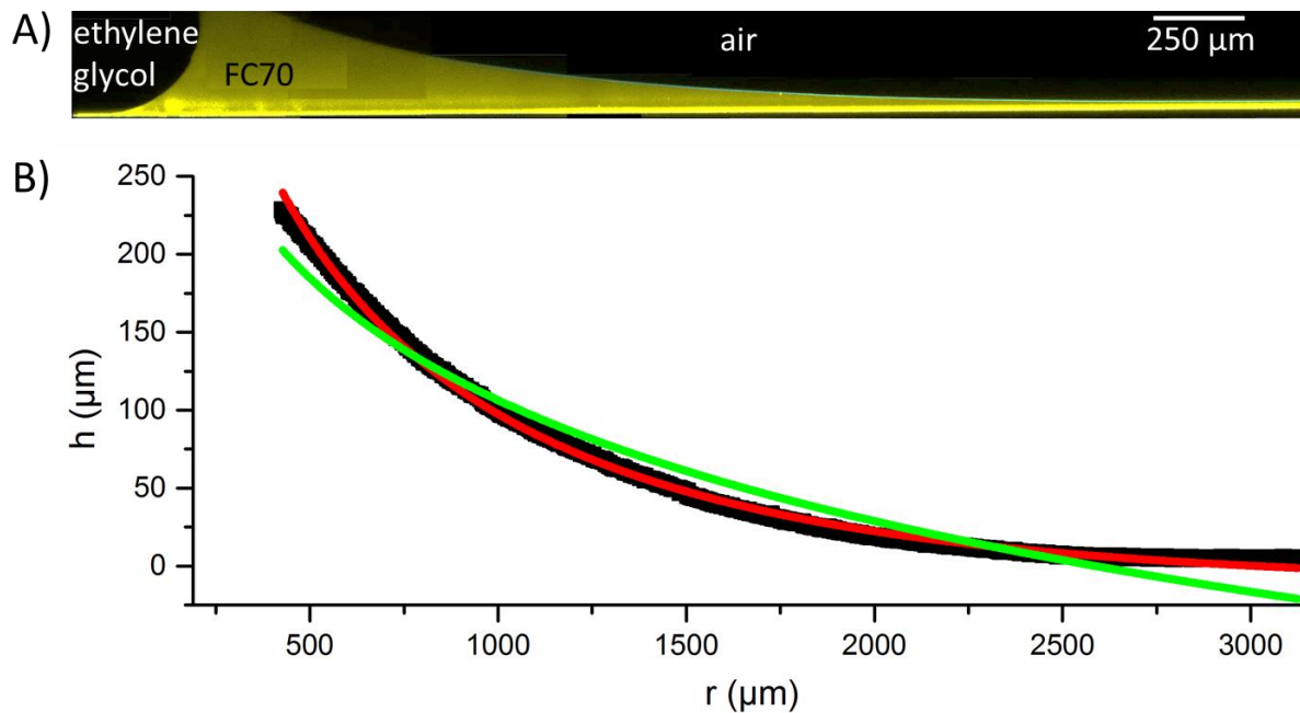
Figure 5. Shape of the wetting ridge. A) Extent of the wetting ridge of the FC70 (yellow) which formed after an ethylene glycol drop (black) was deposited on an inverse opal infiltrated with FC70. To span the full, wide range of the wetting ridge (approximately 3 mm, Fig. 5B), various images were combined (each image covered a width of merely 400 μm). B) Meniscus of FC70 around an ethylene glycol drop on an inverse opal fitted with different models. Red: catenoid; Green: nodoid, C_0 \neq 0 , with fixed pressure P . The experimental data for the height of the wetting ridge z(r) is shown as a function of the distance from the drop center r (black squares). h = 0 corresponds to the top face of the pillars.
