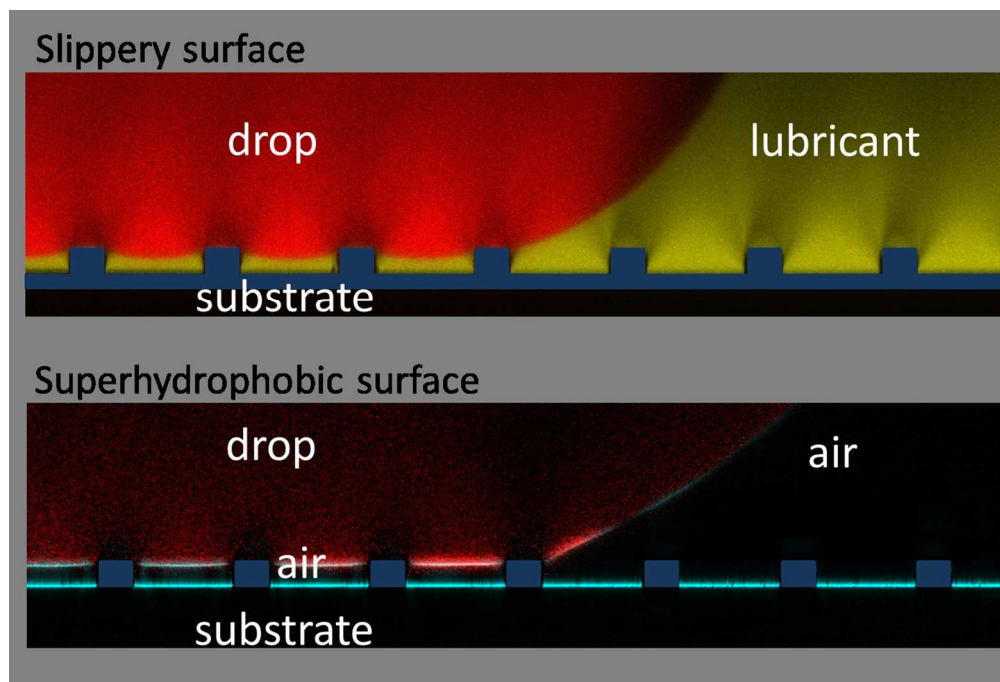
Slippery compared to superhydrophobic surface.
