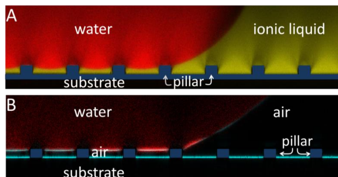
Figure 9. Slippery compared to superhydrophobic surface. Comparison of a water droplet (red) deposited on (A) a slippery ionic liquid (yellow) infused micropillar array, (B) a superhydrophobic surface. Air, glass substrate and the micropillar arrays appear black. On a slippery micropillar array the drop rests on the pillars' top faces and the region between the micropillars is filled with lubricant. On the super-hydrophobic surface the interpillar space is filled with air. Image size: 291.6 \times 71.7 \mu\text{m}^2 .
