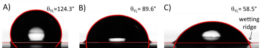
Figure 3. Drops deposited on a lubricant-infused textured surface. A) Water, B) ethylene glycol, and C) hexadecane drops were placed on inverse opals infiltrated with FC70. The circular red line represents a fit of the drop contour to the Young–Laplace equation. The angles were obtained by fitting the contour of the drop using a Young-Laplace fit. The volume of each drop was 3 \mu\text{L} .
