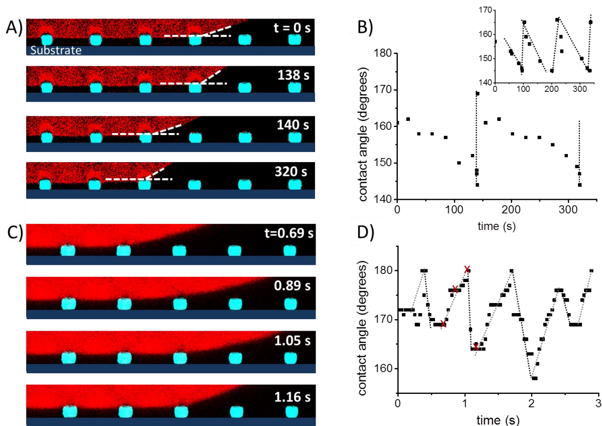
Figure 8. Receding and advancing contact angles at the solid-TPCL. A) Confocal microscopy images monitoring the contact angle of a water drop (red) as it recedes because of evaporation on an FC70-impregnated micropillar array (blue). The FC70 was not dyed. B) The contact angle continuously decreased until it approached the receding contact angle, \theta_{r,app} = 144^\circ \pm 1^\circ . Inset: Variation in \theta_{app} for a water drop on a micropillar array impregnated with the ionic liquid. C) Confocal microscopy images monitoring the advancement of a drop on an FC70-impregnated micropillar array. Advancement was induced by applying air flow. D) Variation in \theta_{app} as the drop advanced. The contact angle continuously increased until it reached 180^\circ and subsequently abruptly decreased to a lower value. The crosses correspond to the images shown in C. The receding ( v_{rec} = 0.18 \pm 0.05 \mu\text{m/s} ) and advancing ( v_{adv} = 60.5 \pm 6.5 \mu\text{m/s} ) velocities were averaged over the time required to recede/advance over three pillars.
