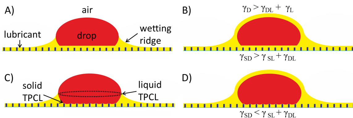
Figure 1. Wetting configurations. Schematic illustrations of possible wetting configurations of a slippery lubricant-infused textured surface. A, C) The drop (red) resting on a micropillar array (blue) is surrounded by an annular wetting ridge that may end in a pulled-up liquid three phase contact line (liquid-TPCL). The lubricant (yellow) does not cloak (A, C) or it may cloak (B, D) the drop. Drops on slippery surfaces can exhibit zero, one, or two three-phase contact lines. The liquid-TPLC is the line at which the air, drop, and lubricant meet, and the solid-TPCL is where the substrate, drop, and lubricant meet. The interfacial tensions \gamma_{ij} are denoted as follows: \gamma_{DL} - interfacial tension between the drop and the lubricant; \gamma_{SD} - interfacial tension between the surface and the drop; \gamma_{SL} - interfacial tension between the surface and the lubricant. \gamma_D represents the surface tension drop-air and \gamma_L the surface tension lubricant-air.
