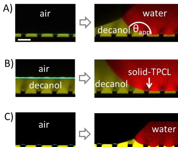
Figure 6. Influence of the filling height. Image of a micropillar array infiltrated with decanol before (left) and after (right) a water drop was deposited. (A) The height of the lubricant film was adjusted to the height of the micropillar array. (B) The micropillar array was overfilled with lubricant (left) before the water drop was deposited (right). (C) The micropillar array was underfilled before the drop was deposited. The height of overfilling or underfilling was measured relative to the height of the pillar's top face ( h = 0 \mu\text{m} ). Colour code: water drop - red or black; lubricant - yellow; reflected light - cyan; air - black. Diameter of a pillar: 10 \mu\text{m} ; height of pillar: 10 \mu\text{m} ; centre to centre distance: 40 \mu\text{m} .
