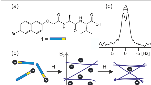
Scheme 1. a) Structure of gelator 1 . b) Cartoon to illustrate that upon a decrease in pH, molecules of 1 assemble to form fibres which bear a significant negative charge ( vide infra ). Upon further decreases in pH, these lose charge and bundle together. The presence of the magnetic field, B_0 , induces significant anisotropy in the orientations of the fibres leading to the observation of residual quadrupolar couplings (RQCs), \Delta , on the ^1\text{H} and ^{15}\text{N} NMR resonances of probe molecules (c).
