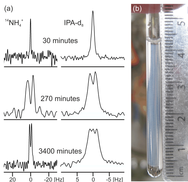
Figure 2. a) Experimental ^{14}\text{N} and ^2\text{H} NMR spectra of sample from Figure 1a at different times since addition of GdL to a solution of the gelator at high pH. The spectra have been scaled to account for the different number of transients recorded at different stages of gelation. b) Photograph of the gel sample of Figure 1a, 4000 minutes after GdL addition. The transparent exuded fluid is apparent above and below the slightly translucent gel. The NMR active region of the sample is centred at 18 mm from the base of the tube and stretches 8 mm either side.
