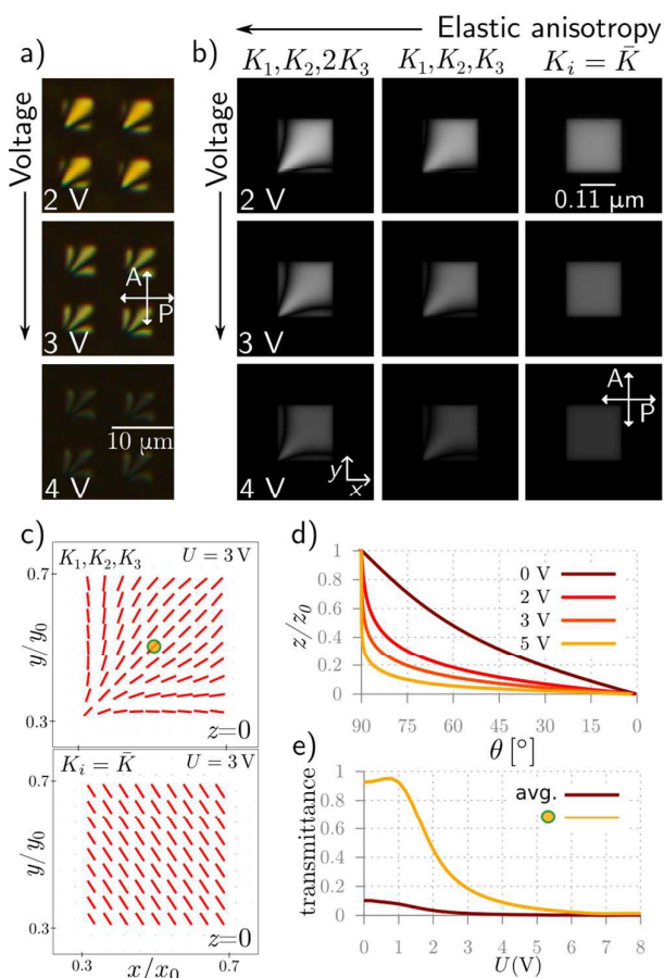
Fig. 2 Electric-field tunability of birefringence. a) Experimental optical microscopy images viewed in white light transmission between crossed polarizers as a function of the applied voltage. b) Simulated optical microscopy images as a function of the applied voltage and the elastic anisotropy. On the vertical axis the electric field is increased from 2 to 4 V, while on the horizontal axis the elastic constants of the simulated LC have been changed. Left column K_1=12.1 pN, K_2=5.9 pN, 2K_3=47.4 pN. Central column K_1=12.1 pN, K_2=5.9 pN, K_3=23.7 pN. Right column K_1=K_2=K_3=K_{av}=13.9 pN. c) Director field at z=0 and U=3V in elastically anisotropic ( K_1, K_2, K_3 ) regime shows modulations in the lateral directions, compared to the uniform response in the elastically isotropic ( K_i = \bar{K} ) regime. d) The director tilt angle \theta across the center-point of the patterned cell (marked by a circle in Fig. 2c) as a function of four applied voltages. e) Simulated transmittance as a function of the applied field at the center point in Fig. 2c (yellow line) and as an average over all the square in Fig 2c (brown line). Under strong electric fields the average tilt angle increases causing a significant drop of transmittance.
