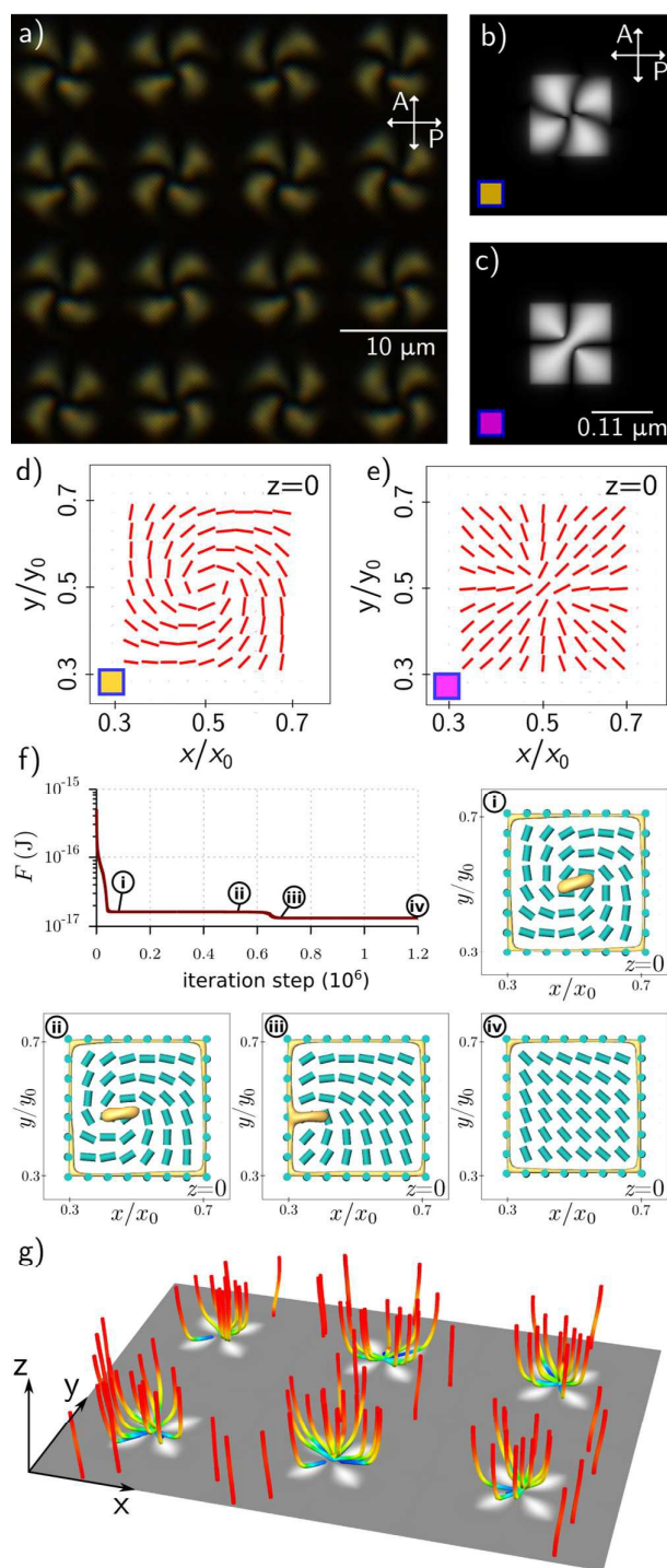
Fig. 3 Complex Skymion-like birefringent phases stabilized by surface patterns. a) Experimental optical microscopy image viewed in white light transmission between crossed polarizers after the application of a potential of 30 V. b) and c) are simulated optical microscopy images for two defect states with the lowest free energy; d) and e) are the corresponding director fields at the patterned surface ( z=0 ). f) Free energy relaxation process of a Skymion state with insets showing the director field (cyan cylinders) and scalar order parameter (yellow isosurfaces at S=0.5 ). Panels (i-iv) show: i) formation of a boojum surface defect from the initial conditions, ii) drift of a boojum defect towards the
