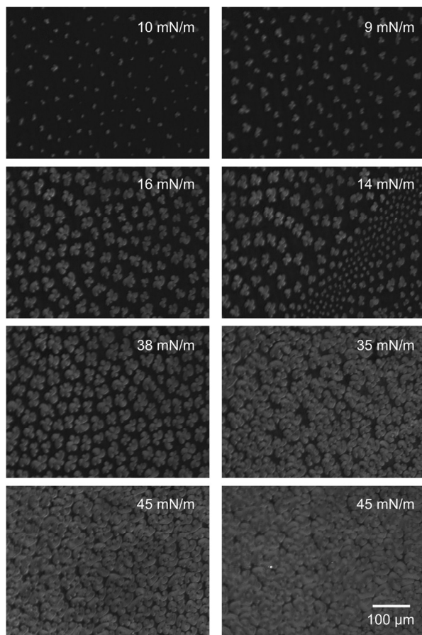
Figure 5. Brewster angle microscopy images of DPPC monolayers at the liquid air interface on salt solutions. Left: sodium chloride ([NaCl]= 155 mM). Right: sodium chloride ( [NaCl]= 155 mM) with calcium chloride ( [CaCl 2 ]= 10 mM).
