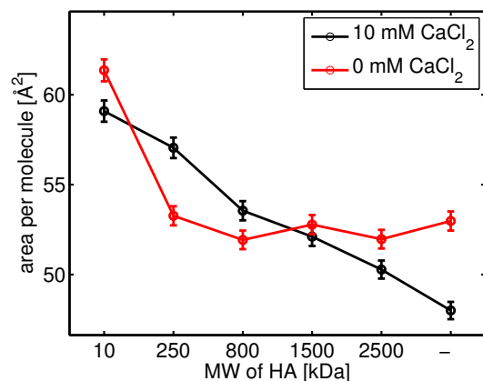
Figure 3. Area per molecule for DPPC on different subphases at a constant surface pressure of 40 mN/m.
