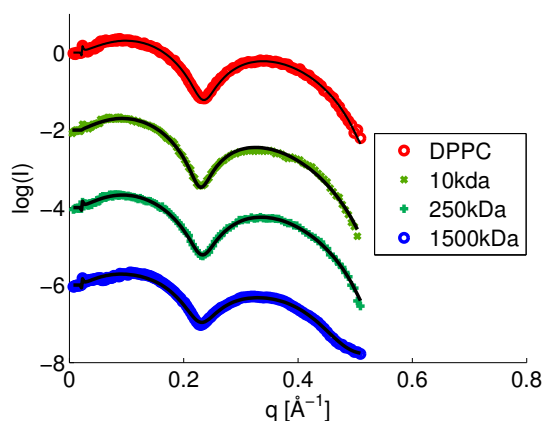
Figure 8. XRR curves of DPPC Langmuir layers on top of different solutions containing 155 mM NaCl in absence and presence of HA with different molecular weight. The curves were measured at an area per molecule of 55 \text{ \AA}^2 , and they are vertically shifted for clarity. The solid lines represent fits to the data.
