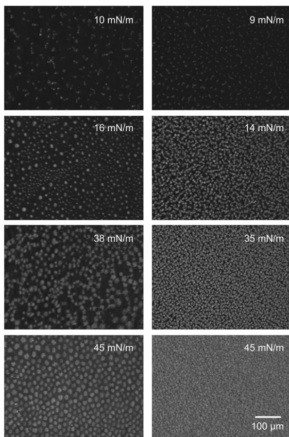
Figure 6. Brewster angle microscopy images of DPPC monolayers at the liquid air interface on salt solutions with HA with a MW of 10 kDa. Left: sodium chloride ( [NaCl]= 155 mM). Right: sodium chloride ([NaCl]= 155 mmol/L) with calcium chloride ([CaCl 2 ]= 10 mM).
