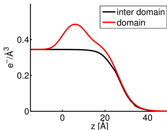
Figure 10. Electron density profiles of DPPC on solutions containing HA with MW 10 kDa. An incoherent model was used to evaluate the data where the domain structures represent the condensed DPPC patches and the inter domain region corresponds to the area in between these patches.
