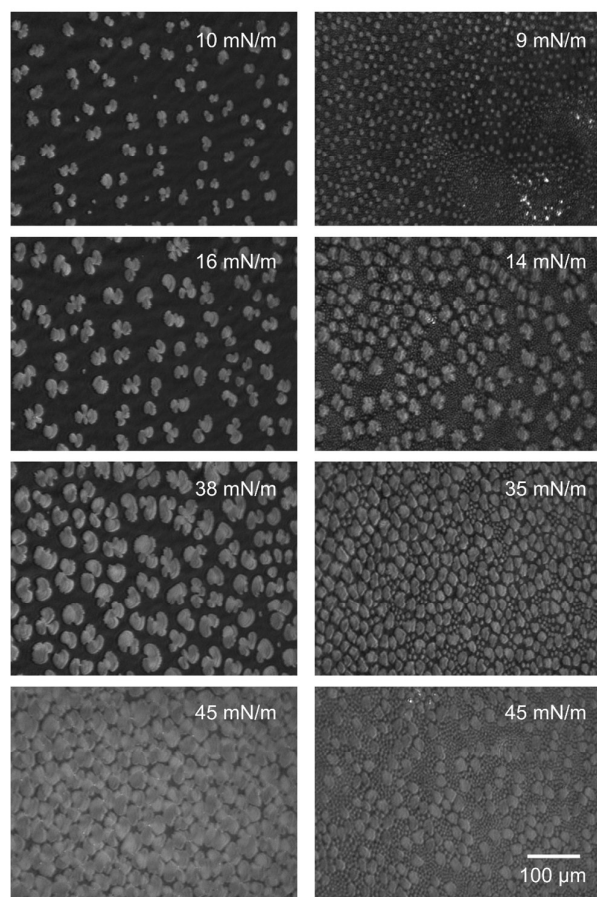
Figure 7. Brewster Angle Microscopy images of DPPC monolayers at the liquid air interface on salt solutions containing 0.5 mg/mL HA with a MW of 1500 kDa. Left: sodium chloride ( [\text{NaCl}] = 155 \text{ mM} ). Right: sodium chloride ( [\text{NaCl}] = 155 \text{ mM} ) with calcium chloride ( [\text{CaCl}_2] = 10 \text{ mM} ).
