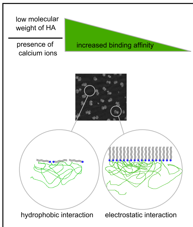
Figure 11. Scheme of the interaction of HA with DPPC at the water-air interface
