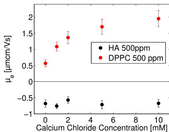
Figure 4. Electrophoretic mobility of DPPC vesicles and HA as a function of [\text{CaCl}_2] at 25°C.
