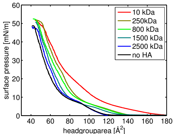
Figure 2. \Pi/A -isotherms of DPPC on subphases containing sodium and calcium chloride ( [\text{NaCl}] = 155 \text{ mM} , [\text{CaCl}_2] = 10 \text{ mM} ). The concentration of HA was 0.5 \text{ mg/mL} .
