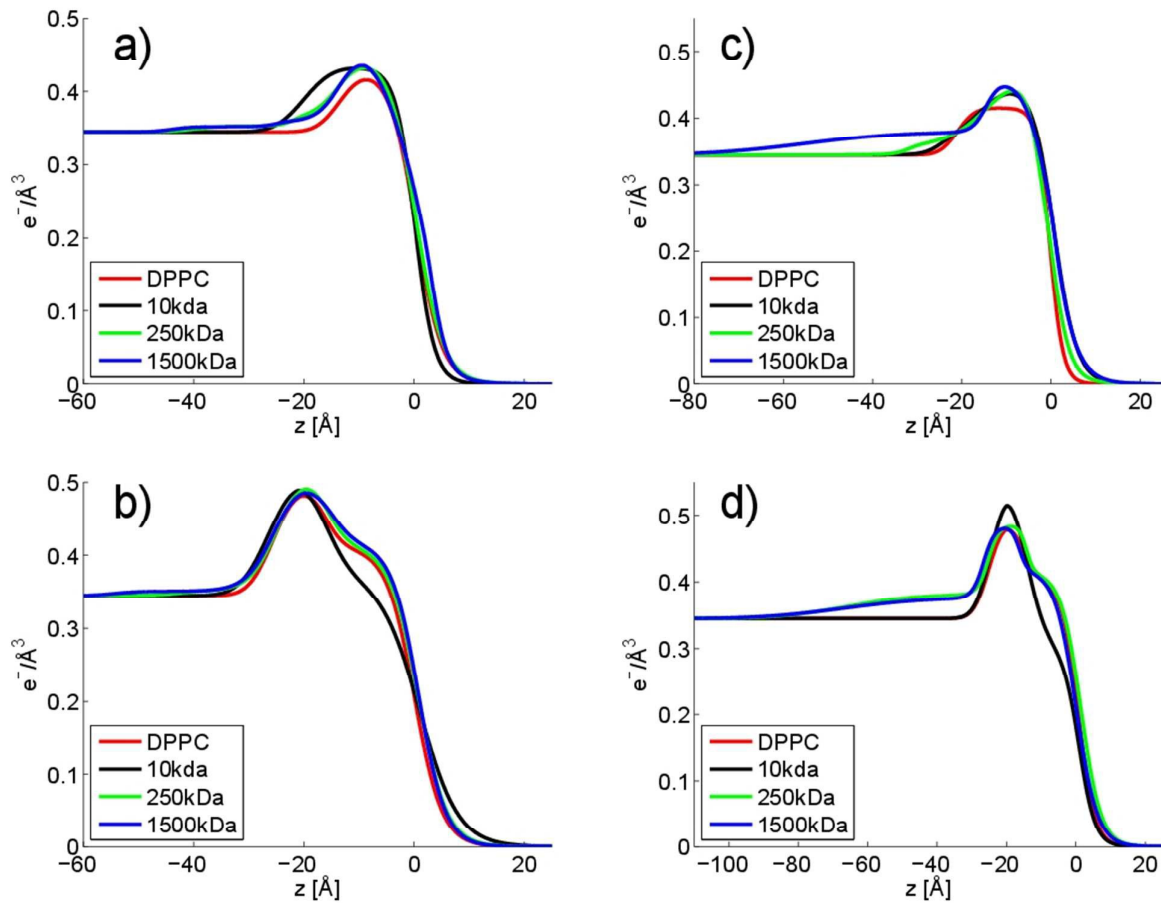
Figure 9. Electron density profiles of DPPC Langmuir layers on different subphases and at different areas per molecule. a) Area/molecule = 120 Å 2 , [NaCl] = 155 mM. b) A = 55 Å 2 , [NaCl] = 155 mM. c) Area/molecule = 120 Å 2 , [NaCl] = 155 mM, [CaCl 2 ] = 10 mM. d) A = 55 Å 2 [NaCl] = 155 mM, [CaCl 2 ] = 10 mM.
