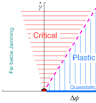
Fig. 6 Regimes in the (\Delta\phi, \dot{\gamma}) plane based on our scaling results for the moments of \Gamma . Our data indicates a crossover, at \dot{\gamma} \sim \Delta\phi^\beta for \beta \approx 1 (purple, dashed) which separates the critical and plastic regime as indicated. The quasistatic regime can smoothly be reached from the plastic regime. Our data clearly evidences critical behavior for \Delta\phi < 0 at finite flow rate, although the nature and location of the crossover to the deeply unjammed regime is unclear. Note that while the jamming point (red dot) plays a crucial role in organizing the physics, the line \Delta\phi = 0 has no particular significance for \dot{\gamma} > 0 .
