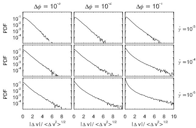
Fig. 2 The shape of the probability density function of the normalized velocity differences, |\Delta v|/\langle\Delta v^2\rangle^{1/2} , varies strongly with packing fractions and strain rates as indicated. In this representation, a Gaussian appears parabolic and an exponential becomes a straight line.
