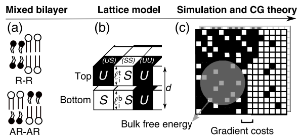
FIG. 2. (a) Mixed bilayer containing S and U ( L_o or L_d -like) model species, illustrating the locally symmetric (R-R) and locally asymmetric (AR-AR) phase coexistences considered here. (b) Microscopic lattice model for coupled leaflets, which can be coarse-grained (CG) (c) to give the mean-field free-energy density f(\phi^t, \phi^b) as a function of locally-averaged leaflet compositions, and analysed for kinetics of domain formation with the inclusion of gradient costs for domain boundaries [1]. The lattice model can also be directly simulated.
