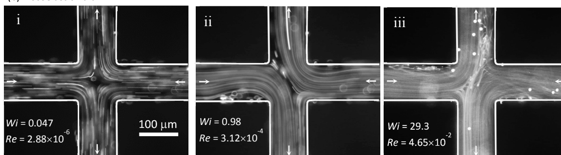
Fig. 3 Flow patterns in the cross-slot geometry with AR = 1.0 . (a) Newtonian fluid flow. (b) PAA300+50%Glyc viscoelastic fluid: (i) Newtonian-like symmetric flow behaviour, (ii) steady asymmetric flow, (iii) time-dependent flow (illustrative flow field at a given instant of the oscillation cycle).
