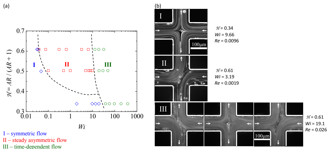
Fig. 4 (a) Flow pattern map. (b) The images obtained using the PAA300+50%Glyc fluid ( \beta = 0.0022 ) illustrate the flow patterns in the three regions of the map. From top to bottom: (I) Newtonian-like or symmetric flow; (II) steady asymmetric flow; (III) time-dependent flow (three instants are shown). The dashed lines in the flow pattern map are simply a guide to the eye of the expected separation between the three types of flow. The Reynolds number varies in the following ranges: 8.8 \times 10^{-4} \leq Re \leq 1.30 for H = 0.34 ; 2.9 \times 10^{-6} \leq Re \leq 9.36 \times 10^{-2} for H = 0.50 ; and 1.5 \times 10^{-6} \leq Re \leq 8.3 \times 10^{-2} for H = 0.61 .
