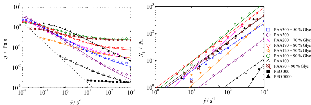
Fig. 2 Steady shear viscosity and first normal stress difference as function of shear rate. The symbols represent the experimental data, the solid lines the fits of the White-Metzner model and the dashed line represents 20\times the minimum measurable viscosity, which was calculated based on the minimum torque ( 0.1\ \mu\text{Nm} ) of the shear rheometer used.
