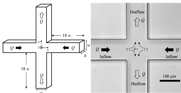
Fig. 1 The cross-slot geometry: (a) schematic representation showing the relevant variables and coordinate system and (b) bright field image showing the two inlets and two outlets. The stagnation point (S) is also represented.
