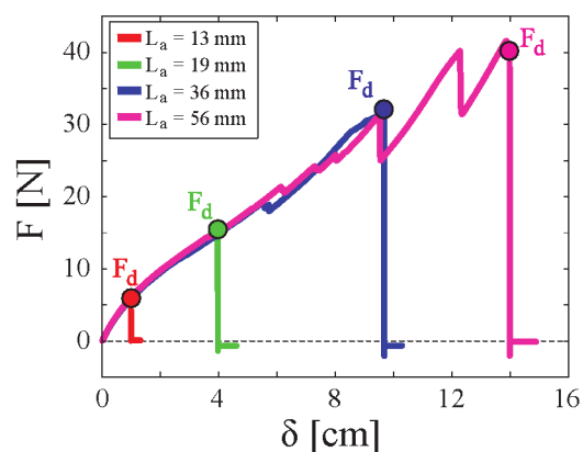
Fig. 4 Tensile force applied to the strip as a function of the imposed displacement. The material parameters for the strip are E = 529(\pm 2) kPa, L = 49 mm, w_o = 30 mm, h = 2.3 mm. The detachment force is marked for each experience with a point of the same color of the corresponding adhering length.
