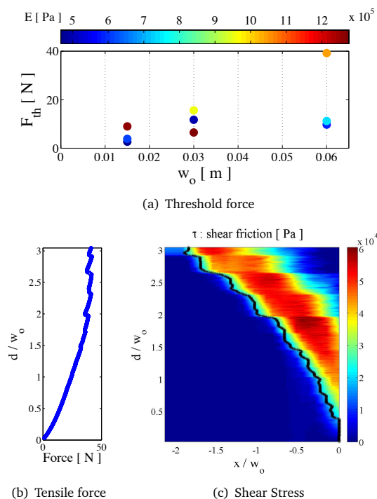
Fig. 11 (a) Threshold force as a function of the width of the strip. The colorbar represents the Young modulus of each sample in units of Pa. (b) Evolution of the tensile force as a function of the imposed displacement in an experiment displaying stick slip behavior (upwards). (c) Space-stress diagram quantifying the corresponding shear stress on a strip, the black line represents the sliding front position. Sample's parameters for diadrams (b) and (c): E = 1055 kPa, h = 2.2 mm and w_o = 30 mm.
