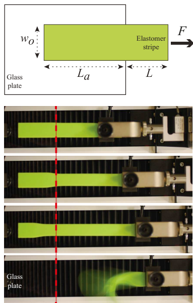
Fig. 1 Top: sketch of the experimental setup in an initial stage, i.e. before any deformation is applied (top view). A long strip of elastomer (in green) of width w_0 adheres on a glass plate along a length L_a . The pulling force F at the free end of the strip of length L at a constant speed v is monitored with a force displacement machine. Bottom: snapshots of an actual experiment. The free end is clamped between the moving jaws of the force displacement machine while the glass plate is fixed to the frame. In the last image, the strip has just detached.
