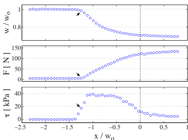
Fig. 8 Measurement of the local width and estimation of the corresponding force and shear stress acting on the strip at a given time (the applied displacement corresponds to d/w_0 = 2.33 in fig.9). In the x coordinate, zero corresponds to the edge of the glass plate, while positive coordinates represent the side of the strip that is away from the plate, i.e. zone 3. The arrows indicate the position of the sliding front x_F . This front is defined as the location where local width has decreased by 1% from its initial value. Experimental parameters are: E = 1055 kPa, h = 2.2 mm and w_0 = 60 mm.
