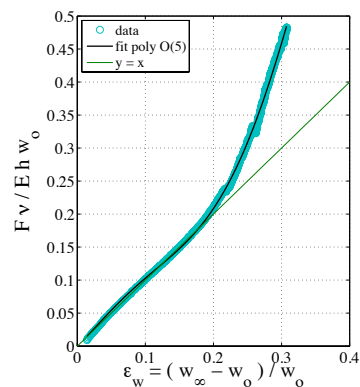
Fig. 7 Calibration curve of the force as a function of the width of the strip. The initial linear dependence provides the Young modulus of the material (in the current case, 1 MPa). The black solid curve corresponds to a 5 th order polynomial fit and the green solid line is the reference of a linear curve with unit slope.
