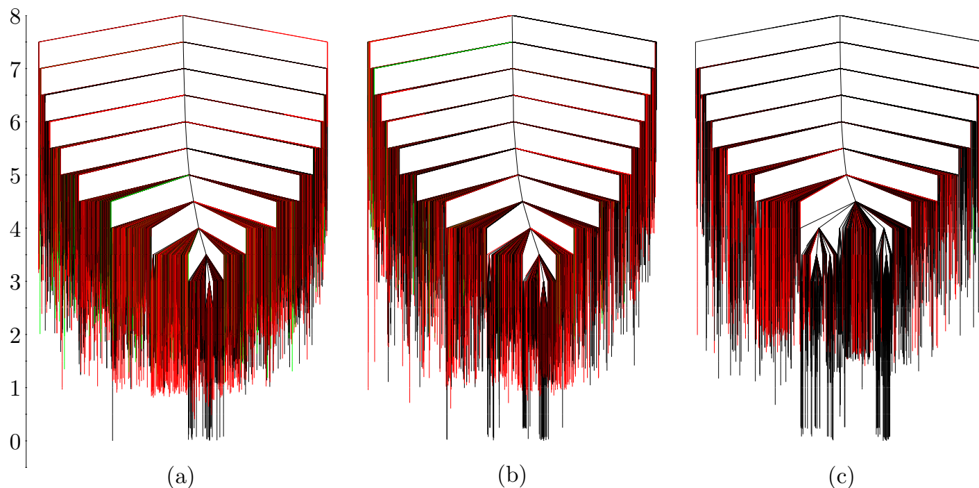
Fig. 4 Disconnectivity graph for N = 26 building blocks under different conditions: (a) no sedimentation ( \varepsilon^g = 0 ); (b) \varepsilon^g = 0.0165 ; (c) \varepsilon^g = 0.165 . Minima containing one, two and three tetrahedra are coloured red, green and blue, respectively. The number of minima containing tetrahedral configurations decreases drastically with increasing gravity effects: e.g. panel (a) contains 121 minima with two tetrahedra, panel (b) contains 42, while panel (c) contains only one such structure. Energies are displayed relative to that of the global minimum in each system. Only minima with at least three connections in the database are shown.
