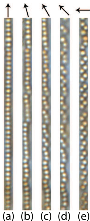
Fig. 6 Optical microscopy images of structure transformations of a colloidal single chain stretched from zigzag chain composed of superparamagnetic M-silica spheres with a diameter of 583 nm in magnetic field with different directions.
