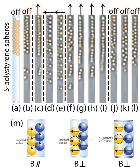
Fig. 7 Schematic image of zipper pattern (a) and optical microscopy images of structure transformations of zipper chain composed of S-polystyrene spheres with a diameter of 506 nm (the size ratio is around 1.75) from a attractive chain in a parallel field (c, f-i) to repulsive dimers in a perpendicular field (d-e) and back to original zipper chain after removal of the field (j-l). Illustration of dipole interactions in parallel and perpendicular fields (m).
