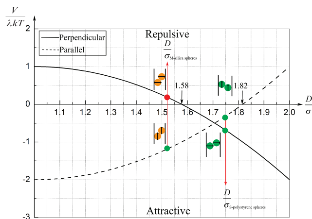
Fig. 14 Sketch of the magnetic contact interaction from eq. (5) and eq. (11); the interaction is zero at D/\sigma = 1.58 and 1.82 . In a perpendicular field (solid line), at larger D/\sigma , the spheres attract whereas below this zero point the spheres repel. In a parallel field (dashed line), at larger D/\sigma , the spheres repel whereas below this zero point the spheres attract.
