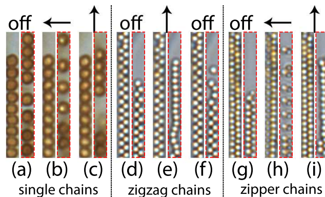
Fig. 11 Optical microscopy images of different magnetic response of single chains (a-c), zigzag chains (d-f) and zipper chains (g-i) with different volume fractions under either parallel field or perpendicular field.
