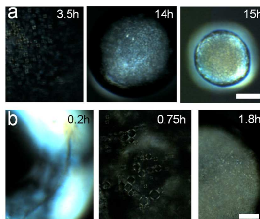
Fig. 4 The time evolution of liquid crystalline phase in shrinking CNC droplets. Reflection polarized microscopy images of a droplet in: (a) toluene/5 vol% ethanol (a) and (b) toluene/15 vol% ethanol, taken at different times during the shrinking process. The initial CNC concentration of the droplets was 0.3 vol%. Birefringent domains appear bright under cross polarized light. The scale bar is 100 \mu\text{m} .
