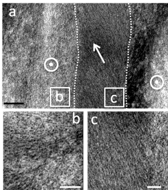
Fig. 8 The internal microstructure of a dried CNC microbead formed in toluene/1 vol% ethanol. The bead was ultramicrotome-sectioned through the centre of the particle and transmission electron microscopy reveals zones of different CNC rod orientation (separated by dotted lines) (a). The rods are aligned normal to the plane of the section (b) or in the plane (c). The circles in (a) indicate the normal orientation and the arrow the in-plane orientation. Scale bars are 100 nm (a) and 50 nm (b,c).
