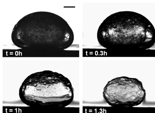
Fig. 5 Side view images of a shrinking CNC droplet with an initial volume of 10 \mu\text{L} in a toluene/10 vol% ethanol solution. The
