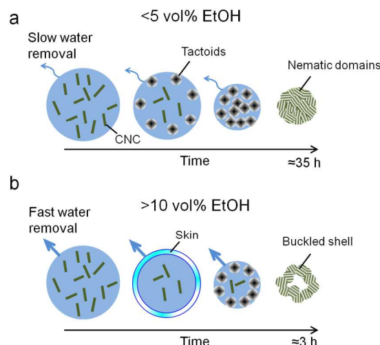
Fig. 9 Schematic description of the CNC assembly process as function of the ethanol concentration. a) Slow water dissolution rates at <5 vol% ethanol lead to a gradual CNC concentration increase until an anisotropic CNC phase (tactoids) is formed. Over time, these tactoids merge to a solid spheroid. b) High water dissolution rates at >10 vol% ethanol causes a rapid increase of the CNC concentration and a birefringent “skin” is formed at the interface. This layer undergoes tactoid transformation and subsequent formation of a shell covering a depleted and hollow droplet.
