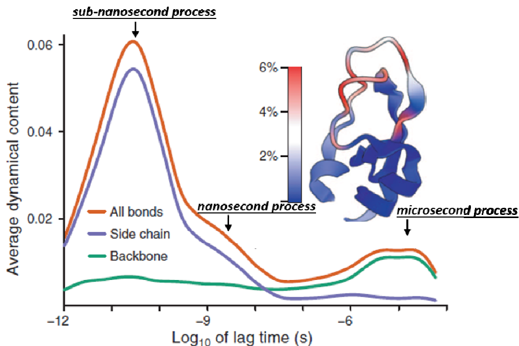
Figure 7: Dynamical content of the P_2 internal correlation function and its decomposition into side chain and backbone contribution for bovine pancreatic trypsin inhibitor (BPTI) obtained from millisecond simulations. 9 It demonstrates how dynamics of different protein parts spread over wide range of time scale. Most important, it clearly indicates existence of three relaxation modes: (i) sub-nanosecond; (ii) nanosecond and (iii) microsecond relaxations. The latter is the only one dominated by the backbone motions. Adopted with permission from ref. 9 .
