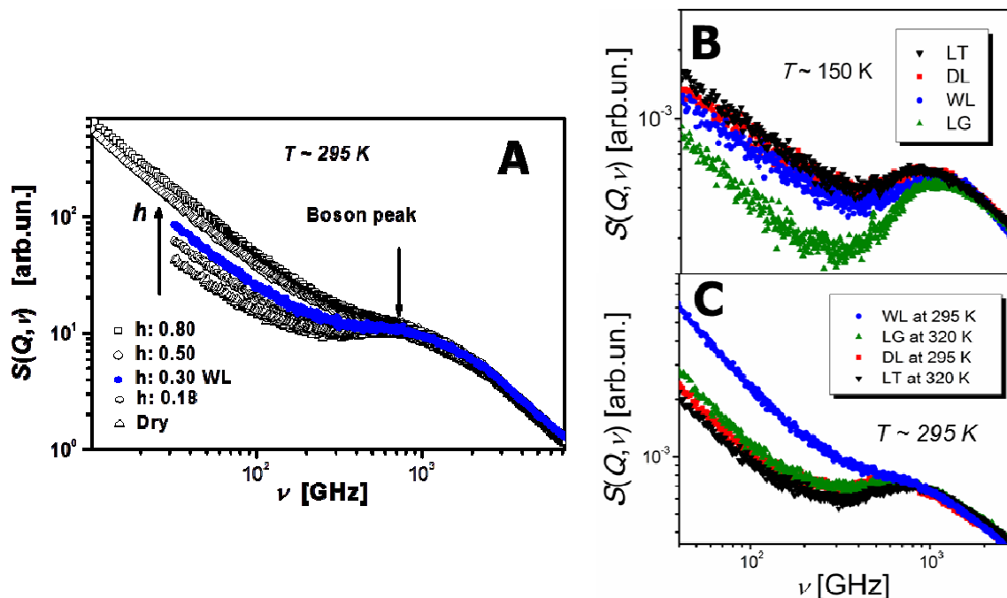
Figure 2: Dynamic structure factor S(Q, \nu) of lysozyme at (A) different hydration levels 39 ( h refers to grams of water, D_2O , per one gram of protein), and (B, C) different temperatures and solvents (DL – dry lysozyme; WL – hydrated lysozyme; LG – lysozyme in glycerol; LT – lysozyme in trehalose). 39, 90 (A): As hydration level increases the Boson peak shifts to higher frequencies and the quasielastic contribution coming mainly from the fast relaxation process strongly increases. (B) At low T=150 K the fast relaxation process is strongly suppressed in LG. While as temperature increase to ambient T \sim 295 K (C) WL has the most contribution from the fast relaxation process. This behavior of the protein's fast relaxation follows the behavior of the solvent. 79, 89
