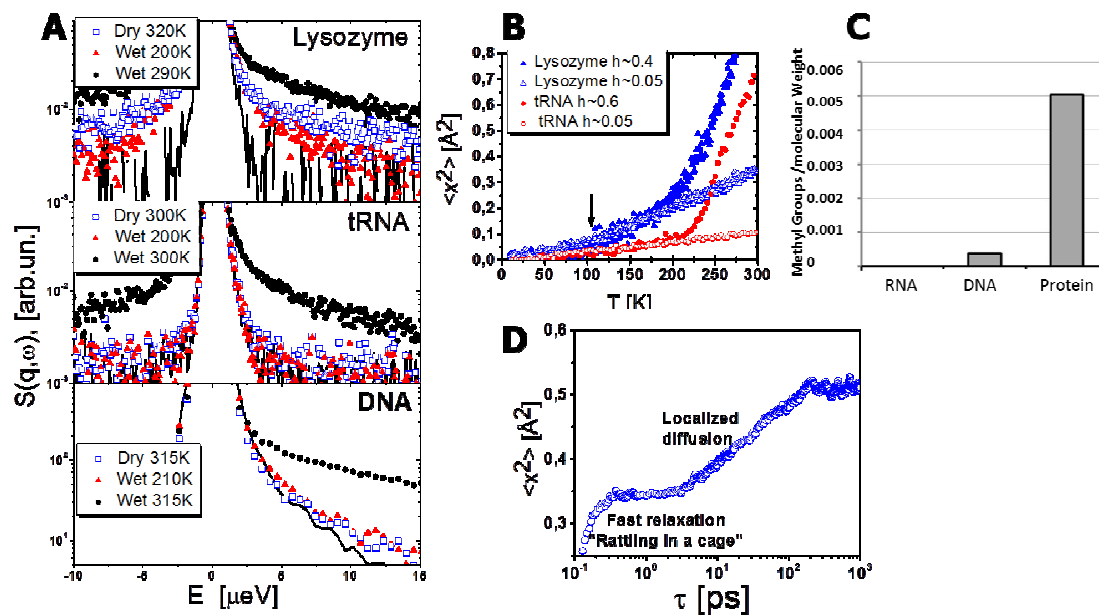
Figure 3: (A) Dynamic structure factor S(Q, E) of lysozyme, tRNA and DNA. Data for lysozyme and tRNA are from, 92 for DNA from. 99 The relaxation process appears as a quasielastic scattering, i.e. extra broadening in comparison to the resolution function of the spectrometer (line). Lysozyme spectra exhibit relaxation contribution even in the dry state and at T = 200 K, while no quasielastic scattering is observed for dry tRNA and DNA, or for hydrated tRNA and DNA below 210 K. This broadening for lysozyme is related to the methyl group rotation. (B) Mean squared displacements demonstrate onset of methyl group rotation at T \sim 100 K for lysozyme as marked by the arrow. This onset is absent in MSD of tRNA. Sharp rise of MSD in hydrated biomacromolecules at T above \sim 220 K is usually called the dynamic transition. (C) Methyl groups in different classes of biological macromolecules are presented in numbers of methyl groups per molecular weight. 94 Proteins have significant number of methyl groups in comparison to DNA (one out of four nucleic acids has a single methyl group) and RNA (no methyl in primary structure of RNA). (D) An example of MSD of hydrogen atoms in lysozyme involved in the localized diffusion motion as a function of time obtained from MD-simulations. 6 It demonstrates fast dynamics and caging (plateau) at times shorter than \sim 3 ps, followed by the localized diffusion with an almost logarithmic increase in MSD up to \sim 200 ps. MSD saturates at longer times indicating localized motion.
