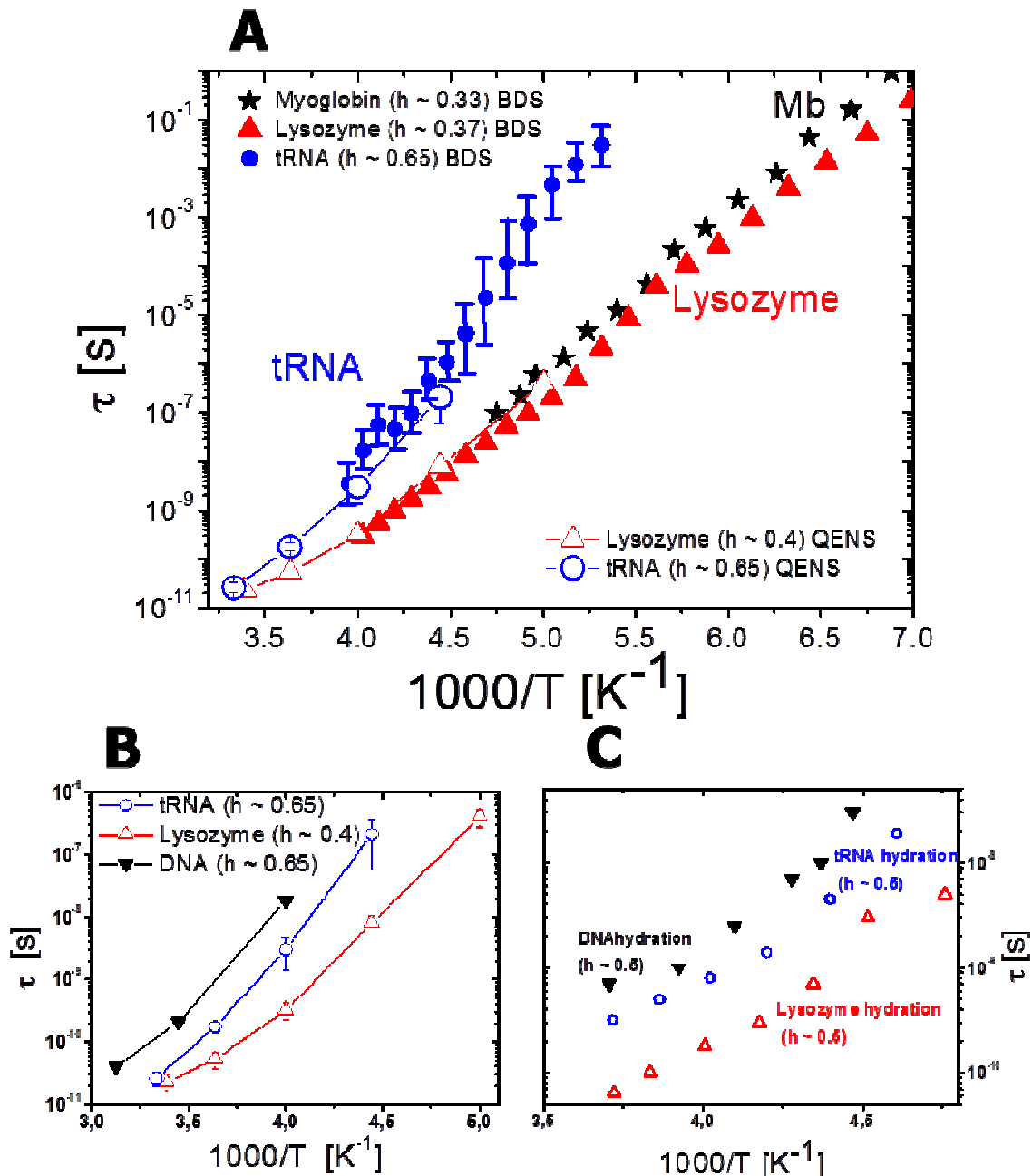
Figure 5: (A) Temperature dependence of characteristic relaxation times of hydrated lysozyme, 48, 122 Myoglobin 123 and tRNA, 122 as estimated from broadband dielectric (closed symbols) and neutron scattering (open symbols) spectroscopies. In all cases the relaxation time was estimated from the susceptibility maximum (Fig.4) or dielectric loss maximum, \tau=(2\pi\nu_{\max})^{-1} . (B) Temperature dependence of characteristic relaxation times estimated from quasielastic neutron scattering spectra of tRNA, 122 lysozyme, 48, 122 and
