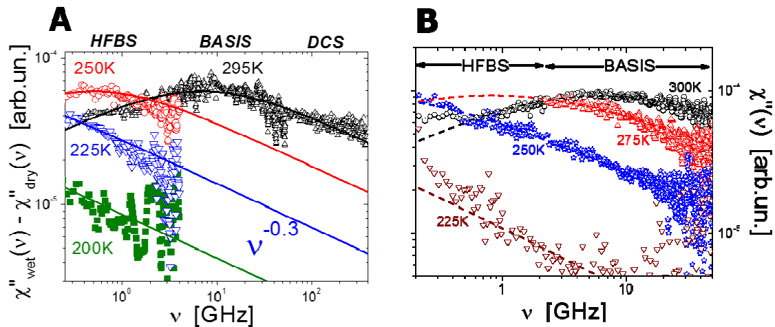
Figure 4: (A) Neutron scattering susceptibility spectra of the localized motion in hydrated lysozyme ( h \sim 0.35 ) at different temperature after correction for methyl group rotation. 106 (B) Neutron scattering susceptibility of the localized motion in hydrated t-RNA ( h \sim 0.65 ) at different temperatures. 122 Symbols are experimental data and lines are the fit to Cole-Cole distribution functions. Names at the top present different neutron scattering spectrometers used in these studies.
