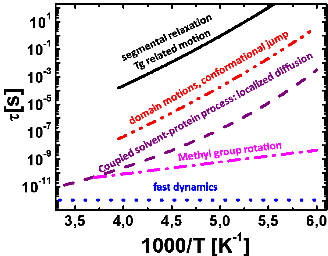
Figure 9: Schematic of temperature dependence of different internal motions of protein including: (i) Main structural (segmental) relaxation reaching \tau \sim 100 s at glass transition temperature T_g of hydrated proteins; (ii) Domain motions, conformational jumps with nanosecond relaxation times at room temperature; (iii) Coupled protein-solvent motions, presents “localized diffusion” of residues and side group motions with relaxation time of tens of picosecond at room temperature; (iv) Methyl group rotation with Arrhenius temperature dependence; and (v) Fast picosecond relaxation with a rather weak temperature dependence of the characteristic relaxation time. Processes (ii) – (iv) are apparently kinds of secondary relaxation in protein.
