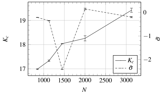
Fig. 5 Measured bending stiffness K_c together with standard error (error bars) as a function of the number of vertices N used in the triangulation of the membrane, for the input bending stiffness \kappa = 20kT . The dimensionless mean lateral tension \bar{\sigma} for the same sets of measurements is also shown. Lines connecting the points are for the guide-of-eye only.
