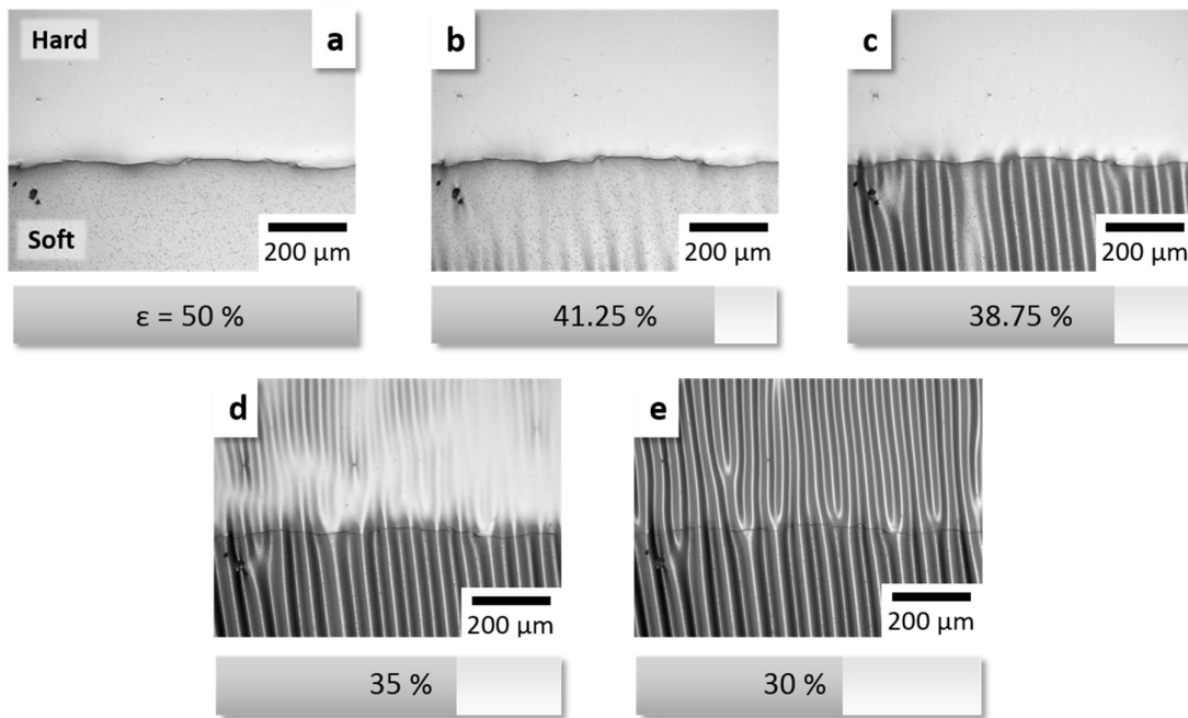
Figure 3: Same-spot in-situ observation of the release process, focused on the crossover line from hard to soft PDMS. The soft discrete inclusion is present at the bottom each, the hard at the top. In the beginning the substrate is pre-strained to 50% of its initial length (a), the oxidized layer on top is unstrained. Upon strain release wrinkles do form first within the soft inclusion (b and c) followed by the hard matrix (d and e). For a video capture of this process, see ESI.
