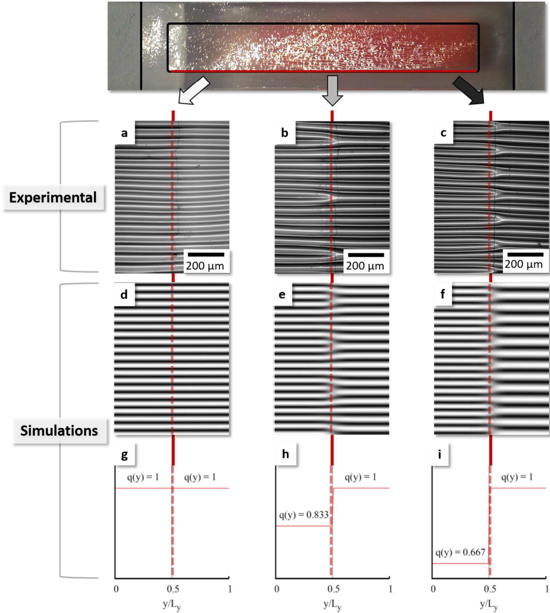
Figure 6: Branching points ordered along the gradient borderline with a jump in elasticity and wavenumber, respectively; (a – c) show experimental results, (d – f) the according simulations that are based on predetermined step-functions (g – i)
