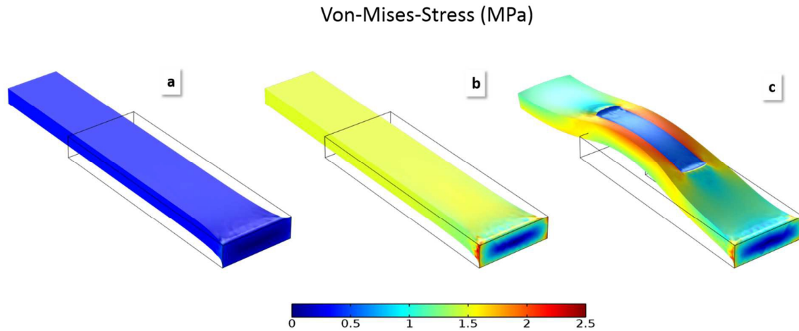
Figure 5: Mechanical simulations of neat, soft (a) respectively hard PDMS block (b) and a composite of soft block in a hard matrix (c). In all cases the initial dimensions of the outer block were set to 30 \times 10 \times 3 \text{ mm}^3 indicated by the black box, in (c) the inner block is sized 10 \times 5 \times 1.5 \text{ mm}^3 , positioned lateral in the middle of the outer block, vertical on the upper side of it. The applied strain \epsilon is set for all simulations to 50 %. Von-Mises-stress distribution was modeled using COMSOL multiphysics with the same parameters as before except \nu_s , which was set to 0.499.
