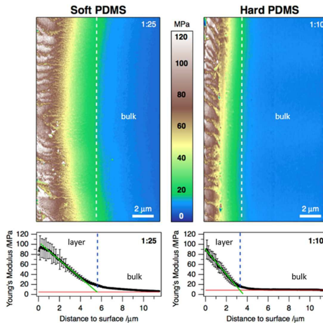
Figure 4: Peak force analysis: The terrain images are nanomechanical mappings of the Young's modulus at the bulk/oxide layer interphase of soft (left) and hard PDMS (right). Below are the according cross section profiles that were averaged over the whole image size consisting of 469 lines.
