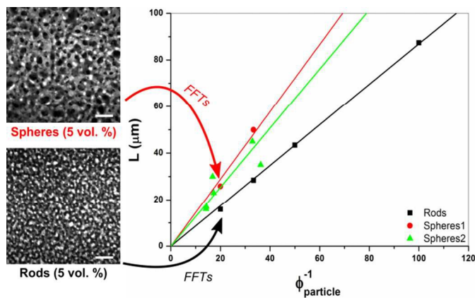
Fig. 2 Low magnification confocal microscopy images of bijels stabilized by 5vol.% (a) spheres and (b) rods, respectively. Observed fluorescence is from (a) Nile Red in the NM-rich phase, and (b) Fluorescein in the EG-rich phase. The graph shows the domain sizes plotted as a function of \phi_{particle}^{-1} , fitted with a straight line through the origin. The scale bar is 100 micron. Note: spheres 1 and 2 are two batches of Stöber silica particles with less than 10% size difference.
