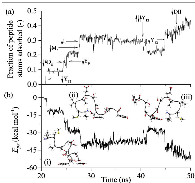
Fig 4. Trajectory of the exemplar MD simulation of GrBP5 adsorption during initiation of the lockdown phase and ongoing lockdown in a step-wise fashion: (a) fraction of peptide atoms in direct contact with the solid surface; (b) total interaction energy between peptide and solid surface, E_{PS} . In (a), direct contact ( \downarrow ) and break away ( \uparrow ) of groups from the surface are shown. Snapshots of four adsorbed states are shown in (b) at: (i) 26 ns, (ii) 35 ns, (iii) 43 ns (the surface underneath and the water have been omitted for simplicity).
