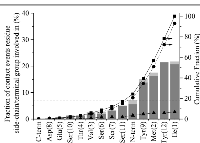
Fig 9. Contact statistics for GrBP5 at the water/graphite interface. Percentage of the total number contact events contributed by each residue or terminal group, alone (dark grey) and in combination with other residues (light grey). The dashed horizontal line at 7.1% corresponds to the fraction of events each residue/terminal group would contribute if they were proportionally distributed along the length of the peptide. Cumulative fraction of (■) total anchoring events, (●) events contributed by a single residue and (▲) combined events where two or more residues instigate anchoring.
